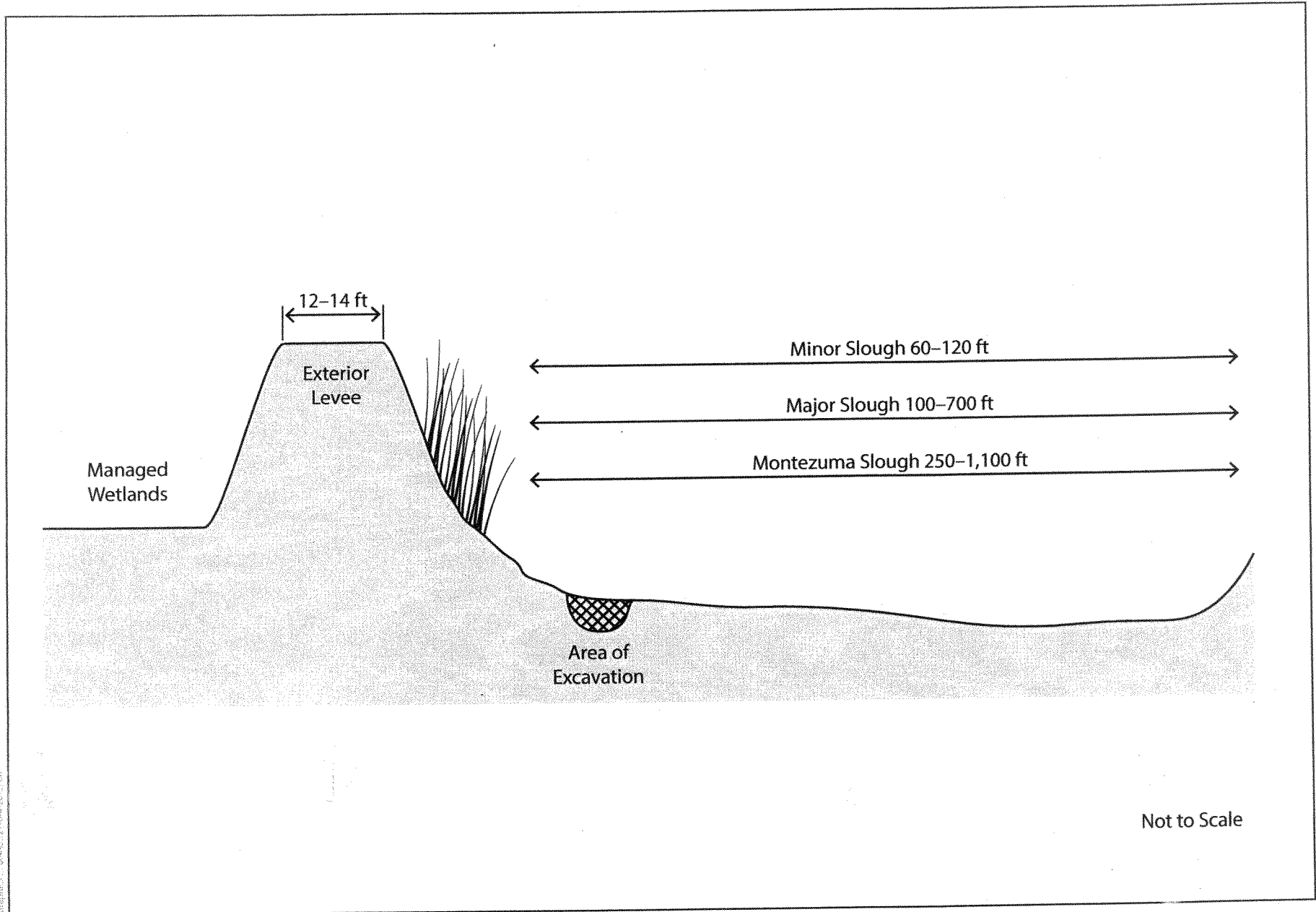
Figure 3a Suisun Marsh Dredging Program Typical Cross Section
