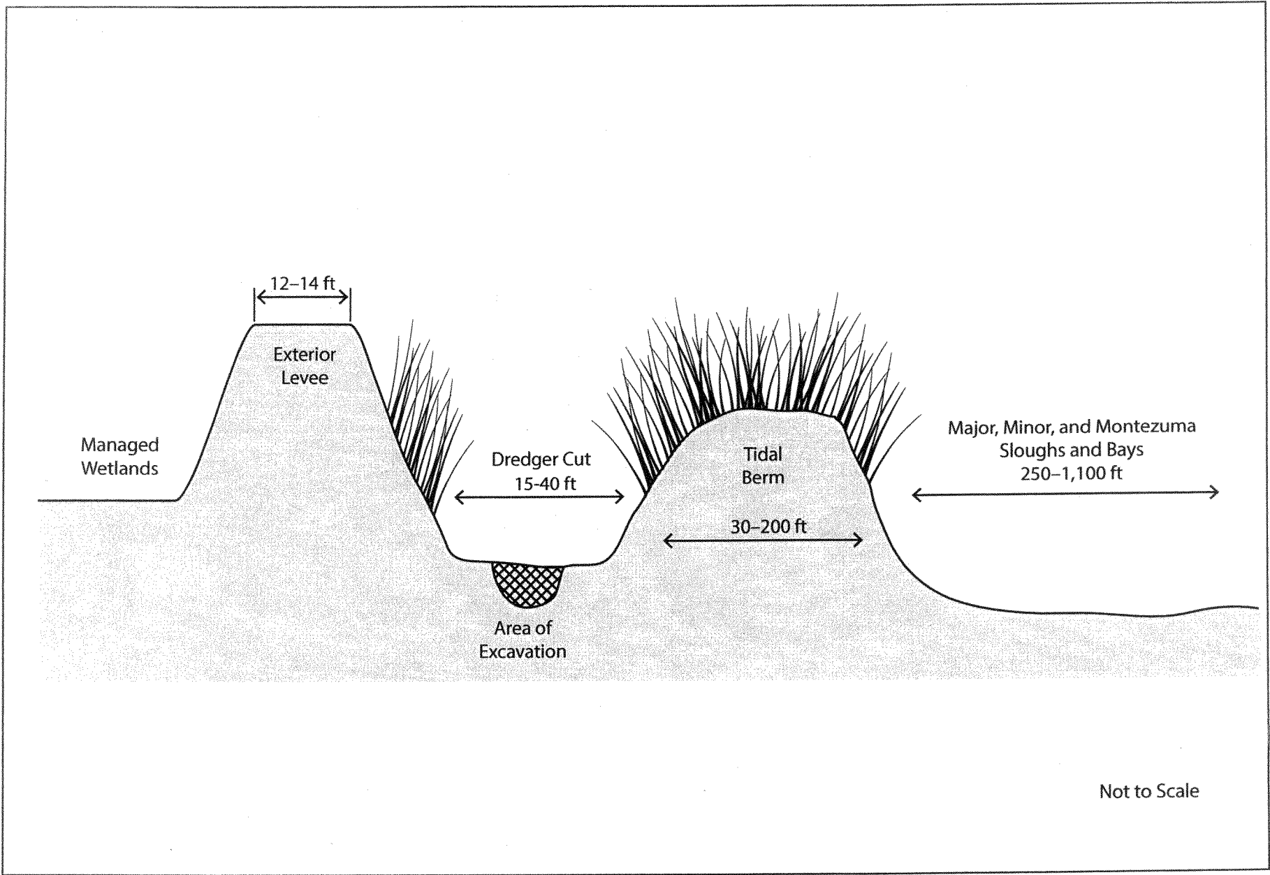
Figure 3b Suisun Marsh Dredging Program Typical Cross Section
