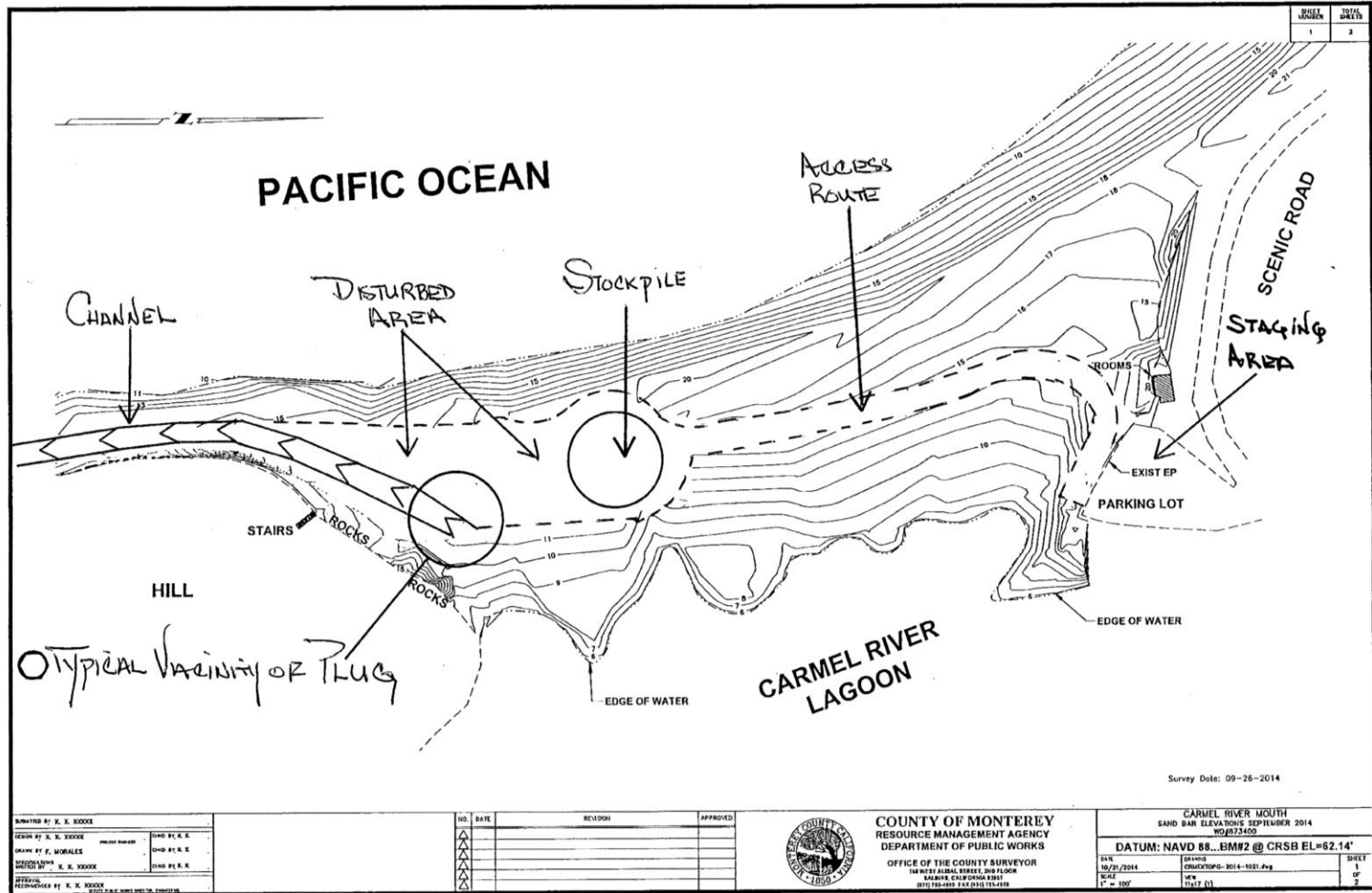
Figure 2. Carmel Lagoon Interim Management Plan Project site plan.
