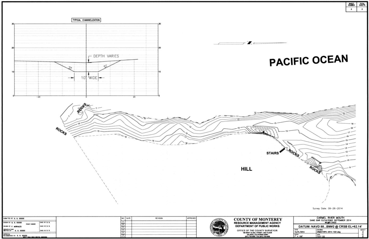
Figure 4. Carmel Lagoon Interim Management Plan Project, survey elevations, sheet 2 of 2.
