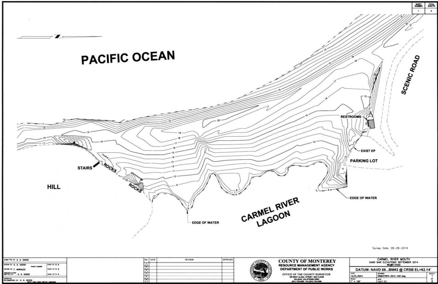
Figure 3. Carmel Lagoon Interim Management Plan Project, survey elevations, sheet 1 of 2.
