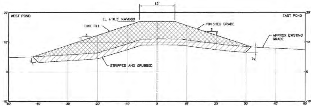
TYPICAL CROSS DIKE SECTION
