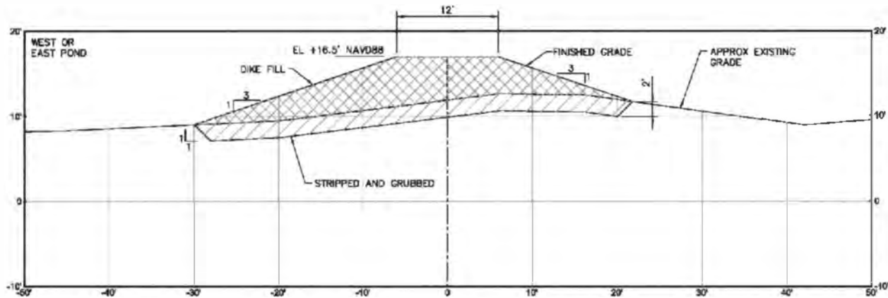
TYPICAL PERIMETER DIKE SECTION
