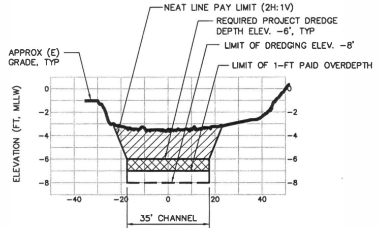
DREDGE UNIT 5 (MARINA VILLAGE CHANNEL) STA 46+50
