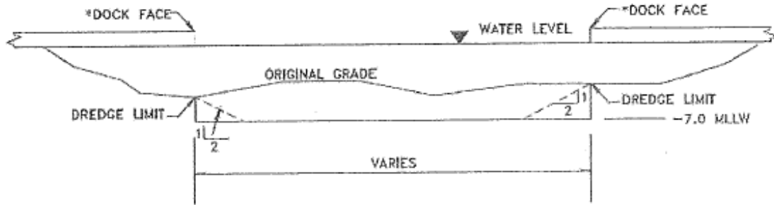
TYPICAL SECTION INSIDE WATERWAYS/CHANNELS A, B, C, D, E, NORTH & SOUTH CHANNEL AREAS
