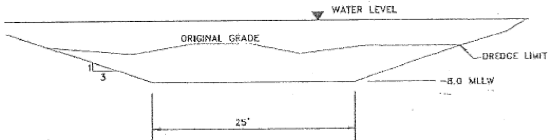
TYPICAL SECTION ENTRANCE CHANNELS
