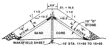
STA. 11+50 TO 17+00 BASED ON BODEGA BAY JETTY SPECS. CHANGE ORDER NO. 2, 7 MAR. '42
