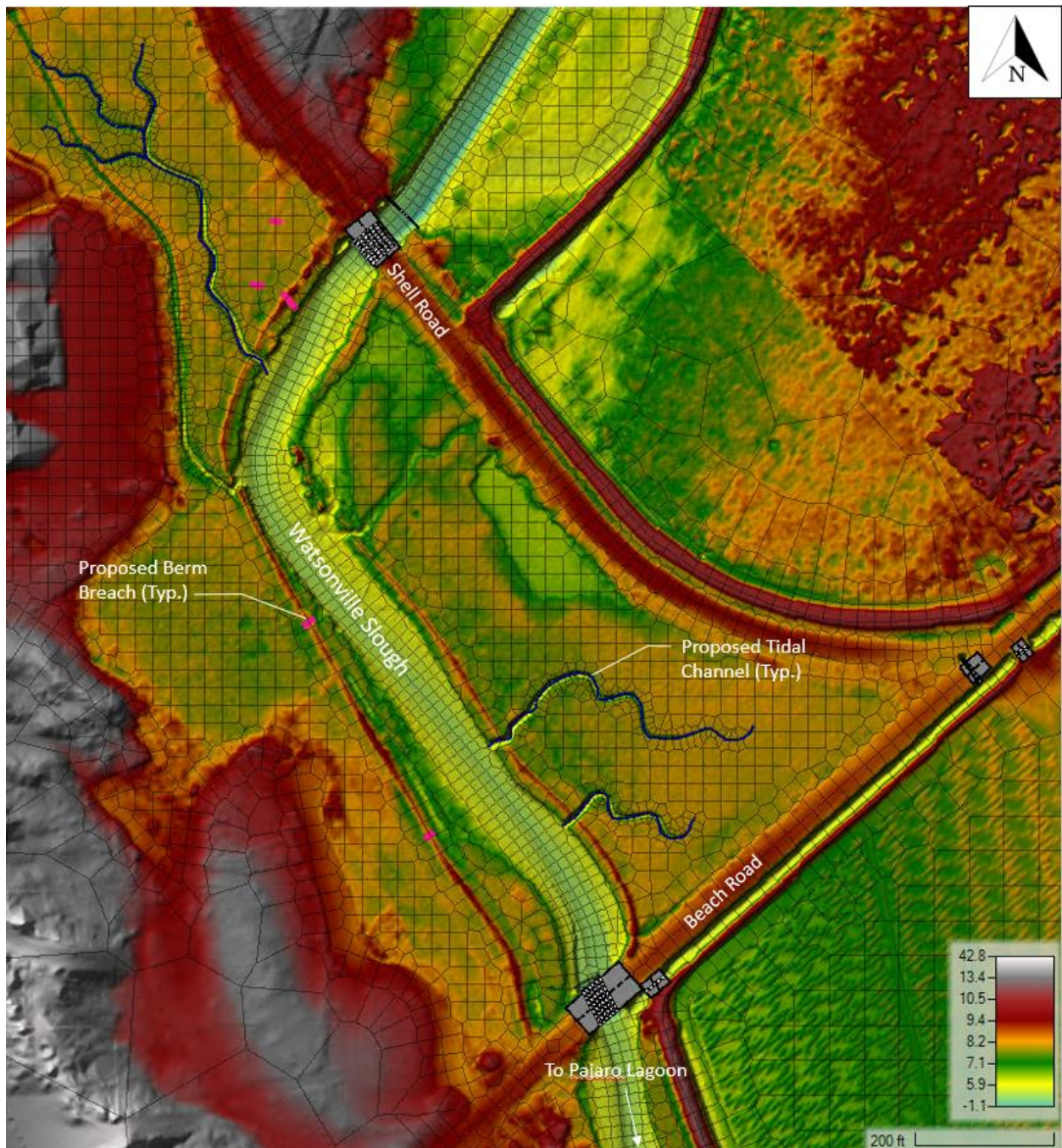
Figure 9: Earthwork project scenario.
