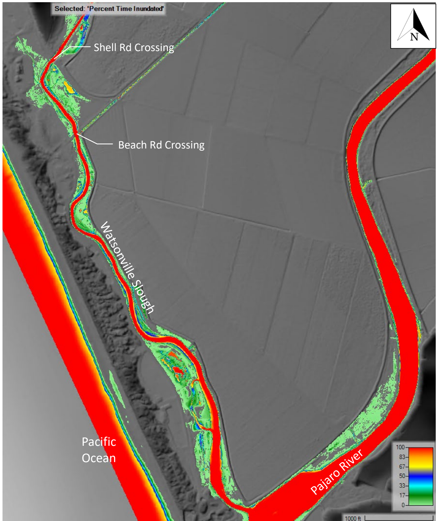
Figure 5: Percent time inundated – No Action; Year 25; Open Lagoon, Wet Season
