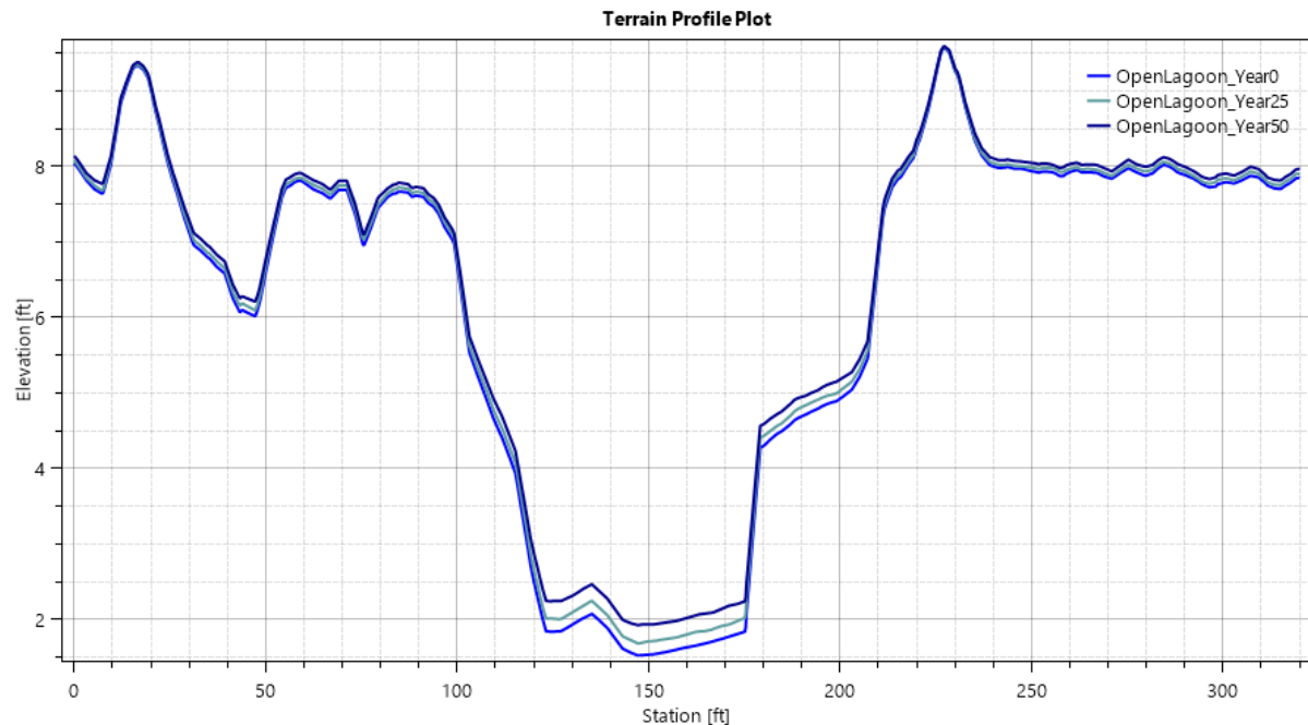
Figure 24: Cross section of HEC-RAS terrains for Project Year 0, Year 25, and Year 50 immediately upstream of the Beach Road crossing, demonstrating how marsh accretion was applied in the model.
