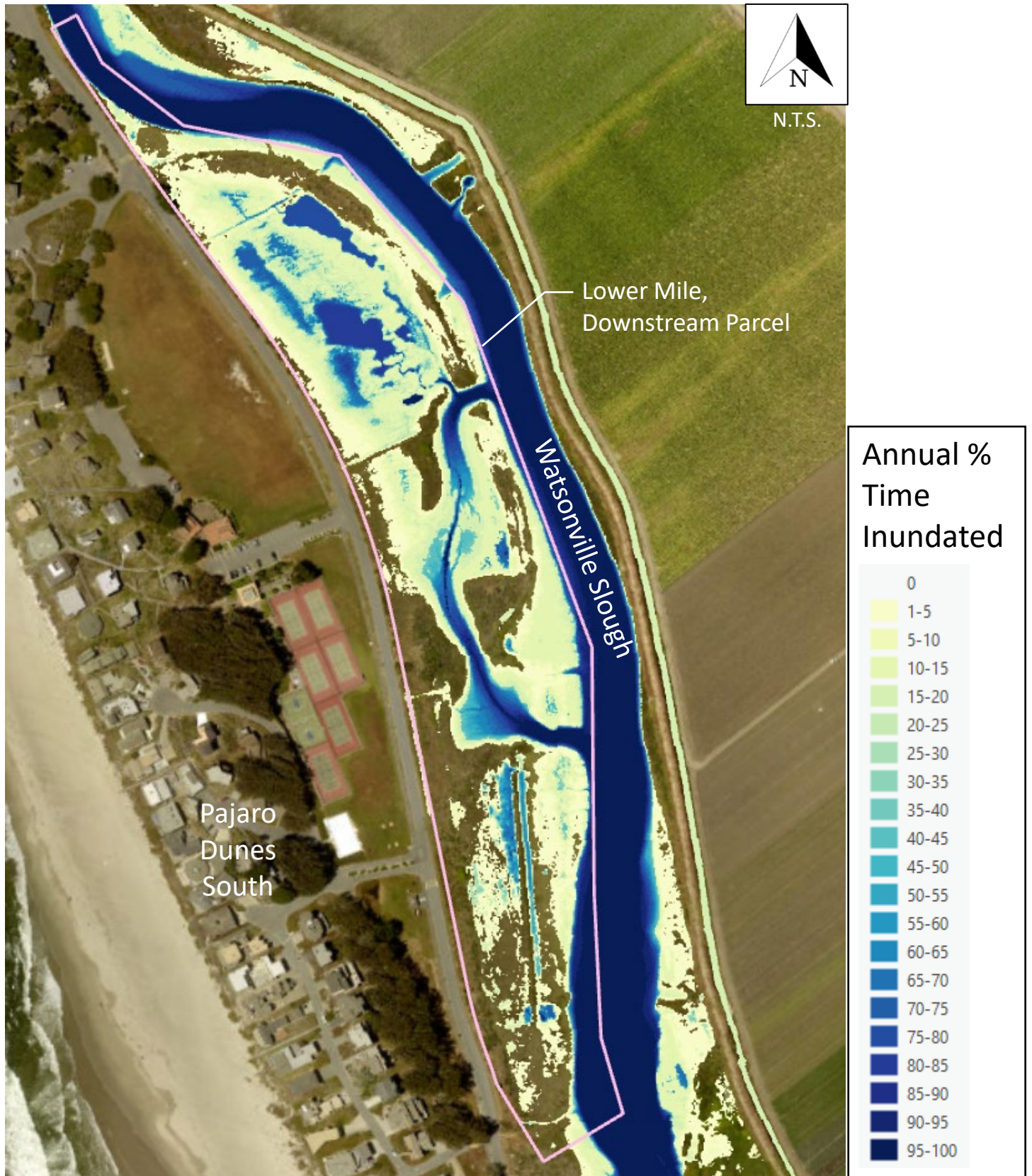
Figure 33: Annual PTI – Lower Mile, Downstream Parcel; Year 50; No Action
