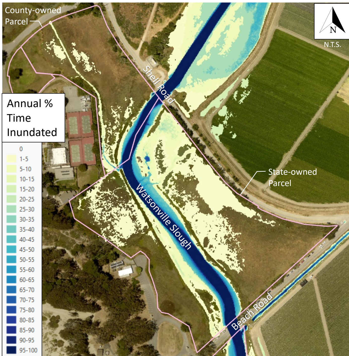
Figure 1: Annual PTI – State and County Parcels; Year 0; No Action
