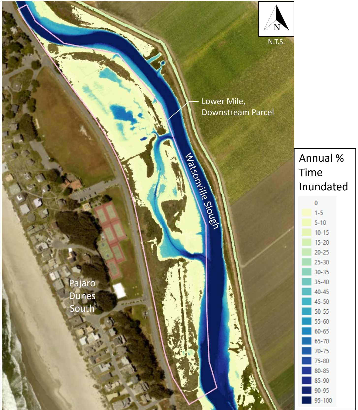
Figure 27: Annual PTI – Lower Mile, Downstream Parcel; Year 0; Earthwork
