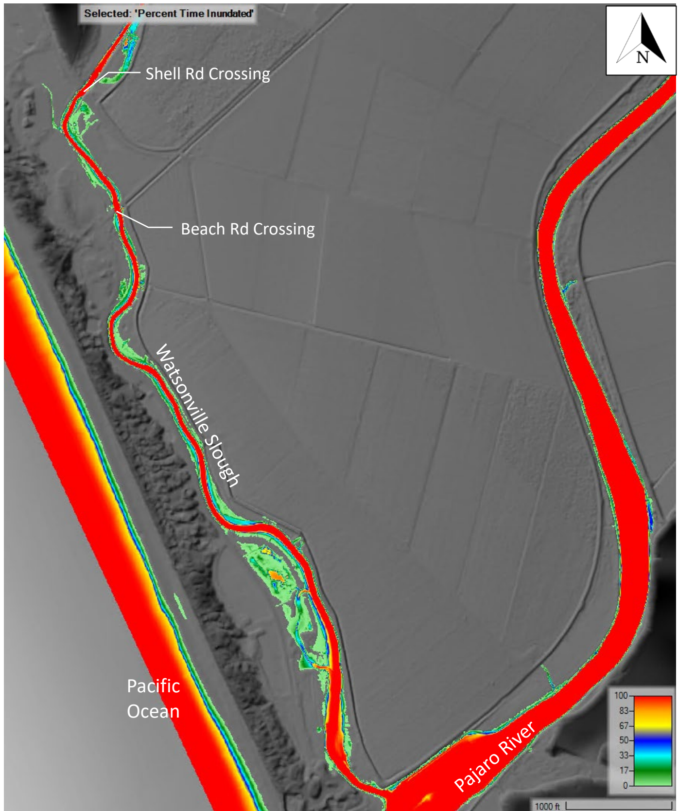
Figure 11: Percent time inundated – Crossing Improvements; Year 0; Open Lagoon, Wet Season
