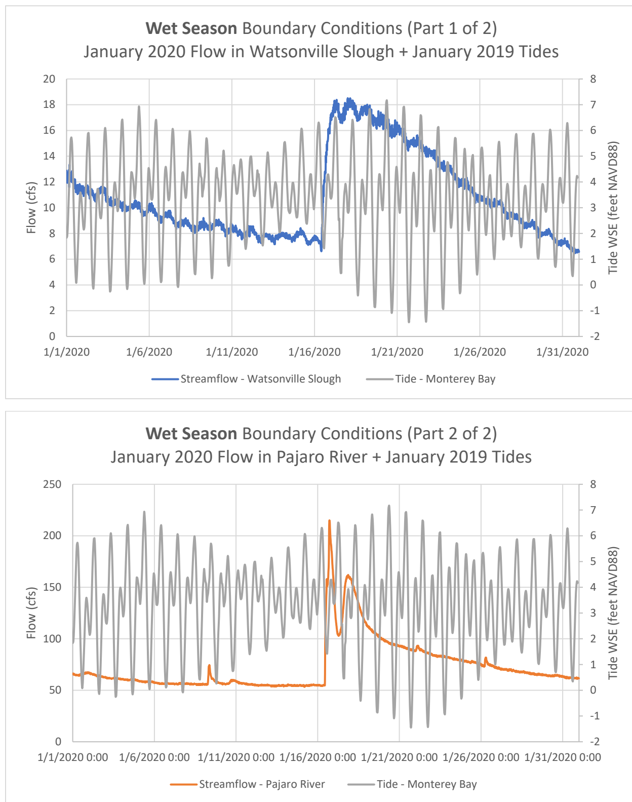
Figure 20: Open lagoon, wet season boundary conditions.
