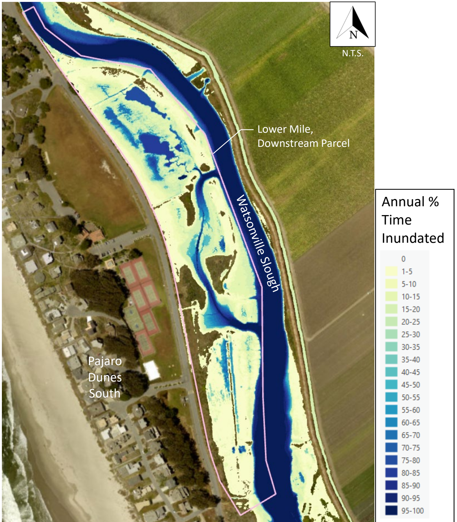
Figure 36: Annual PTI – Lower Mile, Downstream Parcel; Year 50; Crossing Improvements + Earthwork
