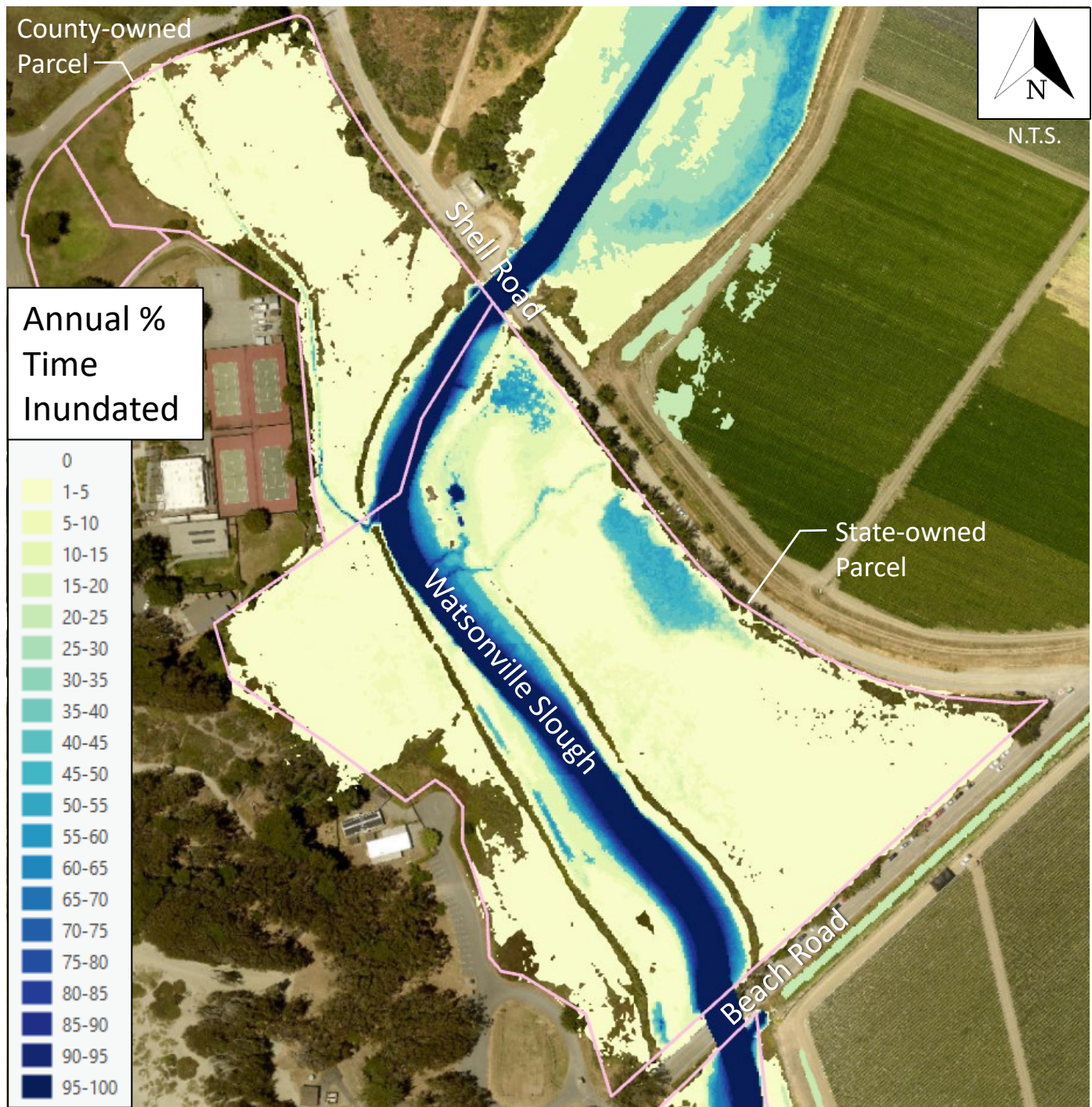
Figure 6: Annual PTI – State and County Parcels; Year 25; Crossing Improvements
