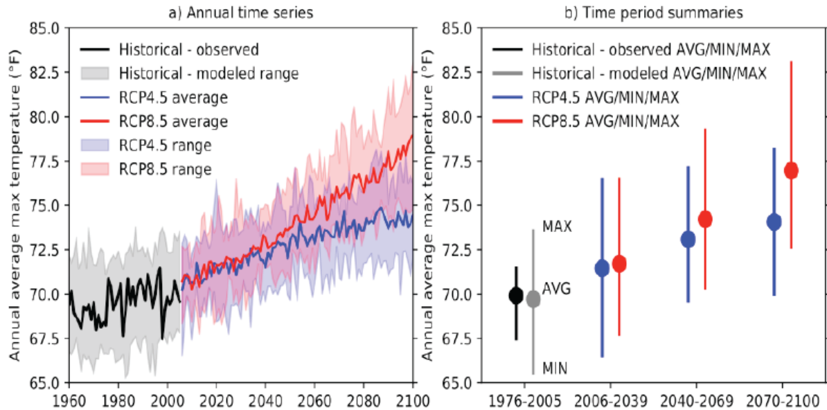
Figure 32: Annual average maximum temperature, historic and projected, for the Central Coast Region of California (Langridge 2018).
