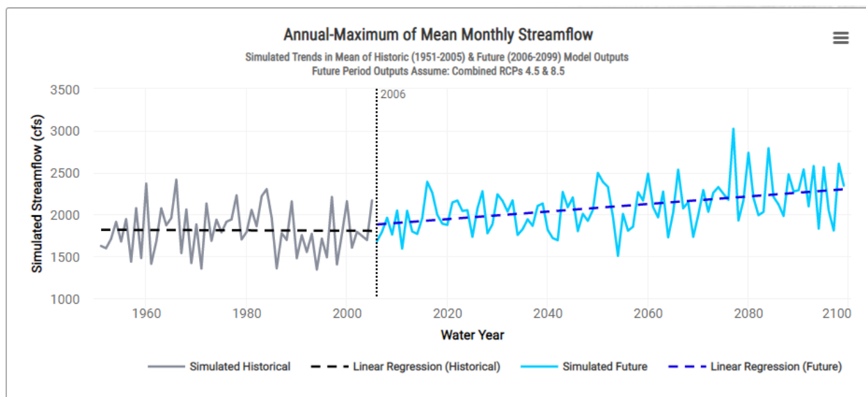
Figure 44. Trend in Annual Maximum of Average Monthly Streamflow. A statistically significant trend was detected for projected streamflow. A statistically significant trend was not detected for simulated historical streamflow.
