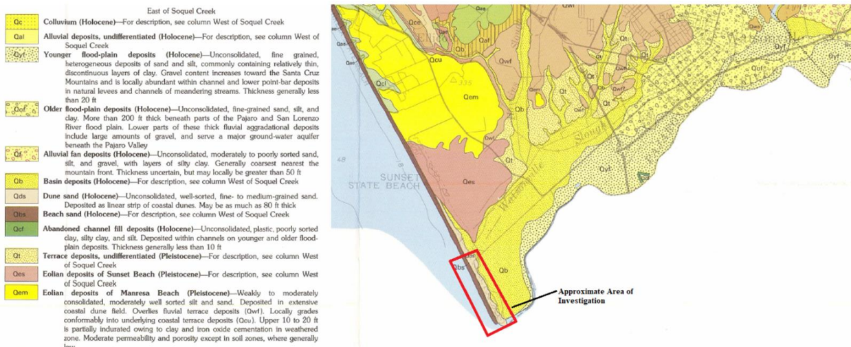
Figure 2. Geologic map of Santa Cruz County (Brabb, 1989)
