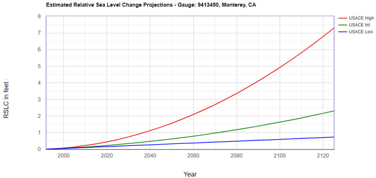
Figure 51: Relative sea level change projections from 1992 to 2125, Monterey, CA, NOAA Station #9413450.
