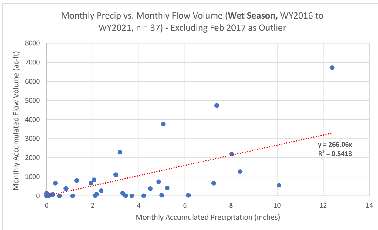
Figure 10: Scatterplot and linear regression for Wet Season.
