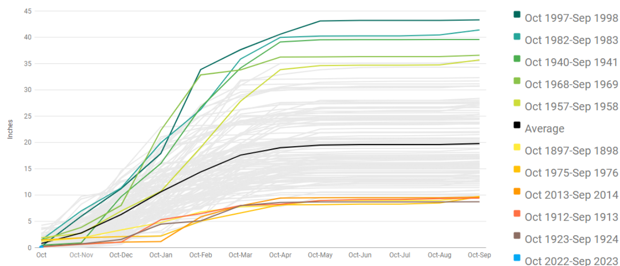
Figure 29: Cumulative precipitation totals by water year for the County of Santa Cruz (top) and Monterey (bottom) for the recent historical record (1895-present). The five highest (green), lowest (orange), and current year-to-date (blue) water year totals are highlighted. While Watsonville Slough is within Santa Cruz County, it is very near the border with Monterey County. Haywood plots downloaded December 6, 2022 from https://www.ncdc.noaa.gov/cag/county/haywood/CA-087/pcp/9 and https://www.ncdc.noaa.gov/cag/county/haywood/CA-053/pcp/9 .
