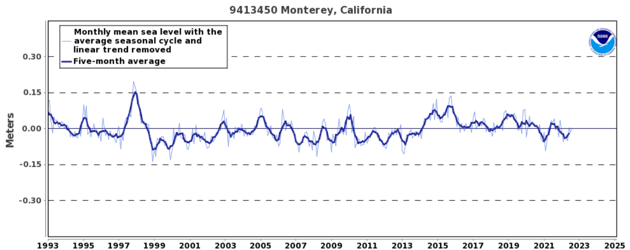
Figure 18: Interannual variability of mean sea level at Monterey tide gage. Figure obtained from NOAA Tides & Currents ( https://tidesandcurrents.noaa.gov/sltrends/sltrends_station.shtml?id=9413450 ).
