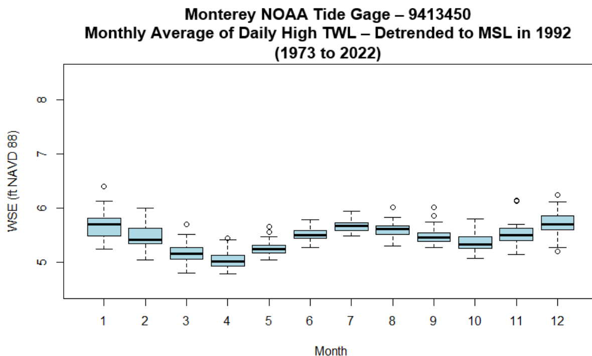
Figure 16: Distribution of Monthly Average Daily High TWL (detrended to MSL in 1992) from 1973 to present at Monterey tide gage.
