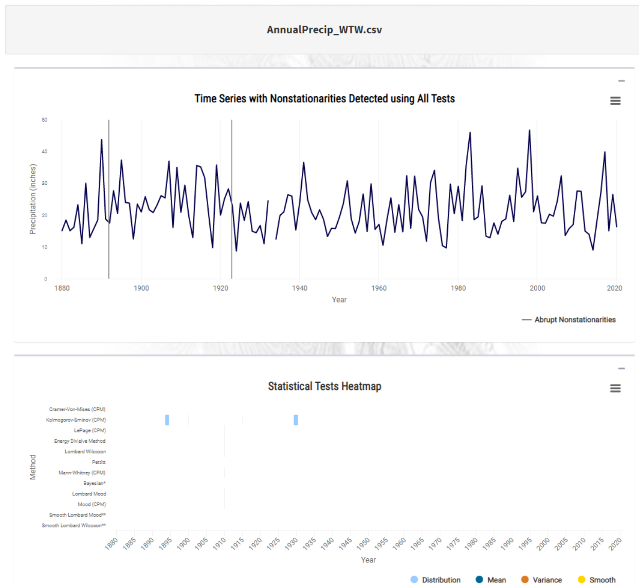
Figure 42: Nonstationarity detection results for annual precipitation at Watsonville Waterworks (WTW). Two nonstationarities were detected in 1890 and 1923 (in distribution). No consensus or robustness were detected for these nonstationarities.
