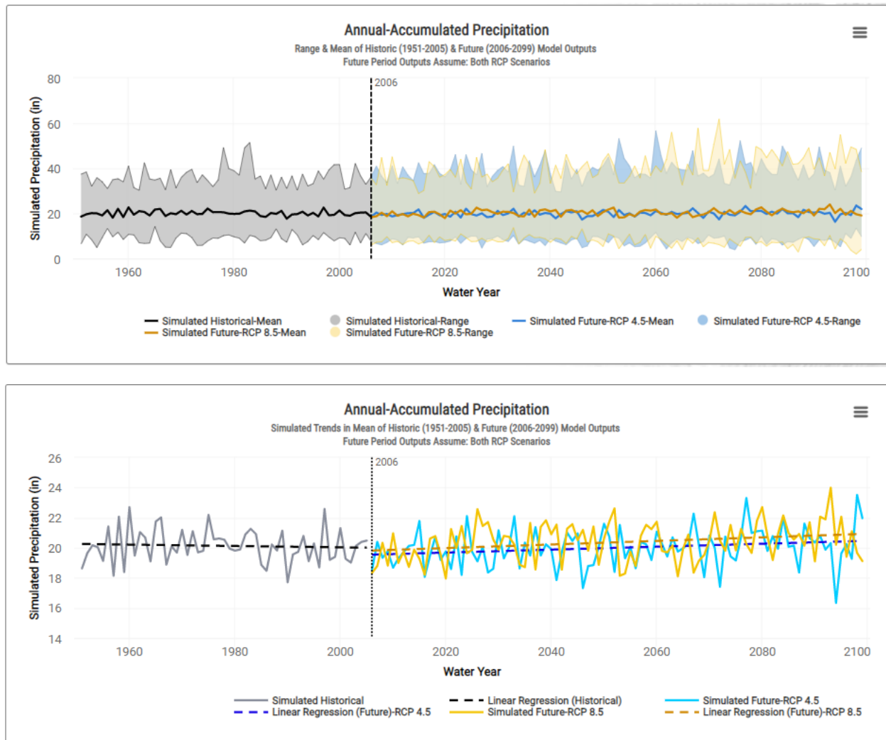
Figure 39. Annual Sum of Daily Accumulated Precipitation. Range and mean (top) and trends (bottom) for RCP4.5 and RCP8.5. Statistically significant trends were detected for projected future precipitation under both scenarios. Statistically significant trend was not detected for simulated historical precipitation.
