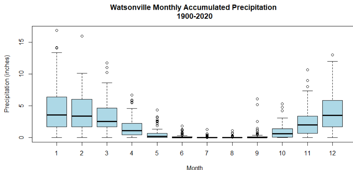
Figure 41: Box and whisker plot of monthly precipitation at Watsonville Waterworks (WTW) rain gage.
