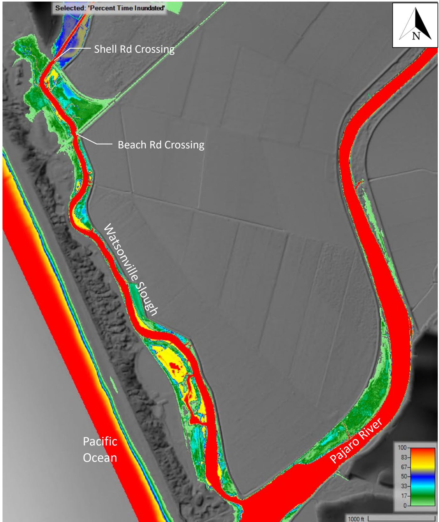
Figure 33: Percent time inundated – Crossing Improvements + Earthwork; Year 25; Closed Lagoon, Wet Season
