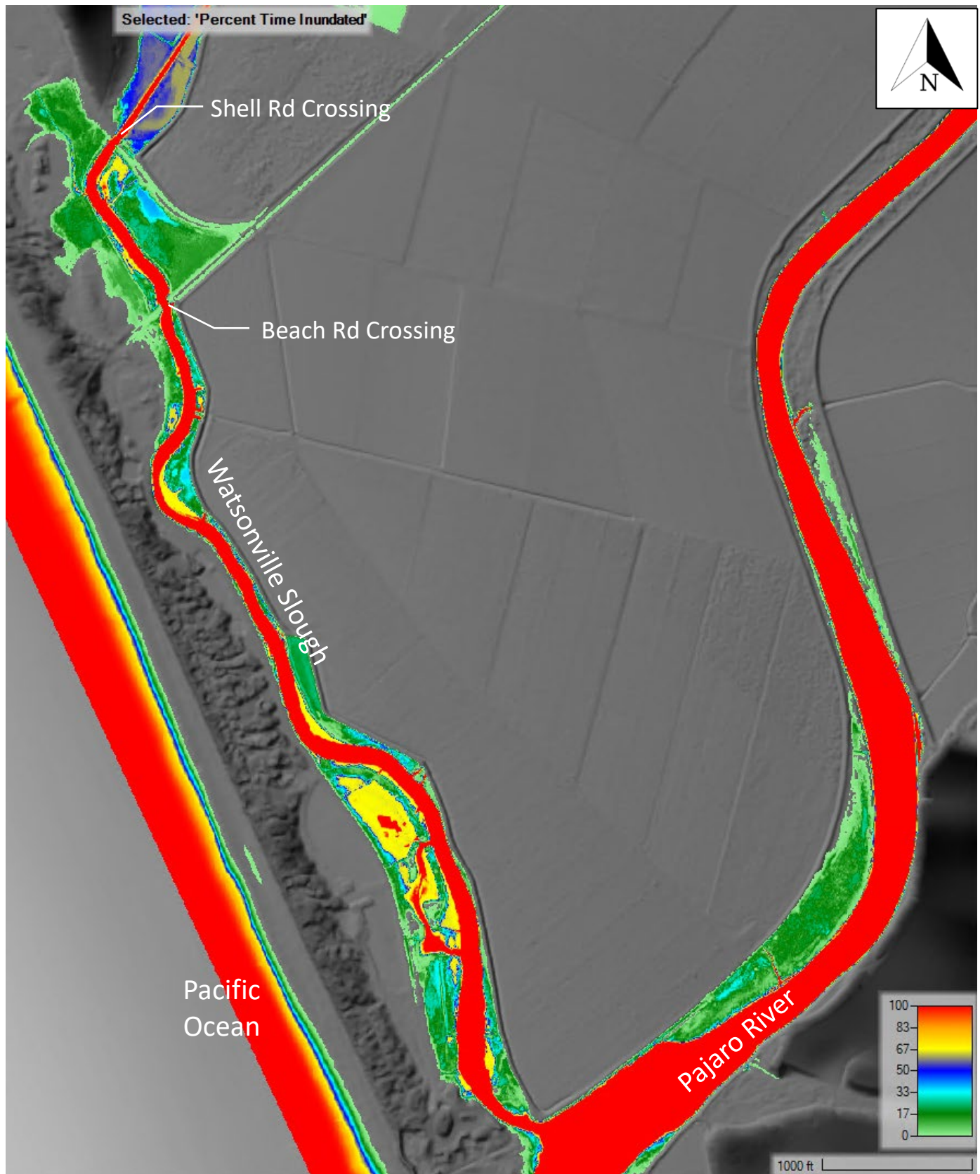
Figure 18: Percent time inundated – Crossing Improvements; Year 50; Closed Lagoon, Wet Season
