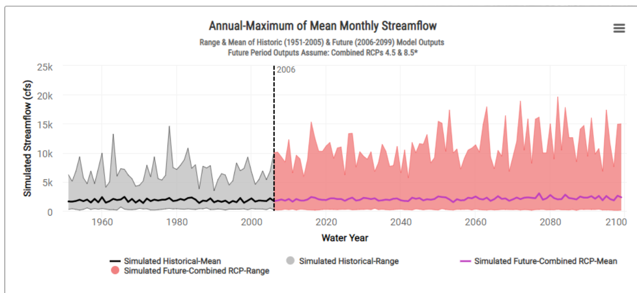
Figure 43. Range and mean of Annual Maximum of Average Monthly Streamflow for HUC 18060002. Spatially-downscaled, hydrologically-simulated and routed, and statistically-aggregated CMIP5 GCM output for the stream segment with the largest flow in the HUC 8 region. Streamflow is representative of cumulative flow from all upstream segments as well as the local runoff contributions to the aligned stream segment. Simulated flows are unregulated.
