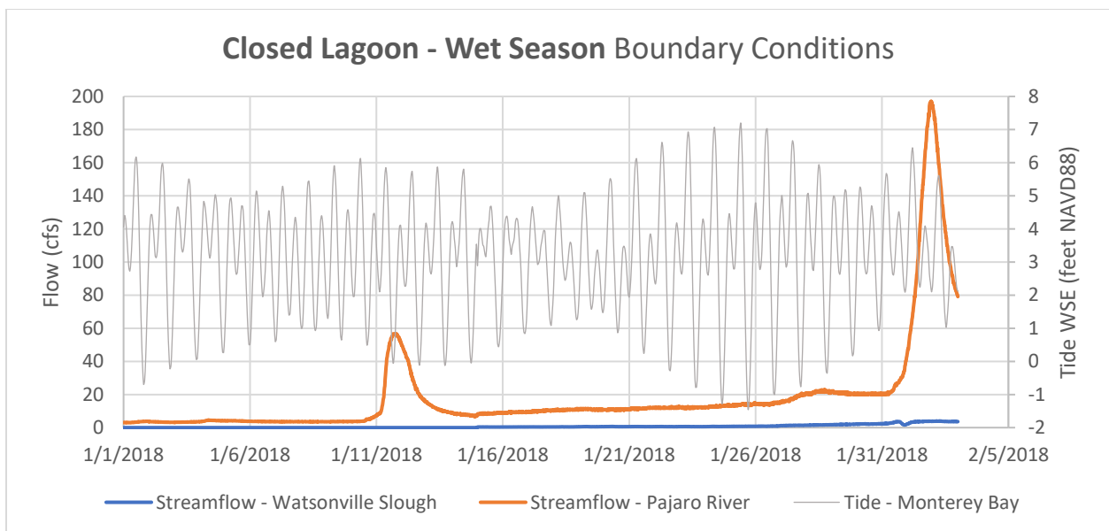
Figure 6: Hydrologic boundary conditions selected as representative of the Closed Lagoon, Wet Season hydrologic regime.
