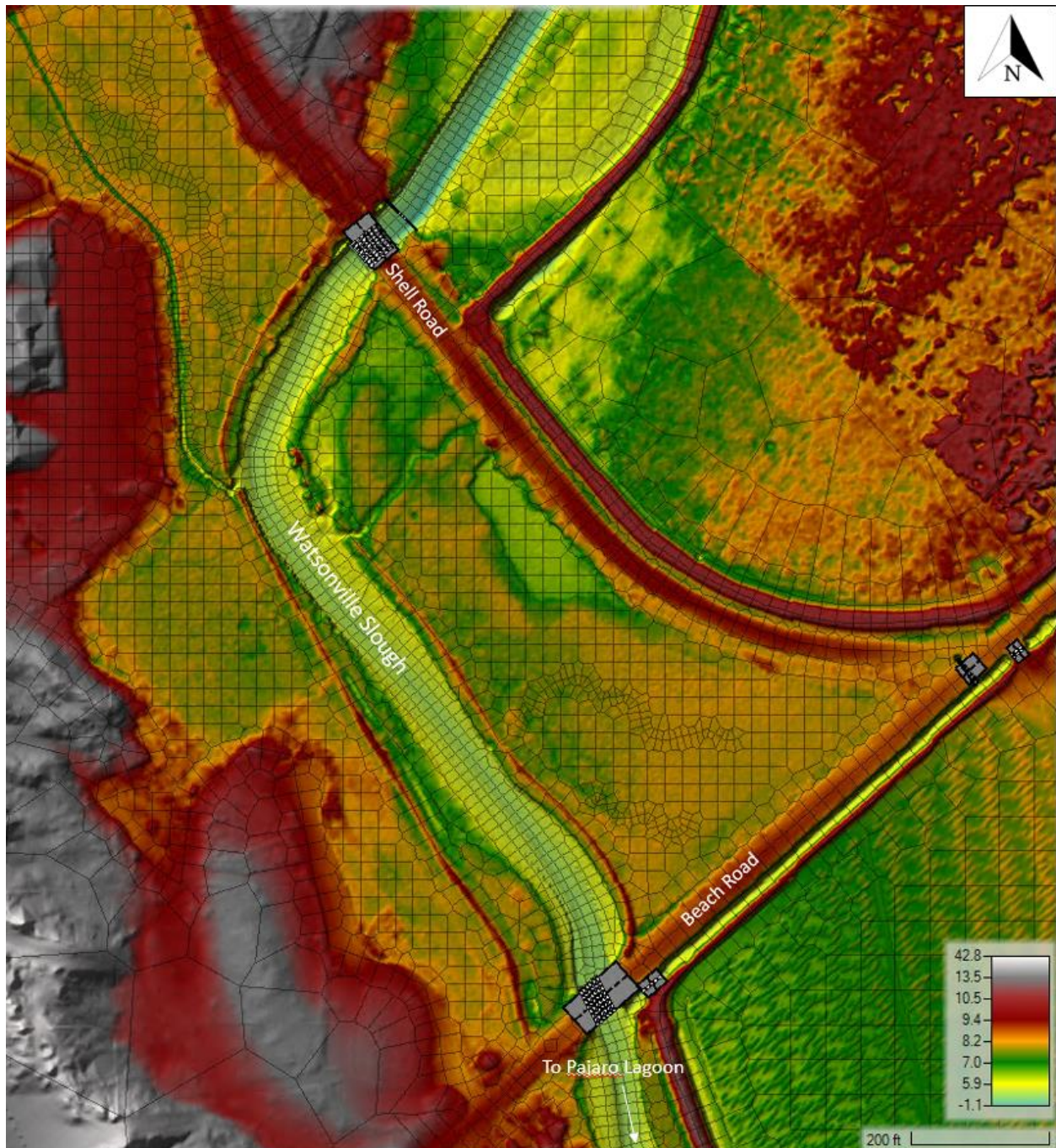
Figure 7: No Action project alternative.
