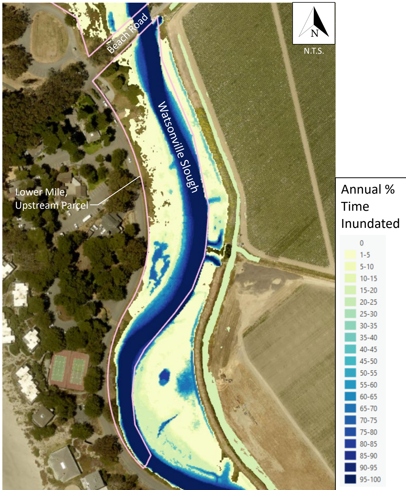
Figure 22: Annual PTI – Lower Mile, Upstream Parcel; Year 50; Crossing Improvements
