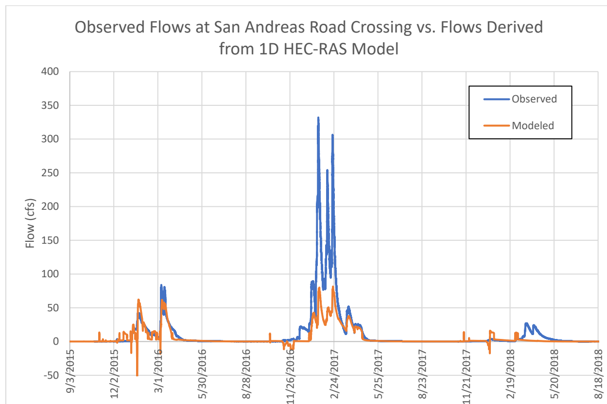
Figure 6: Period of overlap in the modeled and observed streamflow records in Watsonville Slough.
