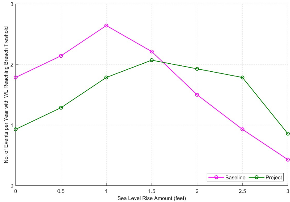
Figure 11 Predicted change in number of events per year with water level reaching breach threshold, with and without Project.
