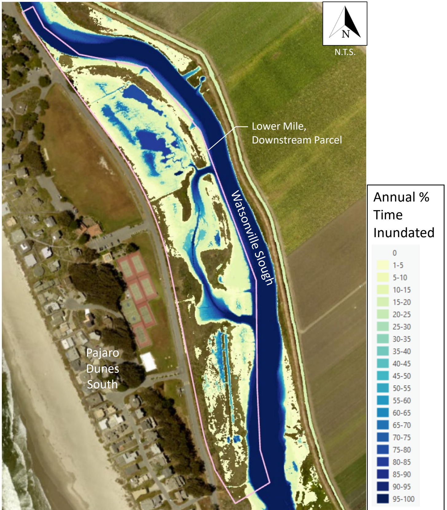
Figure 35: Annual PTI – Lower Mile, Downstream Parcel; Year 50; Earthwork
