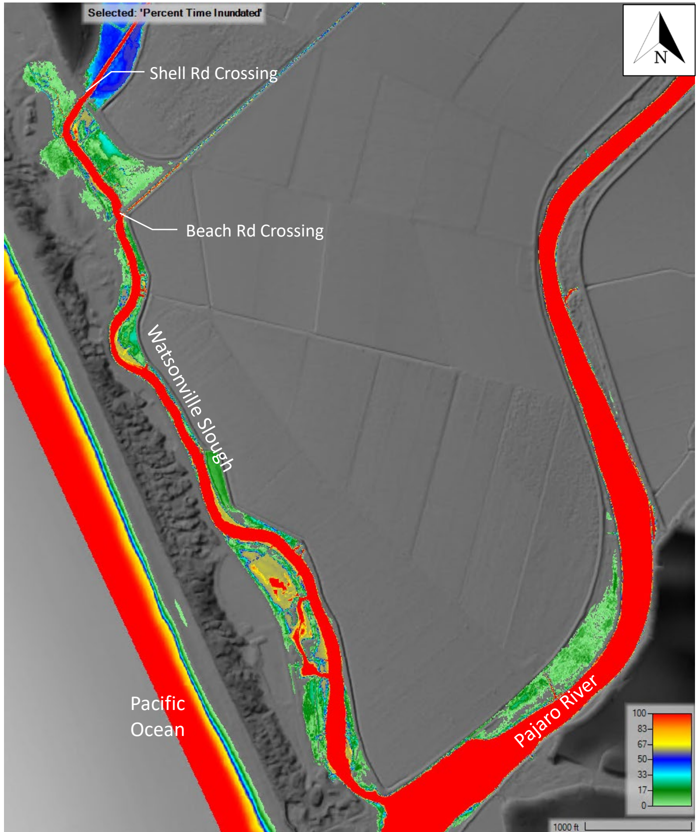
Figure 24: Percent time inundated – Earthwork; Year 25; Closed Lagoon, Wet Season
