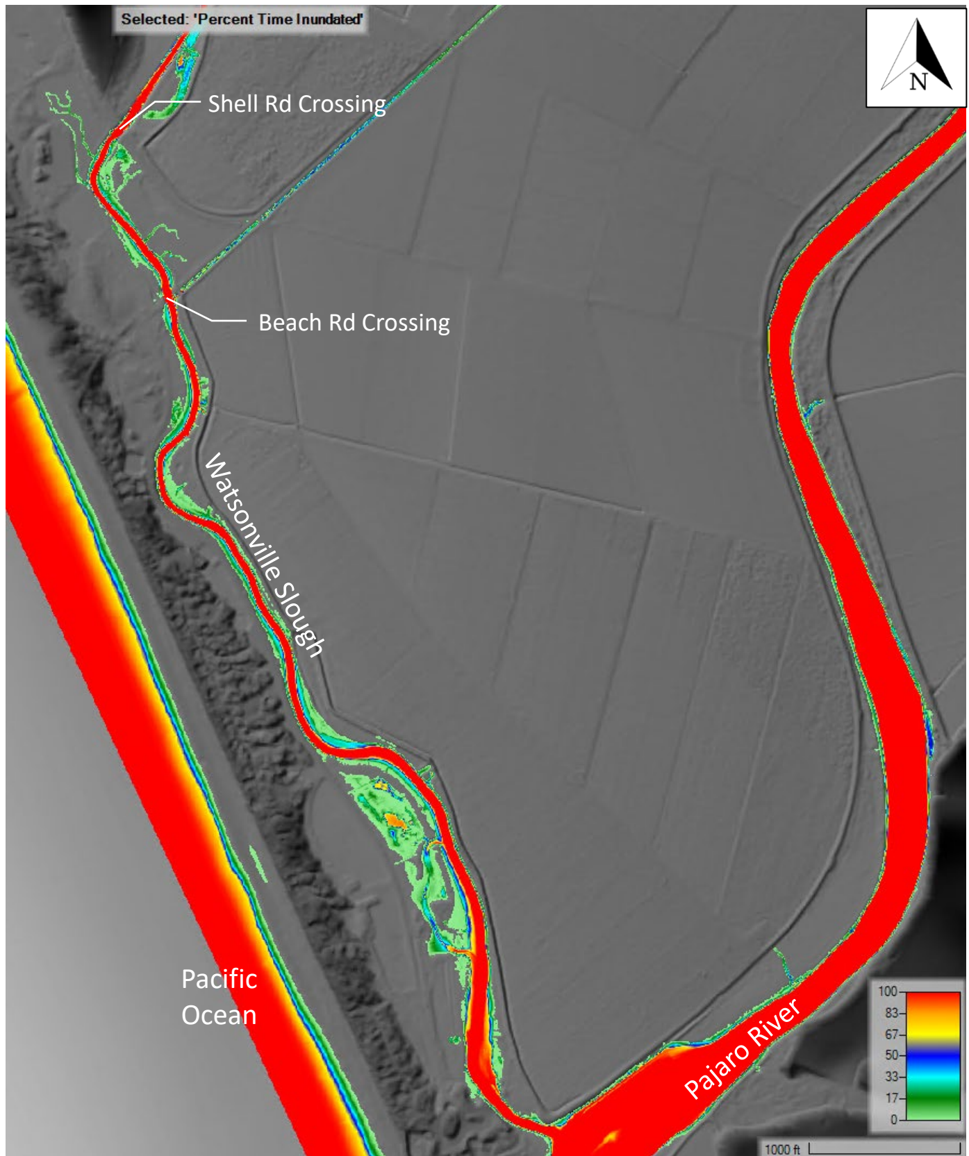
Figure 20: Percent time inundated – Earthwork; Year 0; Open Lagoon, Wet Season
