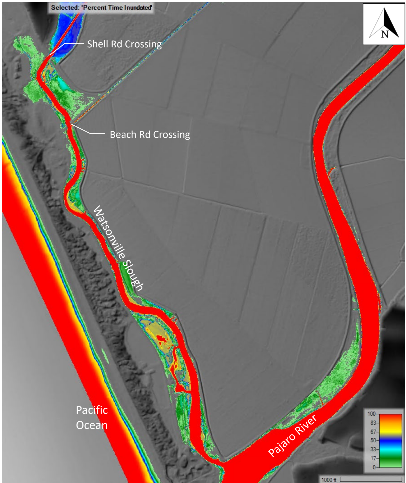
Figure 6: Percent time inundated – No Action; Year 25; Closed Lagoon, Wet Season
