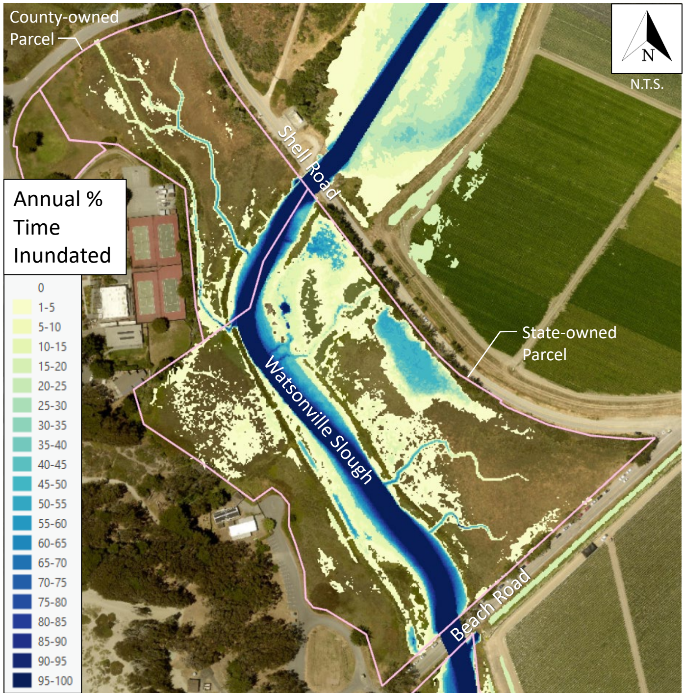
Figure 7: Annual PTI – State and County Parcels; Year 25; Earthwork
