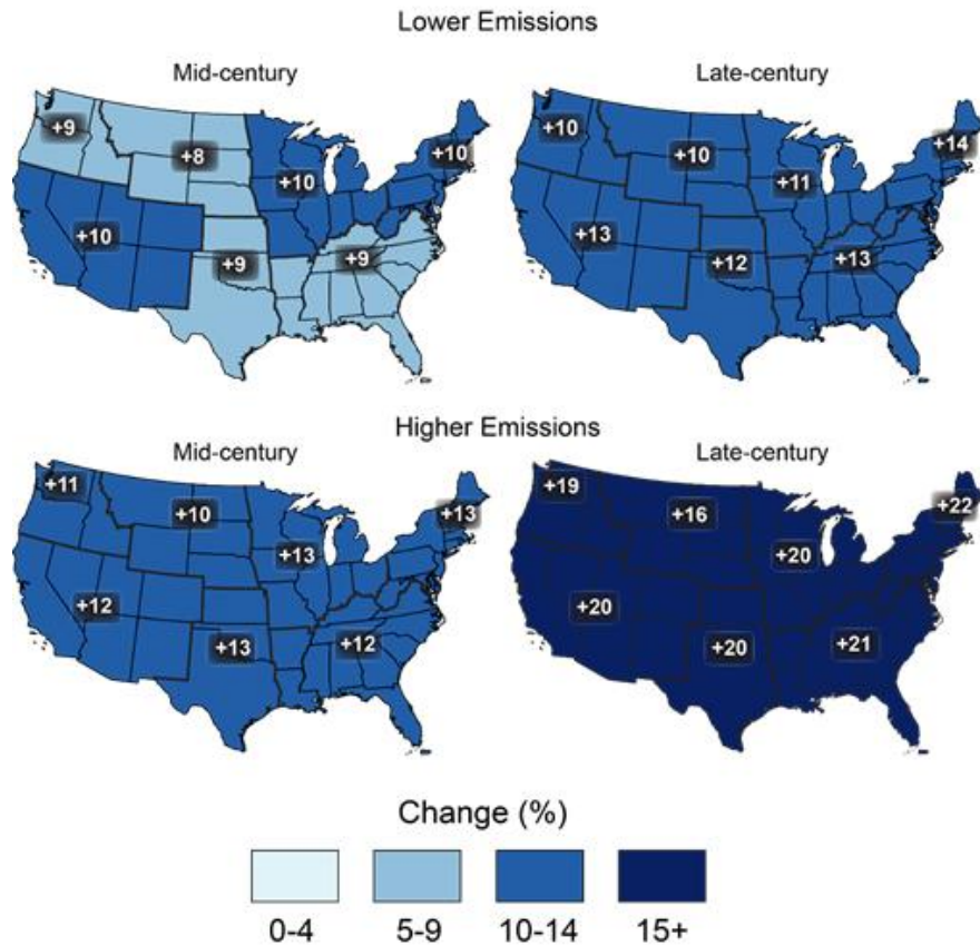
Figure 37: Projected change in the 20-year return period amount for daily precipitation for mid- (left) and late- (right) 21st century. Results are shown for a lower scenario (top; RCP4.5) and for a higher scenario (bottom; RCP8.5) (Easterling et al 2017).
