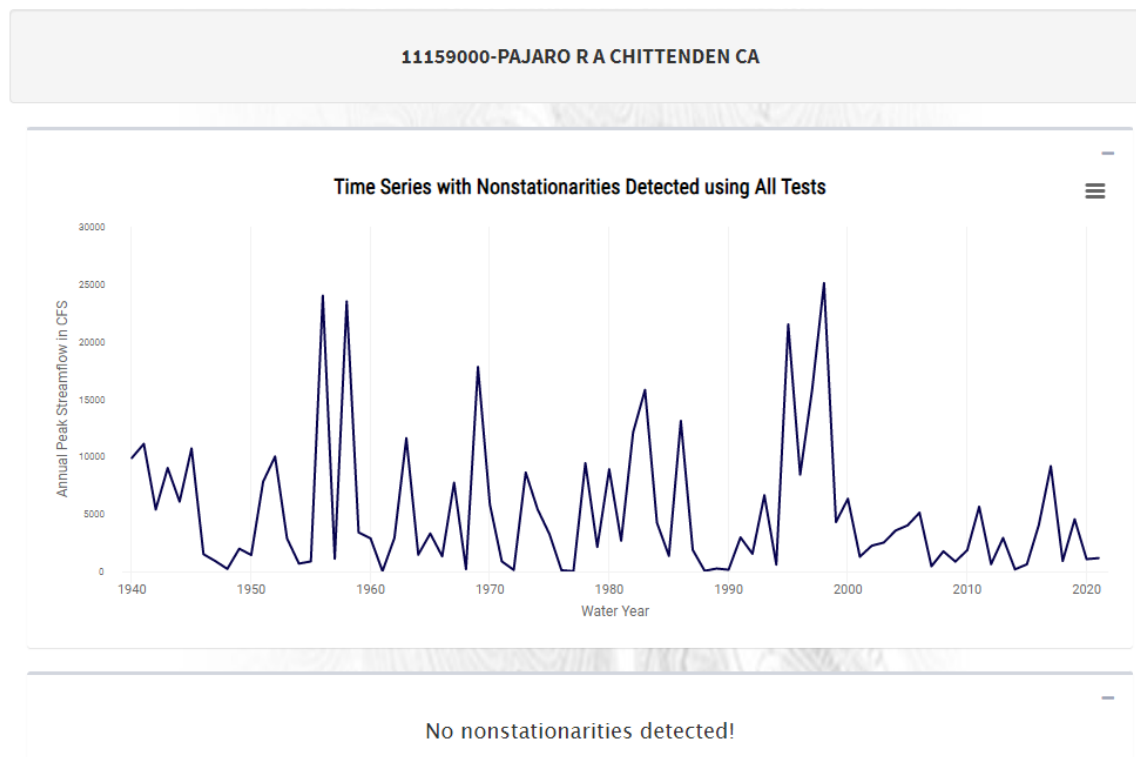
Figure 45. Nonstationarity detection results for annual peak streamflow for Pajaro River at Chittenden (11159000). No nonstationarities were detected.
