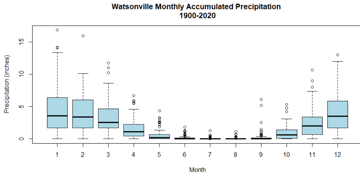
Figure 7: Box and whisker plot of monthly precipitation depths at Watsonville Waterworks rain gage.
