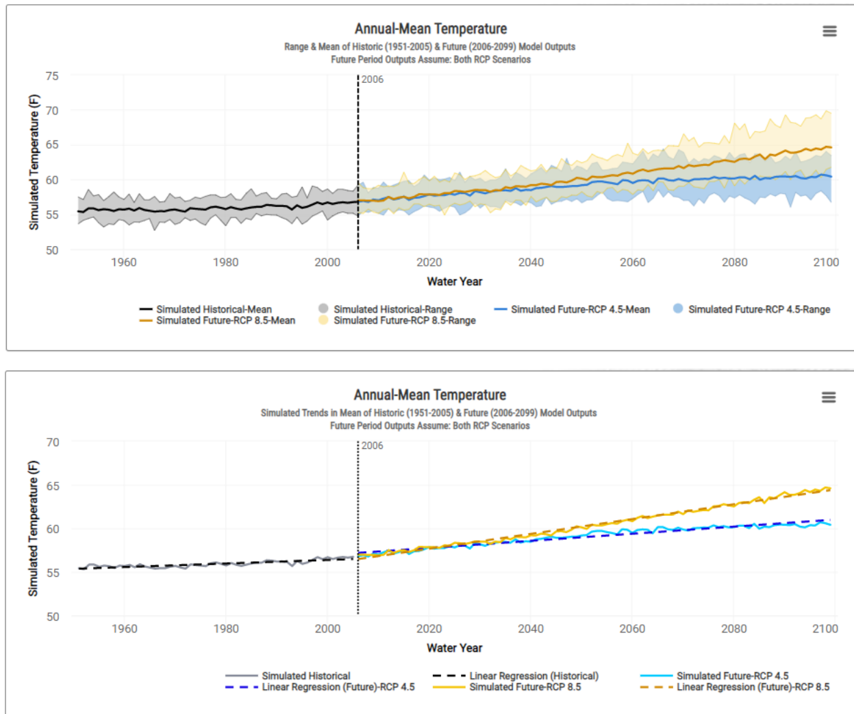
Figure 33: Annual Average of Daily Average Temperature. Range and mean (top) and trends (bottom) for RCP4.5 and RCP8.5. Statistically significant trends were detected for simulated historical and projected future temperatures under both RCP scenarios.
