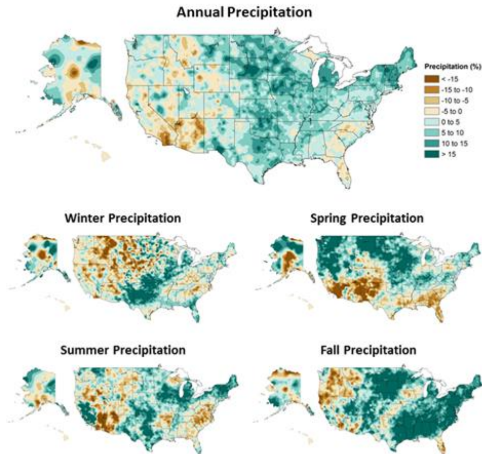
Figure 35: Annual and seasonal changes in average precipitation in the United States. Changes are the average for present-day (1986–2015) minus the average for the first half of the last century (1901–1960 for the contiguous United States, 1925–1960 for Alaska and Hawai‘i) divided by the average for the first half of the century. (Easterling et al 2017).
