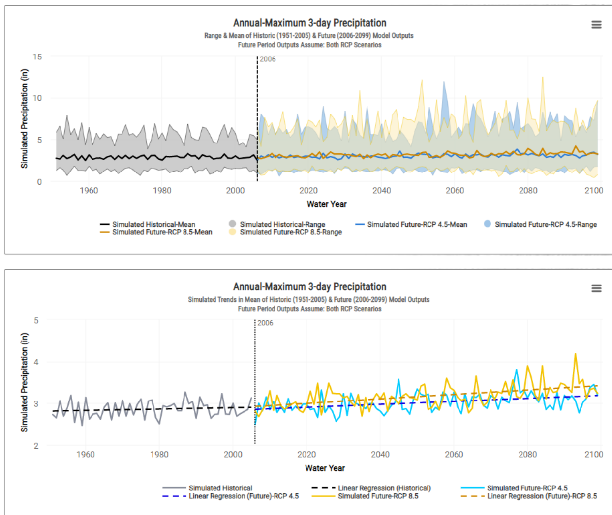
Figure 40. Annual Maximum of 3-day Sum of Daily Accumulated Precipitation. Range and mean (top) and trends (bottom) for RCP4.5 and RCP8.5. Statistically significant trends were detected for projected future precipitation under both scenarios. Statistically significant trend was not detected for simulated historical precipitation.
