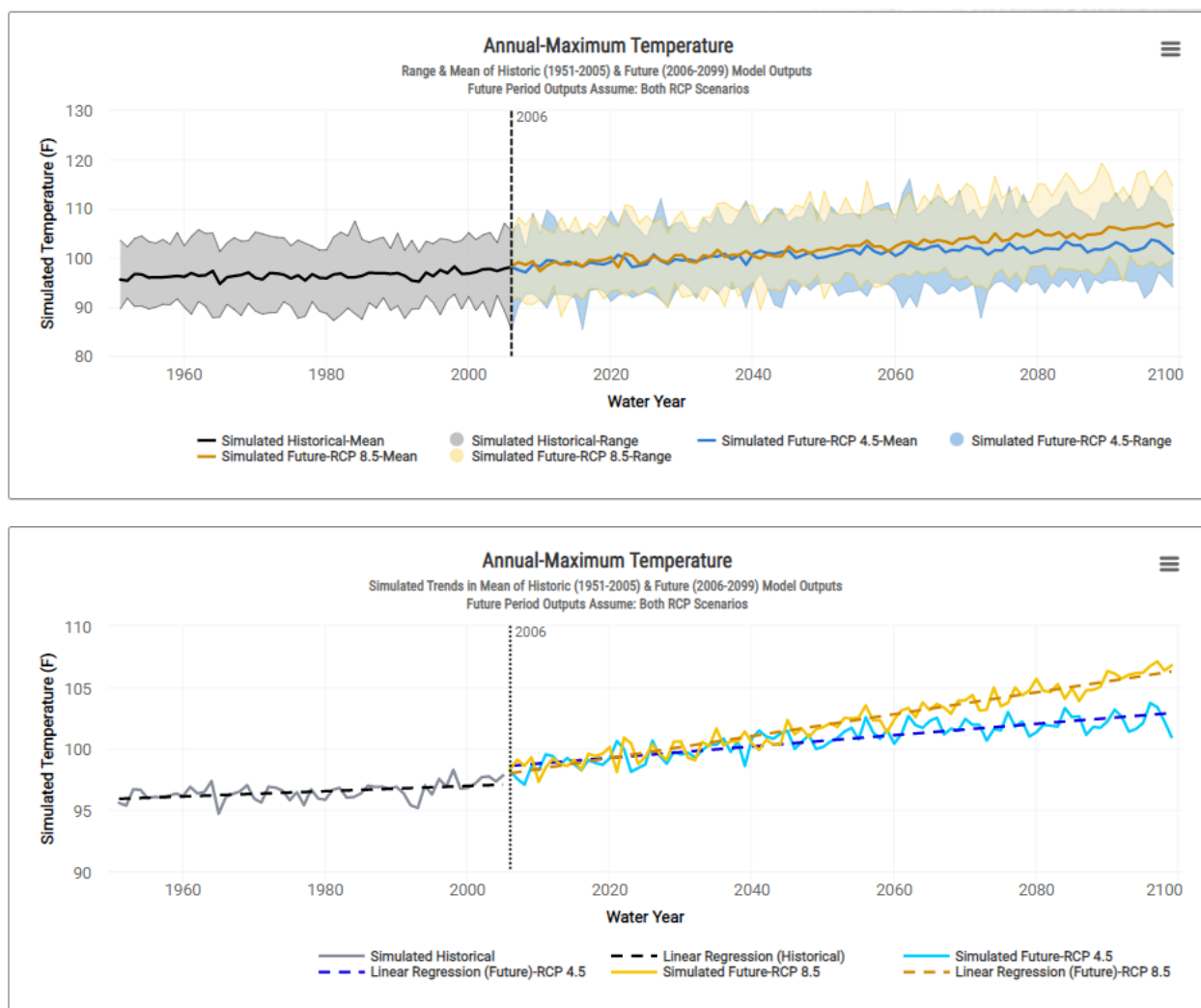
Figure 34: Annual Maximum of Daily Maximum Temperature. Range and mean (top) and trends (bottom) for RCP4.5 and RCP8.5. Statistically significant trends were detected for simulated historical and projected future temperatures under both RCP scenarios.
