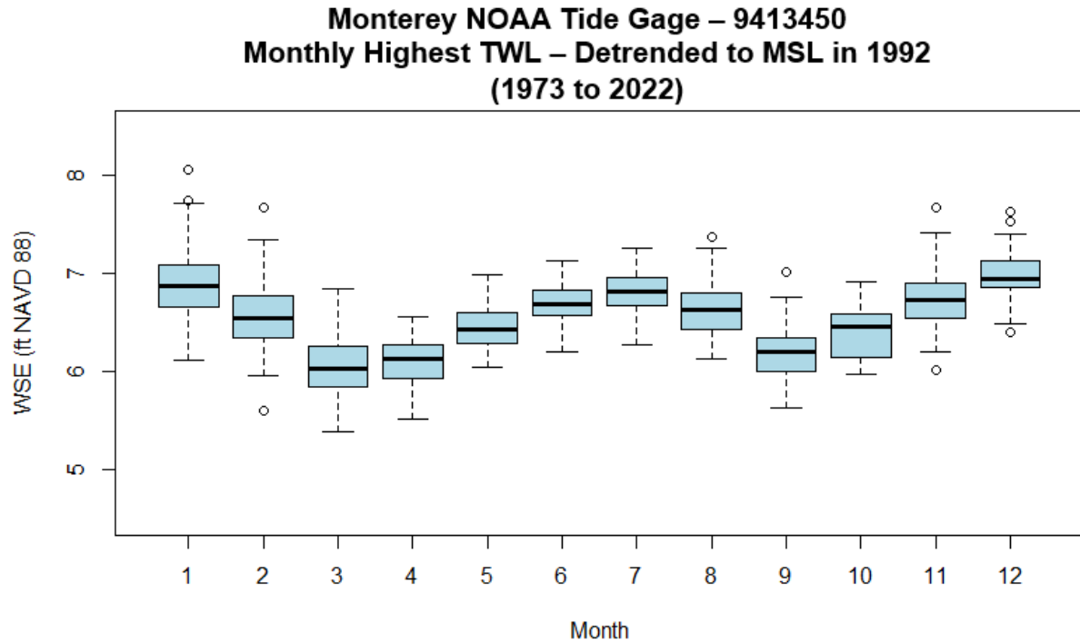
Figure 17: Distribution of Monthly Highest TWL (detrended to MSL in 1992) from 1973 to present at Monterey tide gage.
