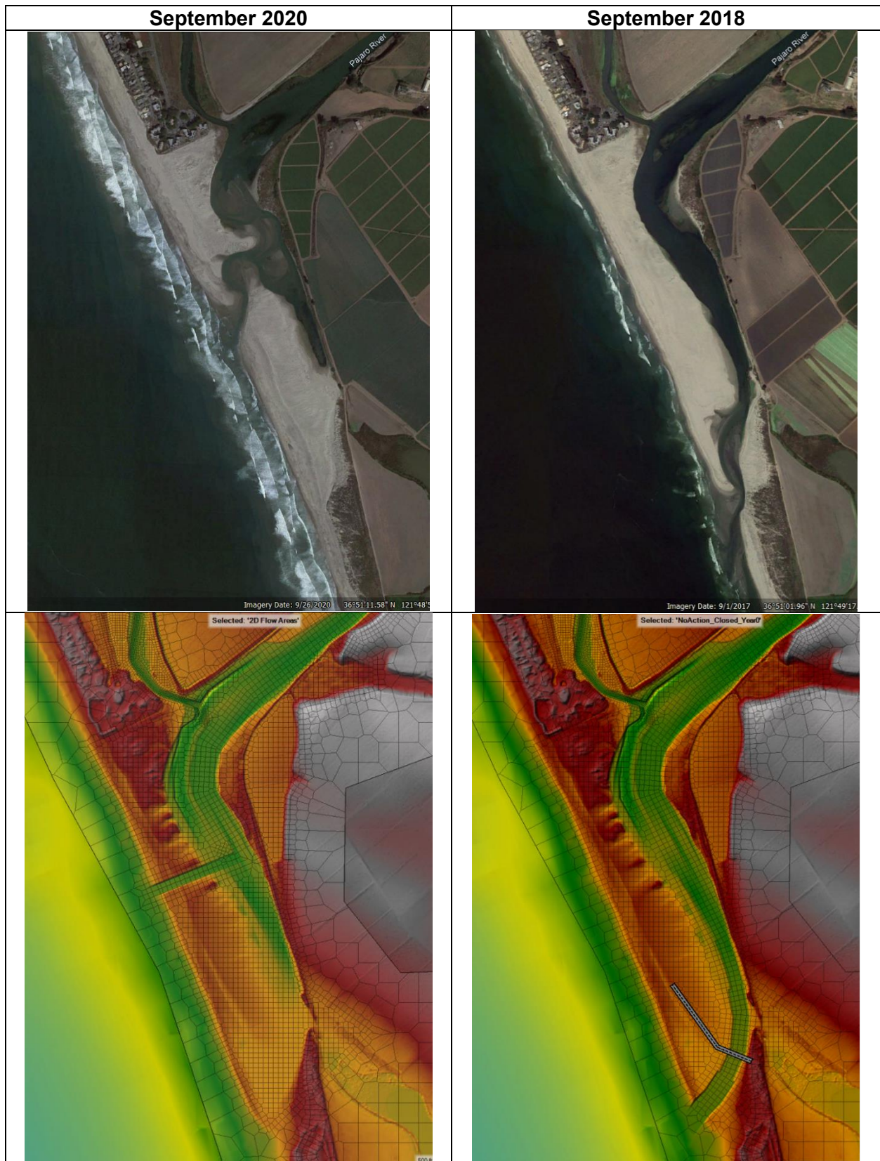
Figure 15: Lagoon aerals obtained from Google Earth and HEC-RAS terrains for the Open Lagoon model based on 2020 conditions (left panels) and the Closed Lagoon model based on 2018 conditions (right panels).
