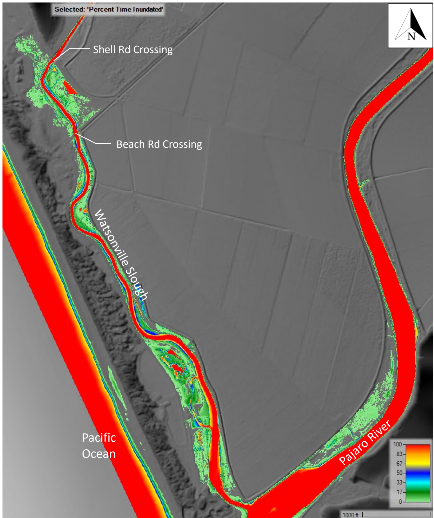
Figure 34: Percent time inundated – Crossing Improvements + Earthwork; Year 50; Open Lagoon, Dry Season
