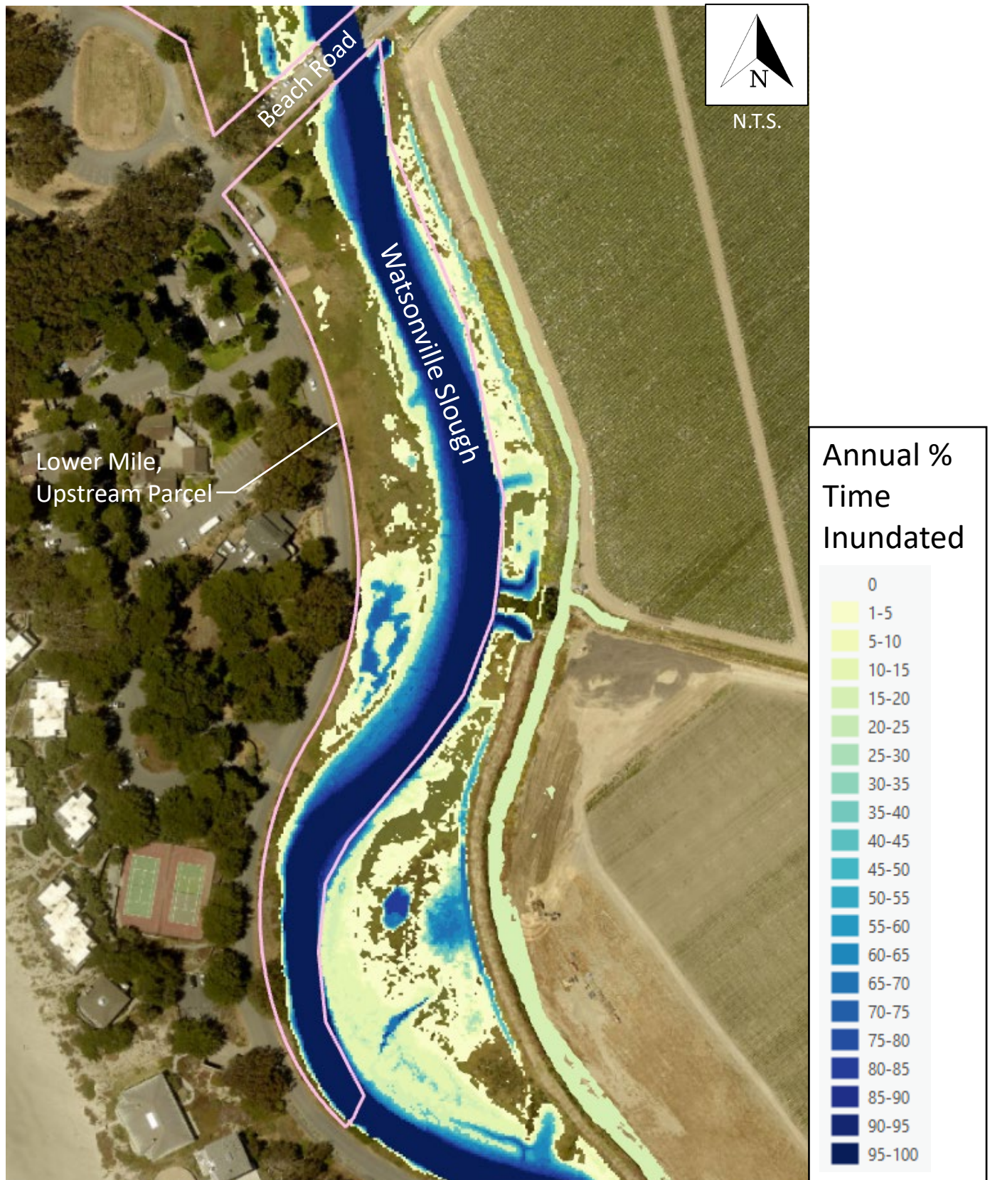
Figure 21: Annual PTI – Lower Mile, Upstream Parcel; Year 50; No Action
