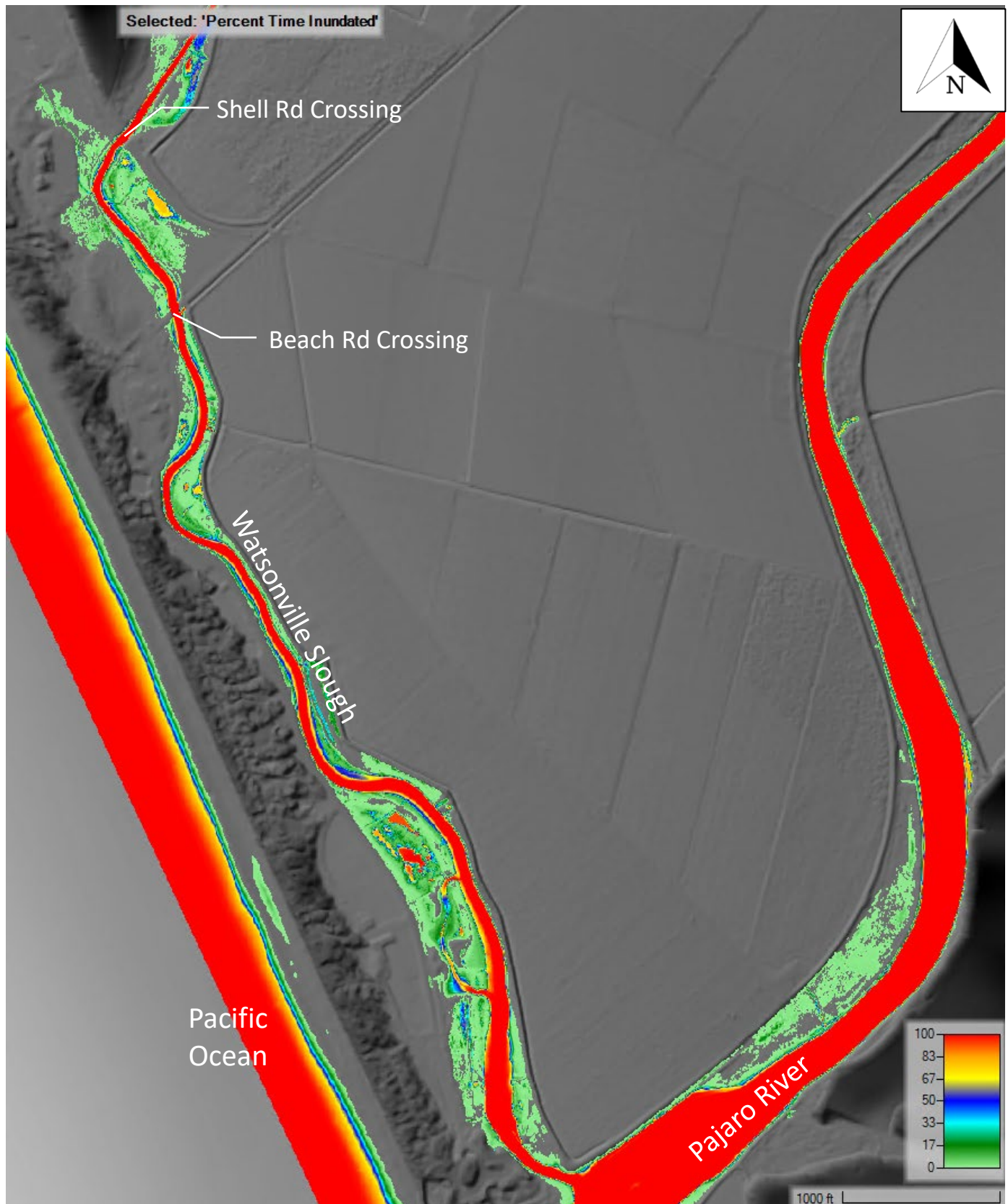
Figure 14: Percent time inundated – Crossing Improvements; Year 25; Open Lagoon, Wet Season
