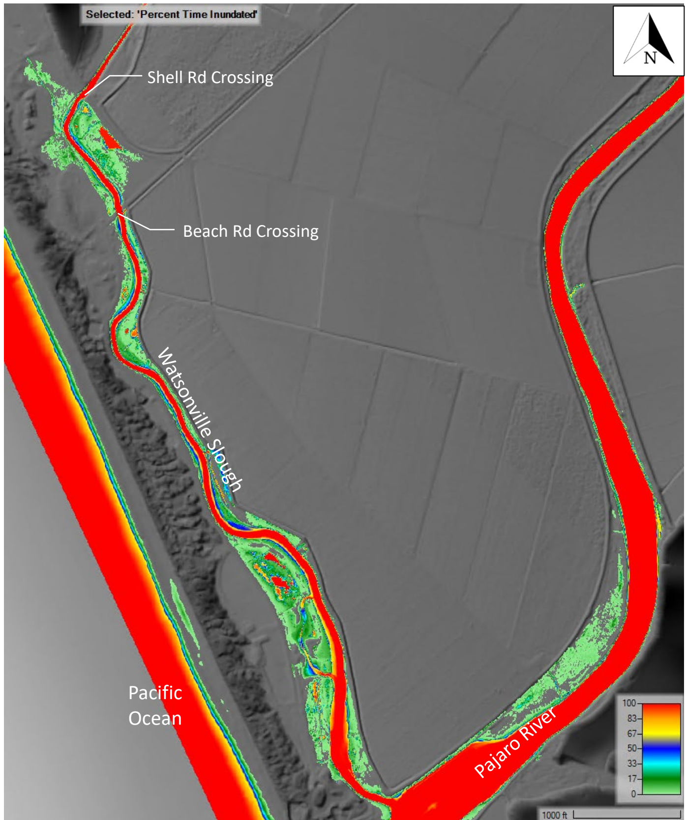
Figure 16: Percent time inundated – Crossing Improvements; Year 50; Open Lagoon, Dry Season
