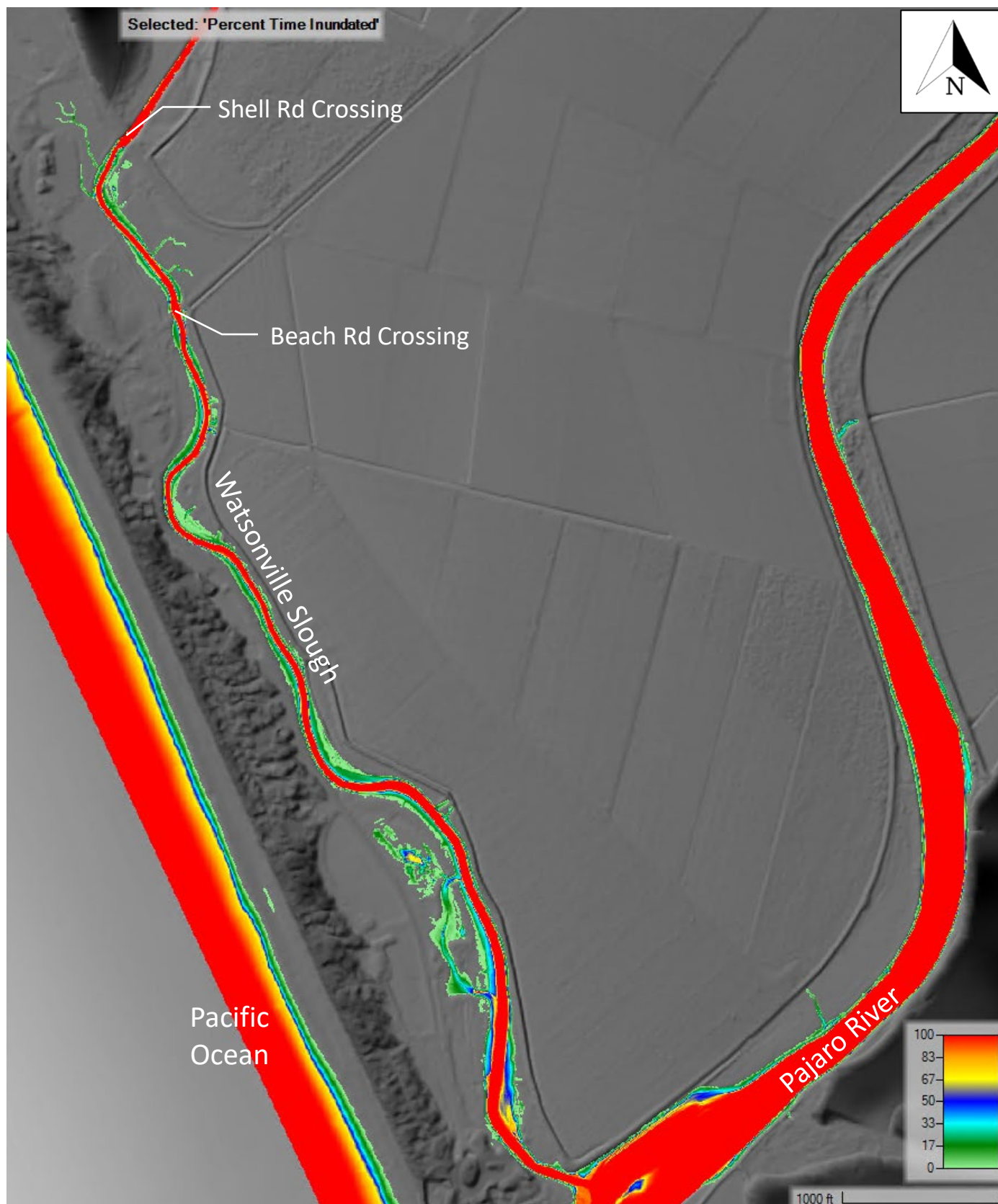
Figure 28: Percent time inundated – Crossing Improvements + Earthwork; Year 0; Open Lagoon, Dry Season
