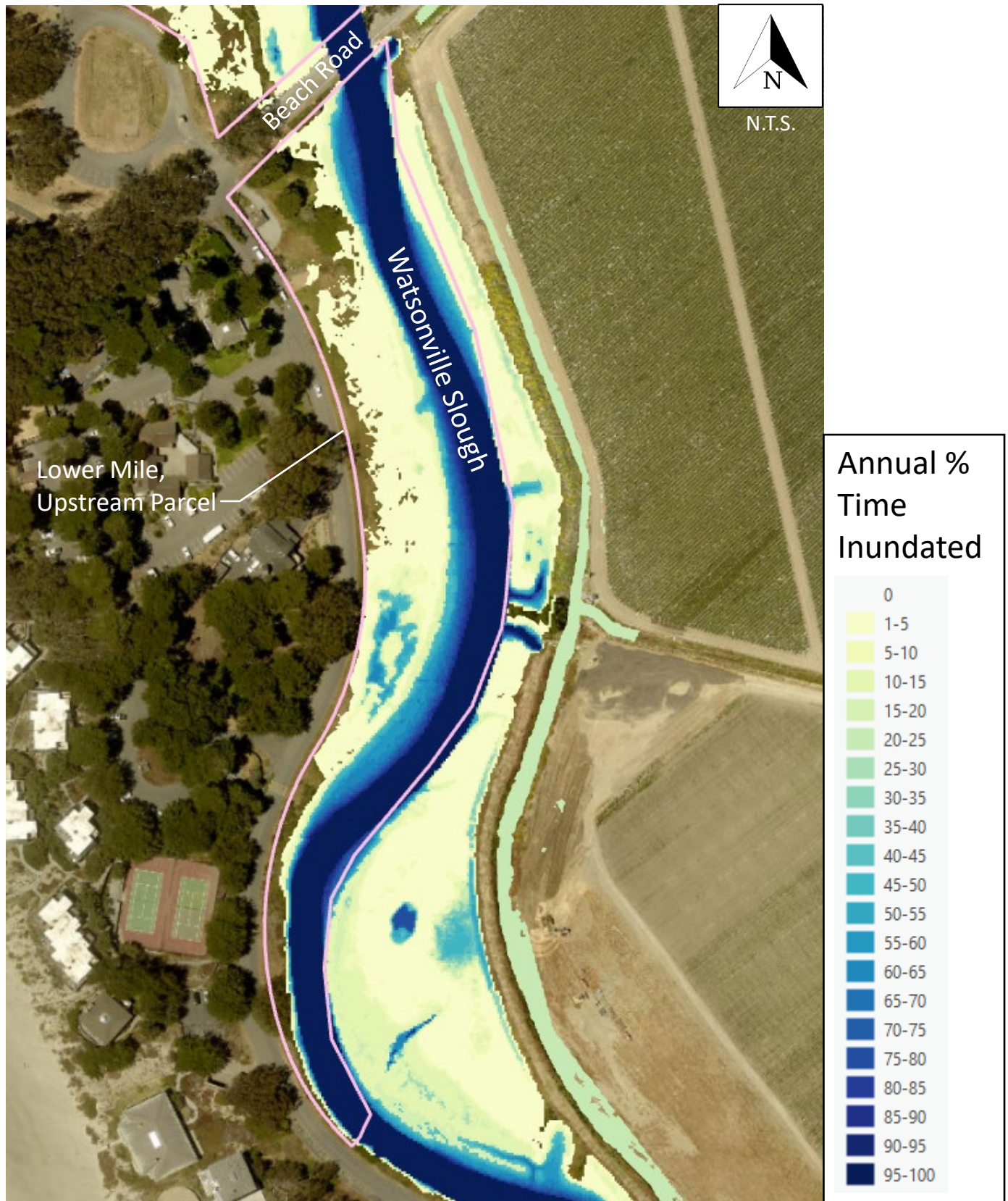
Figure 20: Annual PTI – Lower Mile, Upstream Parcel; Year 25; Crossing Improvements + Earthwork
