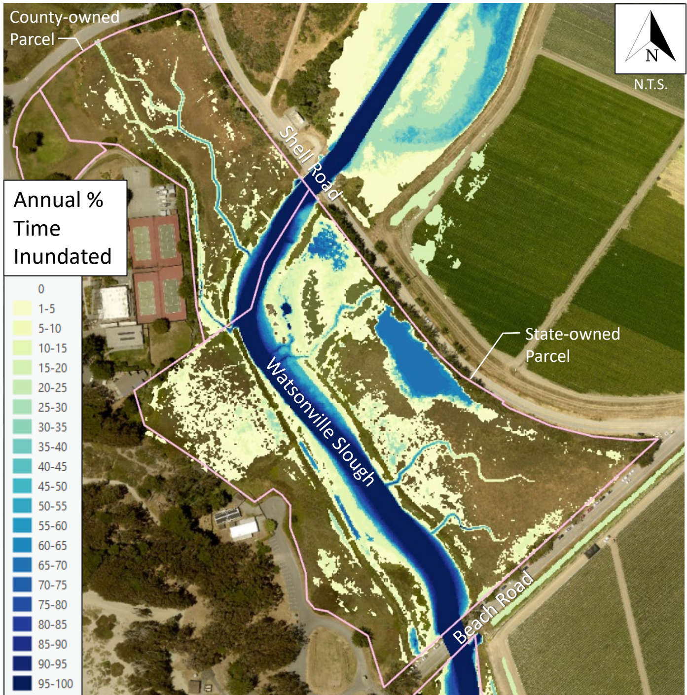
Figure 11: Annual PTI – State and County Parcels; Year 50; Earthwork
