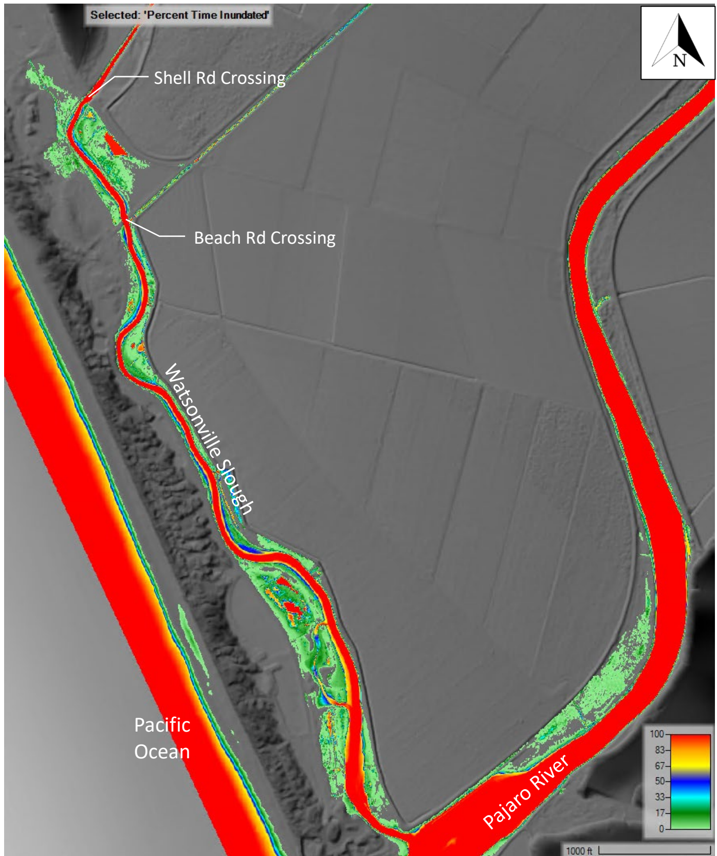
Figure 7: Percent time inundated – No Action; Year 50; Open Lagoon, Dry Season
