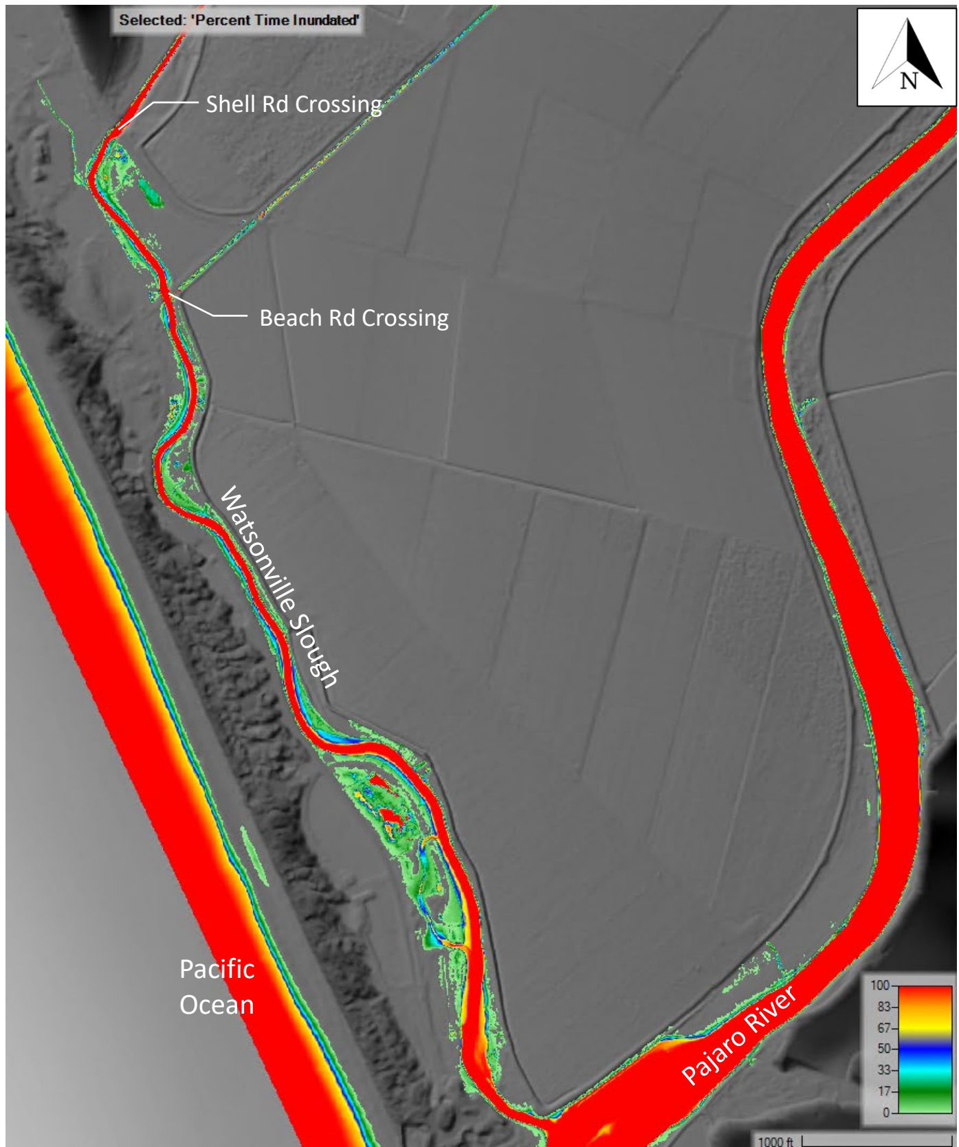
Figure 4: Percent time inundated – No Action; Year 25; Open Lagoon, Dry Season
