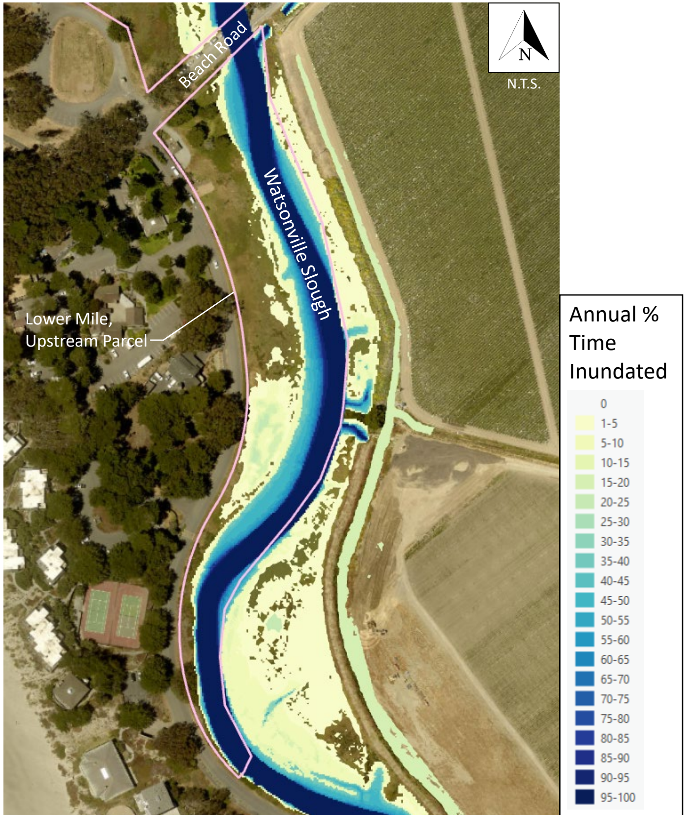
Figure 15: Annual PTI – Lower Mile, Upstream Parcel; Year 0; Earthwork
