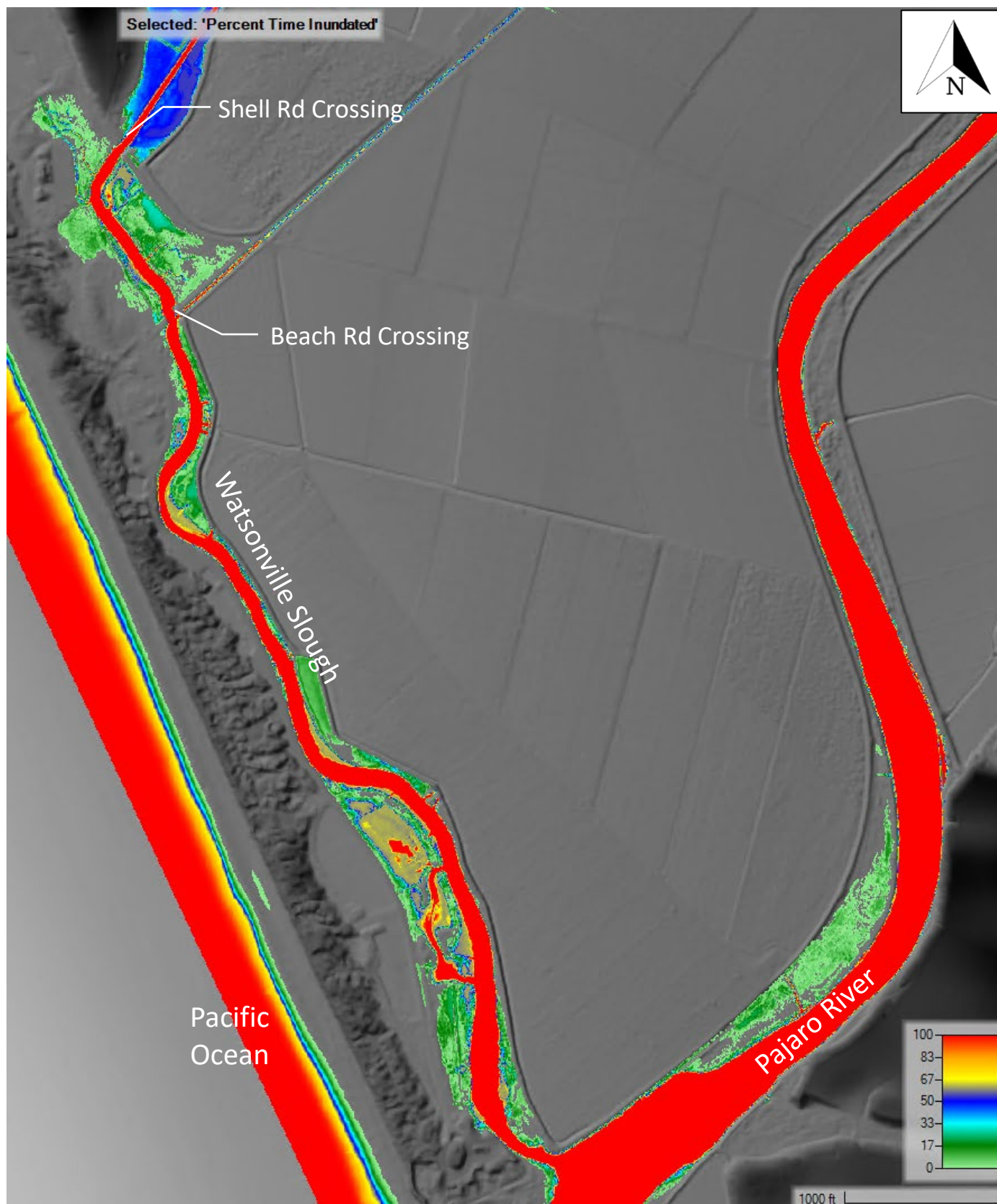
Figure 27: Percent time inundated – Earthwork; Year 50; Closed Lagoon, Wet Season
