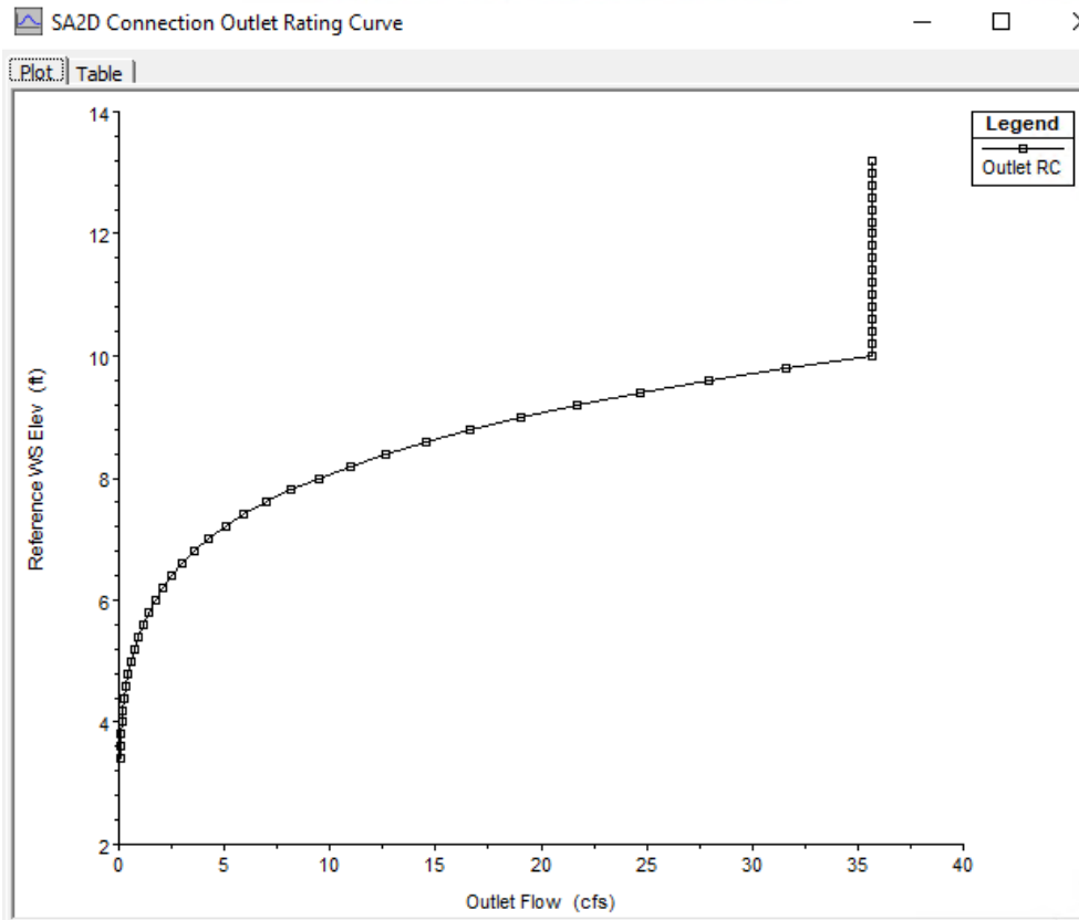
Figure 20: Rating curve for infiltration and seepage losses for the Closed Lagoon model runs.
