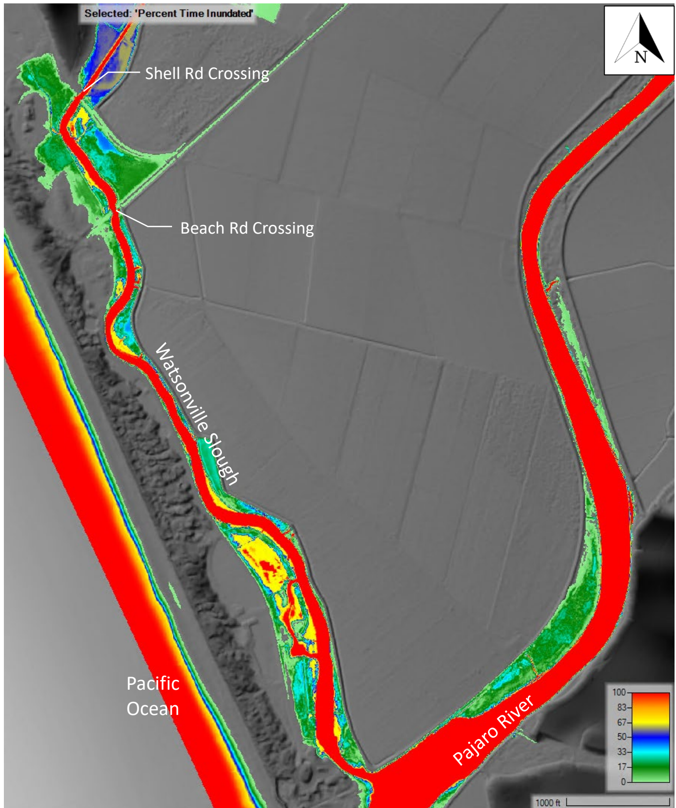
Figure 12: Percent time inundated – Crossing Improvements; Year 0; Closed Lagoon, Wet Season
