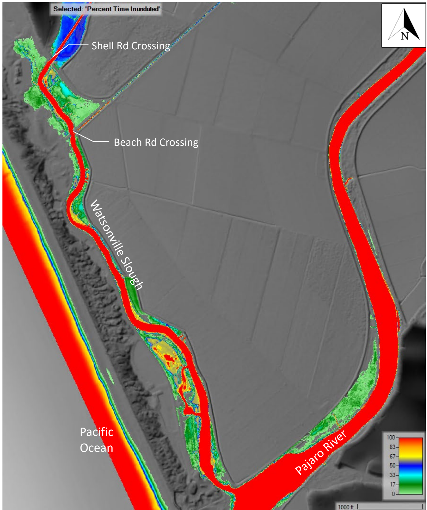
Figure 21: Percent time inundated – Earthwork; Year 0; Closed Lagoon, Wet Season
