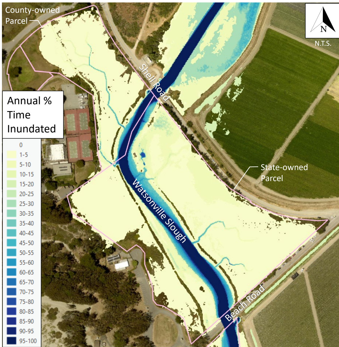
Figure 4: Annual PTI – State and County Parcels; Year 0; Crossing Improvements + Earthwork
