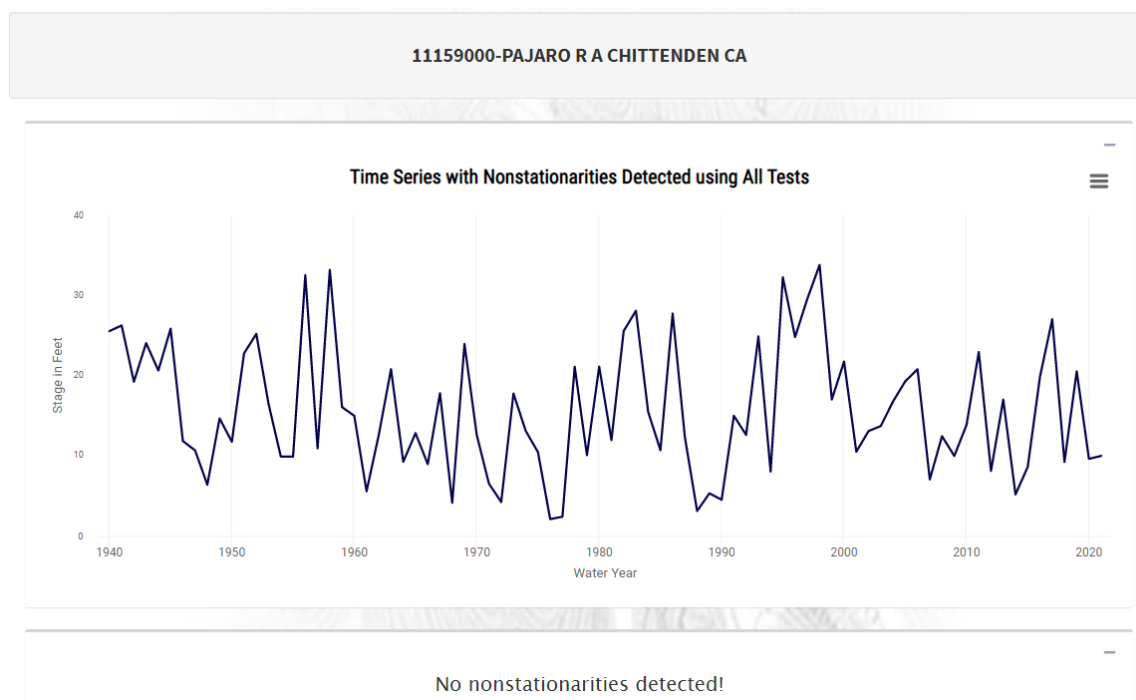
Figure 46. Nonstationarity detection results for annual peak stage for Pajaro River at Chittenden (11159000). No nonstationarities were detected.
