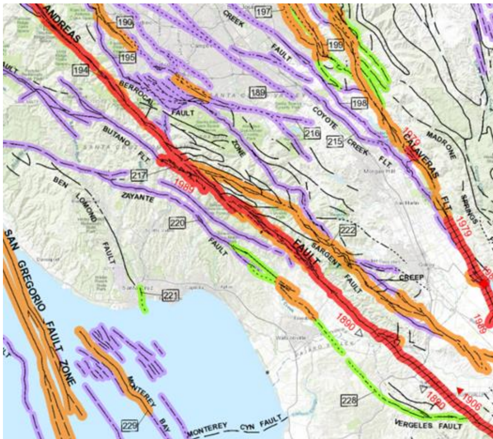
Figure 3. Fault Activity Map of California (Jennings, 2010)
