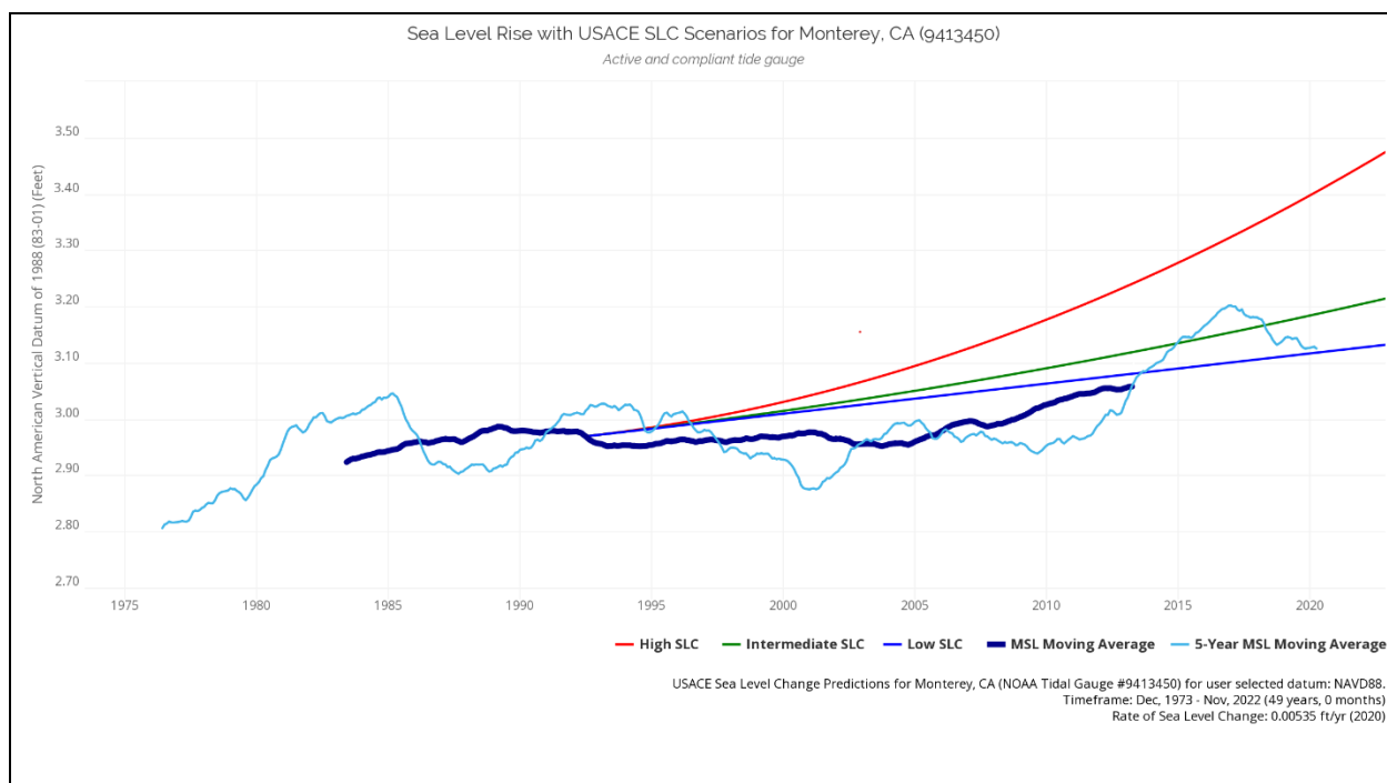
Figure 50: Historical and projected sea level change at Monterey, CA from the USACE Sea Level Tracker, based on the observed mean sea level (MSL) record. The light blue line represents the 5-year MSL moving average and the dark blue line the 19-year moving average.
