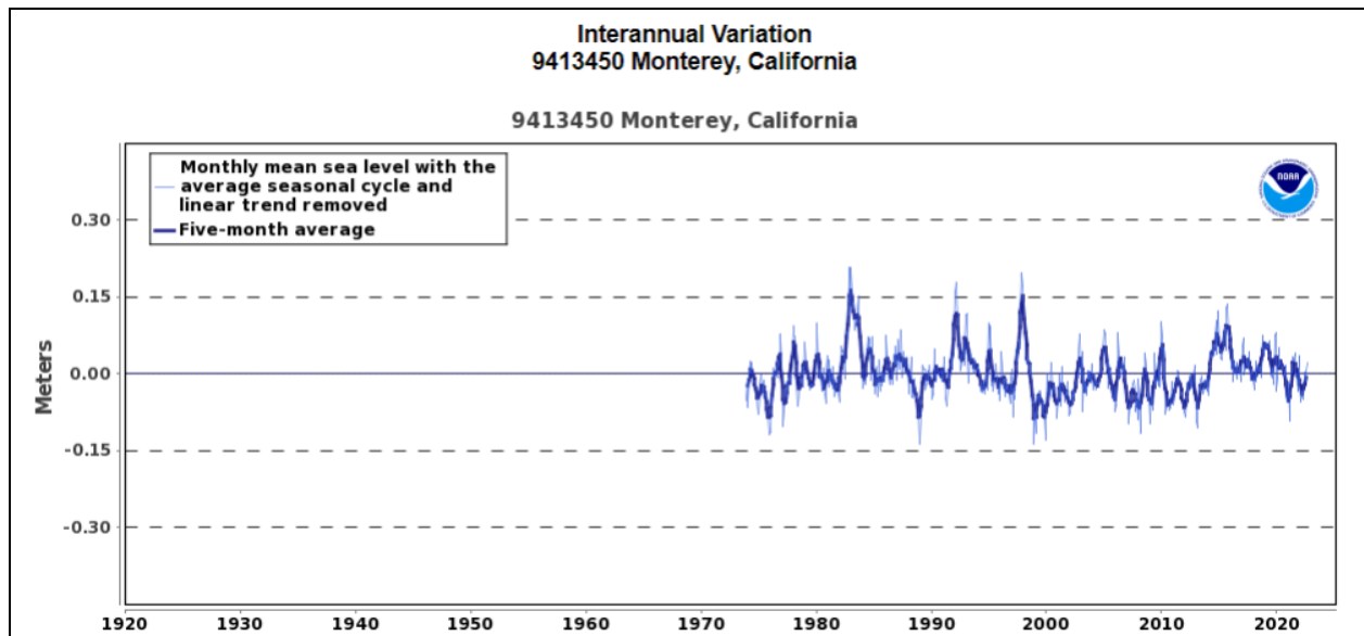
Figure 52: Interannual variation at the NOAA Monterey tide gage (Station #9413450).
