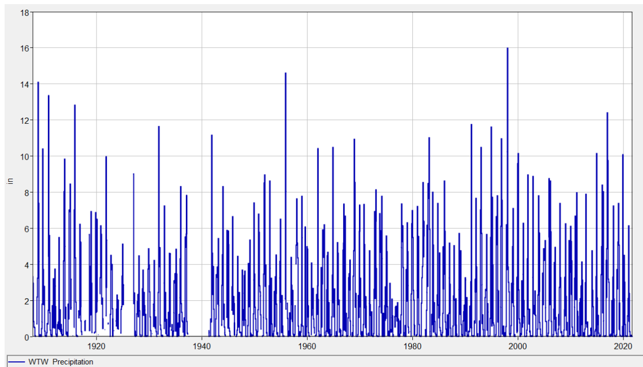
Figure 4: Monthly precipitation depths from 1908 to 2021 at the rain gage at Watsonville Waterworks.
