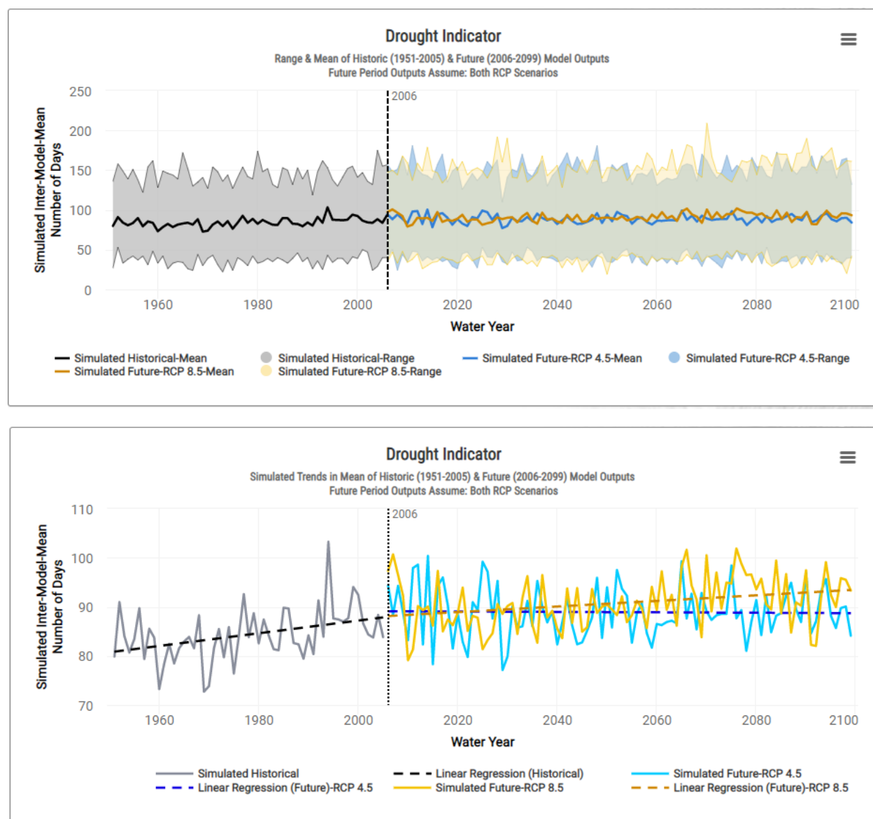
Figure 47. Annual Maximum of Number of Consecutive Dry Days. Range and mean (top) and trends (bottom) for RCP4.5 and RCP8.5. Statistically significant trends were detected for simulated historical precipitation and projected future precipitation under RCP8.5. A statistically significant trend was not detected for RCP4.5.
