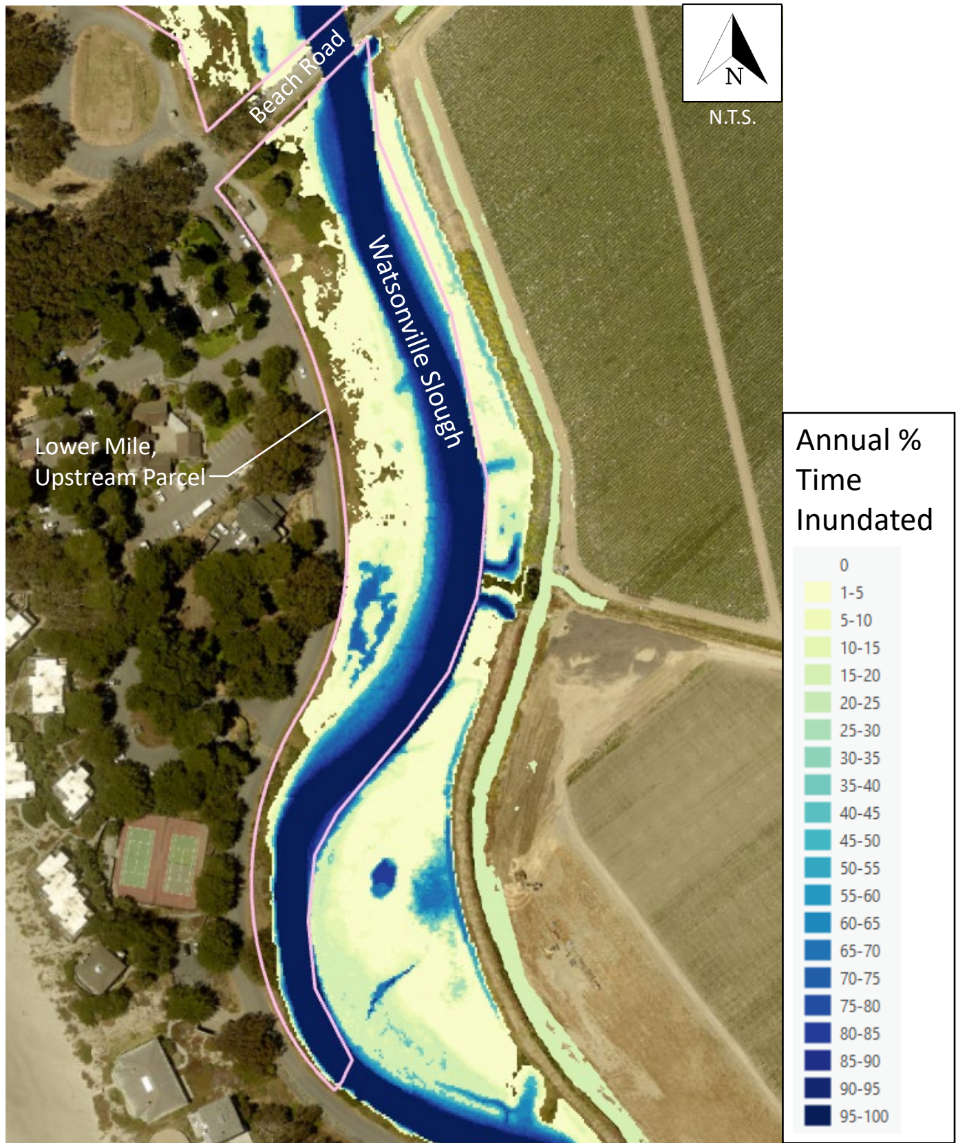
Figure 24: Annual PTI – Lower Mile, Upstream Parcel; Year 50; Crossing Improvements + Earthwork
