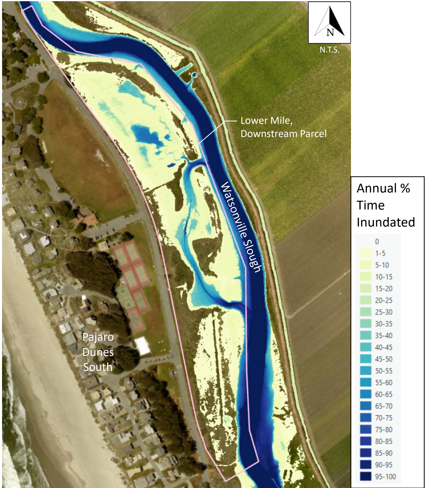
Figure 25: Annual PTI – Lower Mile, Downstream Parcel; Year 0; No Action
