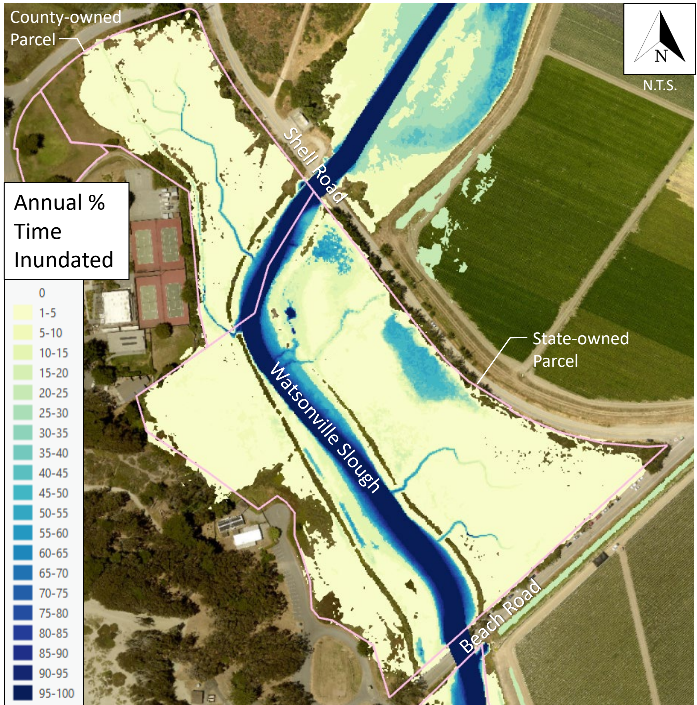
Figure 8: Annual PTI – State and County Parcels; Year 25; Crossing Improvements + Earthwork
