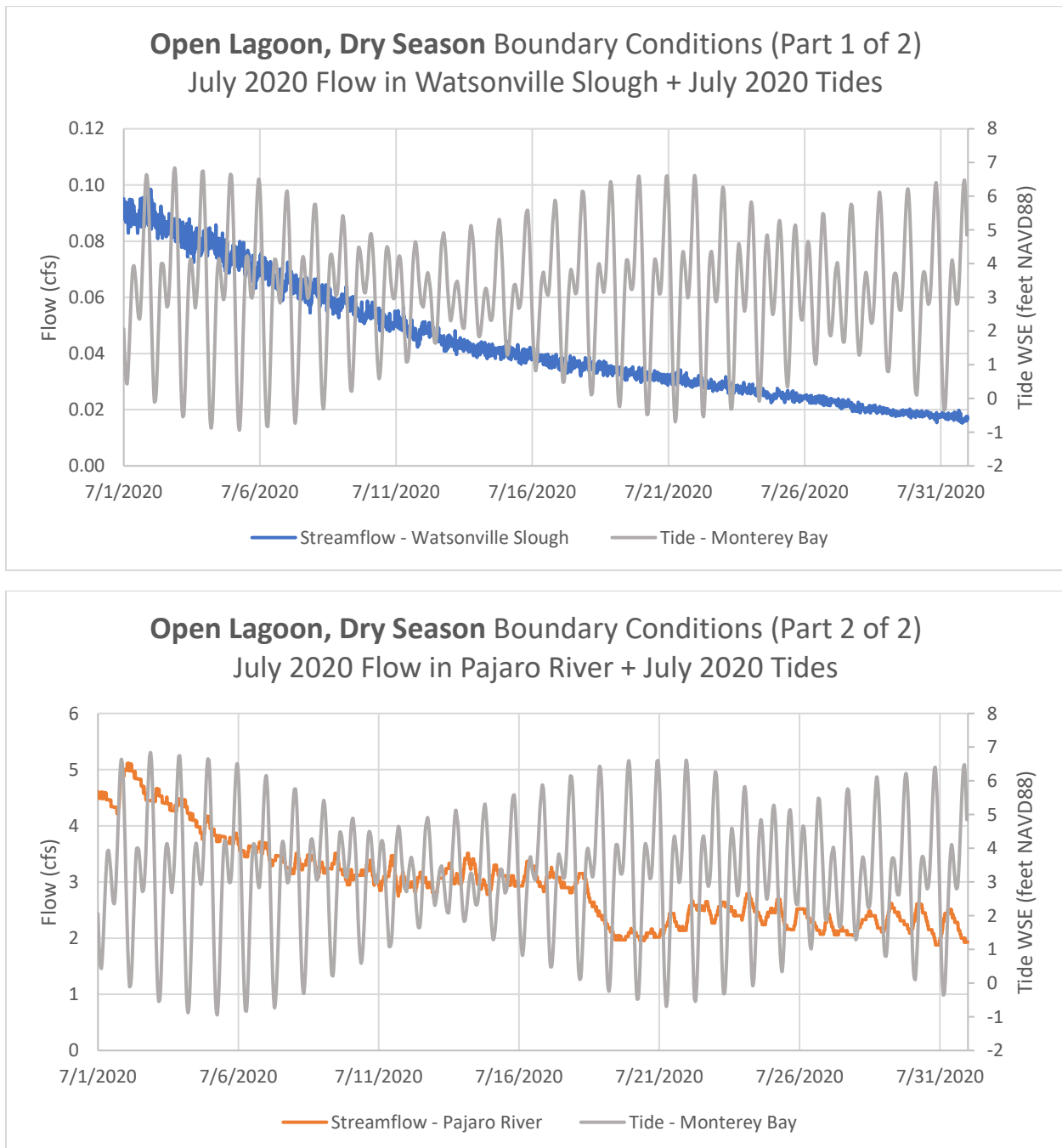
Figure 3: Hydrologic boundary conditions selected as representative of the Open Lagoon, Dry Season hydrologic regime.
