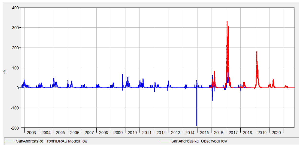
Figure 5: Observed (red) and modeled (blue) streamflow data record in Watsonville Slough at San Andreas Road. Note, negative flow values in the modeled record indicate flow in the upstream direction, due to tidal conditions.
