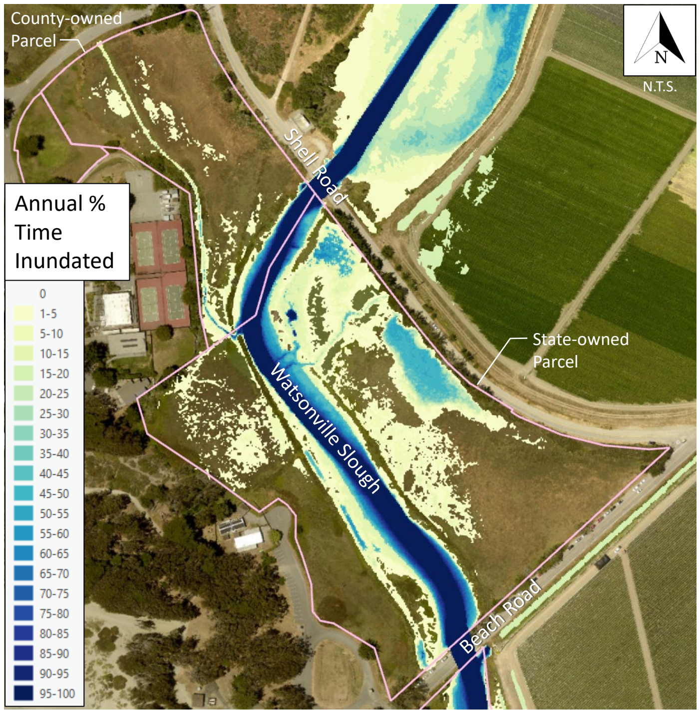
Figure 5: Annual PTI – State and County Parcels; Year 25; No Action
