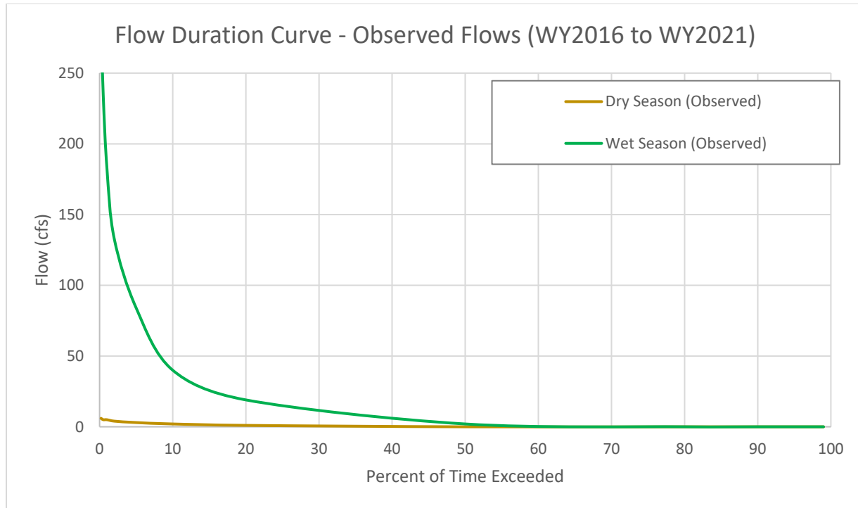
Figure 15: Flow duration curve for observed flows in Watsonville Slough from WY2016 to WY2021.
