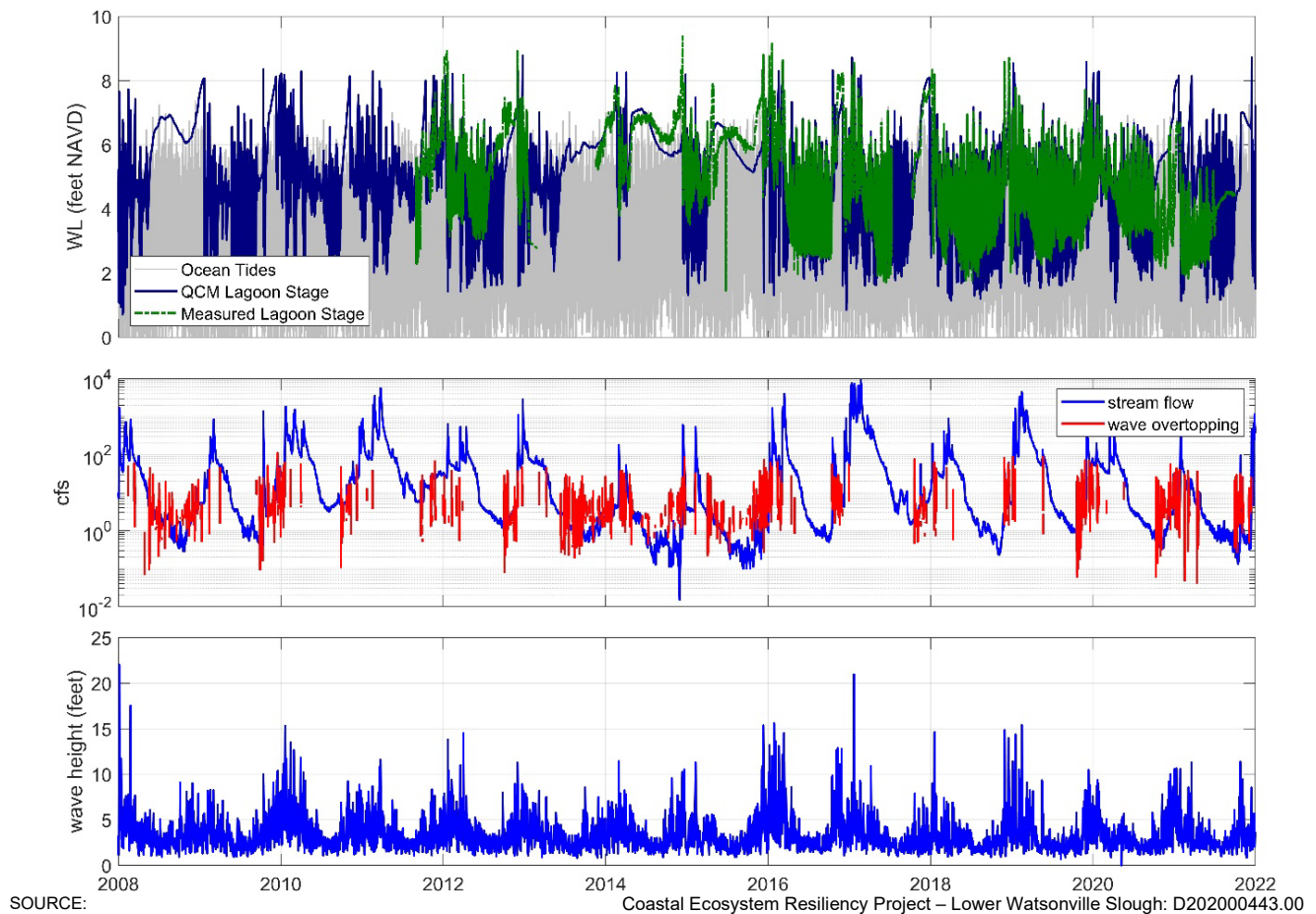
Figure 5 QCM-data comparisons for ‘Baseline’ scenario. Top: QCM calculations of lagoon water levels compared to the observations of lagoon water level and ocean tides. Middle: Observations of streamflow with model estimates of wave overtopping rates. Bottom: Observations of nearshore wave heights.
