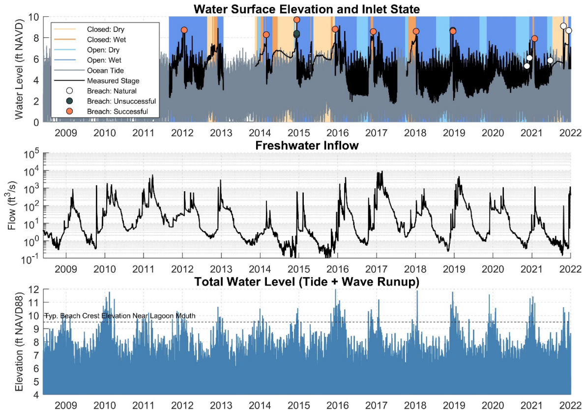
Figure 4 Comparison of (top) observed water levels in Watsonville Slough and nearby ocean tides, (middle) combined streamflow to the lagoon, and (bottom) Total water level on the beach.
