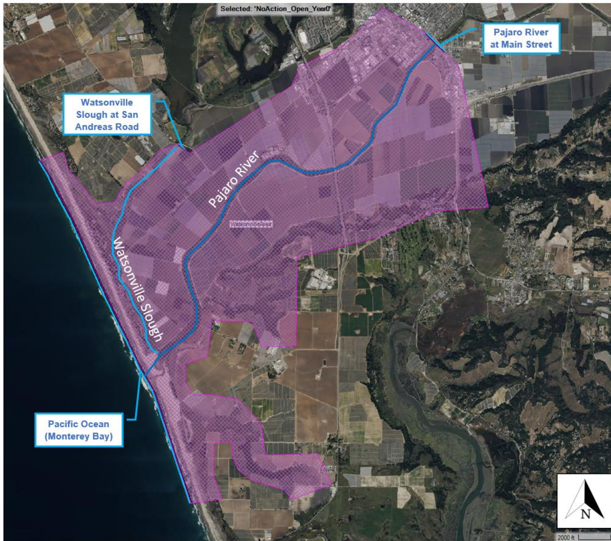
Figure 13: Extents of HEC-RAS model domain with upstream and downstream boundary conditions identified.
