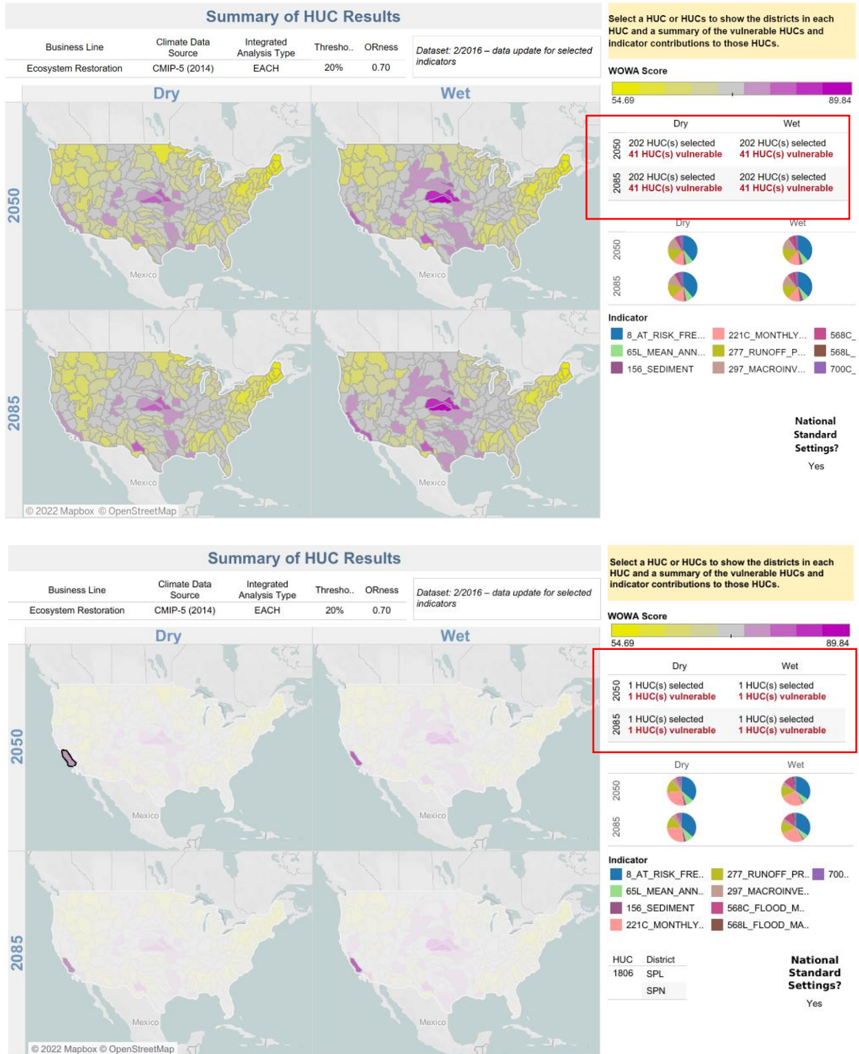
Figure 53. Top: For the Ecosystem Restoration Line of Business, approximately 20% of included HUC-4 watersheds (41 of 202) are considered most vulnerable nationwide. Bottom: HUC 1806 (Central California Coastal) is considered vulnerable under all epoch/scenario combinations.
