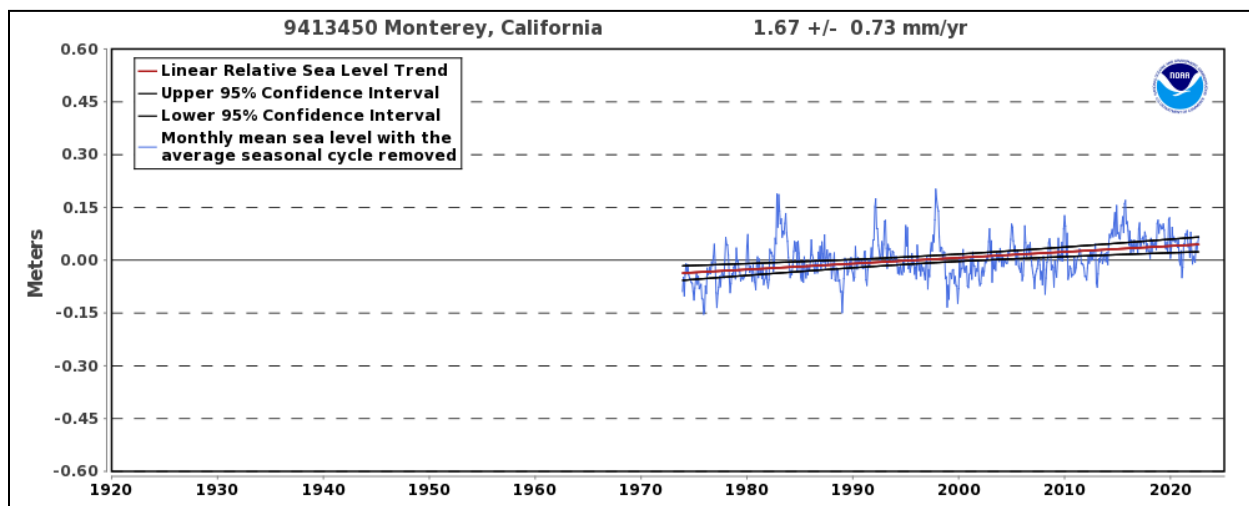
Figure 49: Relative sea level trend for NOAA Monterey station (#9413450), based on mean sea level data from 1973 to 2021. The relative sea level change trend is +1.67 mm/year (0.005479 ft/yr) with a 95% confidence interval of +/- 0.73 mm/yr (0.002395 ft/yr). This translates to 0.55 feet over 100 years.
