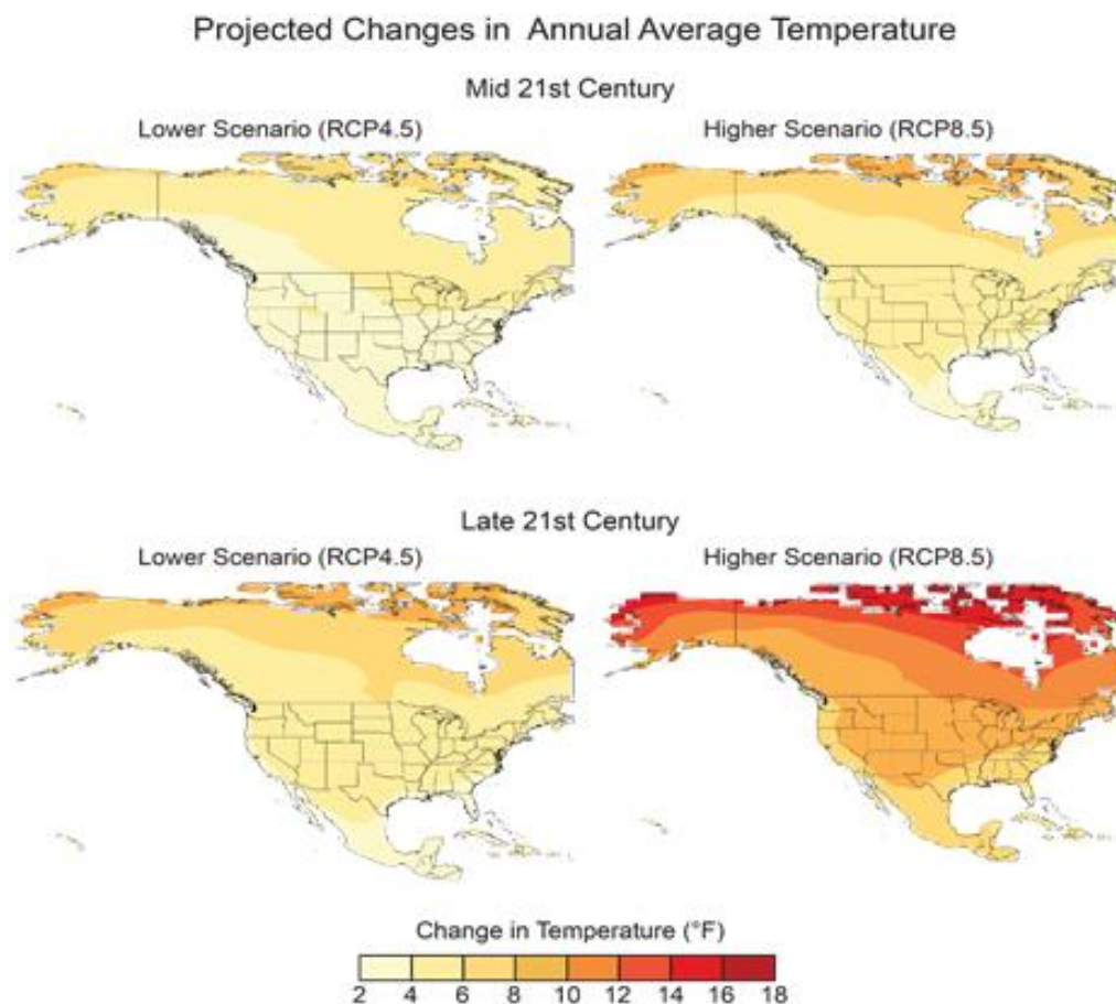
Figure 31: Projected changes in annual average temperatures (°F) for mid and late 21st century under low and high Representative Concentration Pathways (RCP) scenarios. Changes are the difference between the average for mid-century (2036–2065; top) or late-century (2070–2099, bottom) and the average for near-present (1976–2005) (Vose et al 2017).
