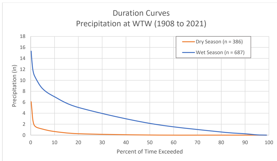
Figure 11: HEC-SSP duration analysis for monthly precipitation depths for dry season and wet season.
