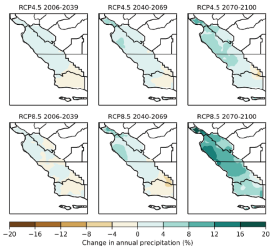
Figure 38: Projected change in annual precipitation from historic baseline of 1961-1990 in California Central Coast Region (Langridge 2018).
