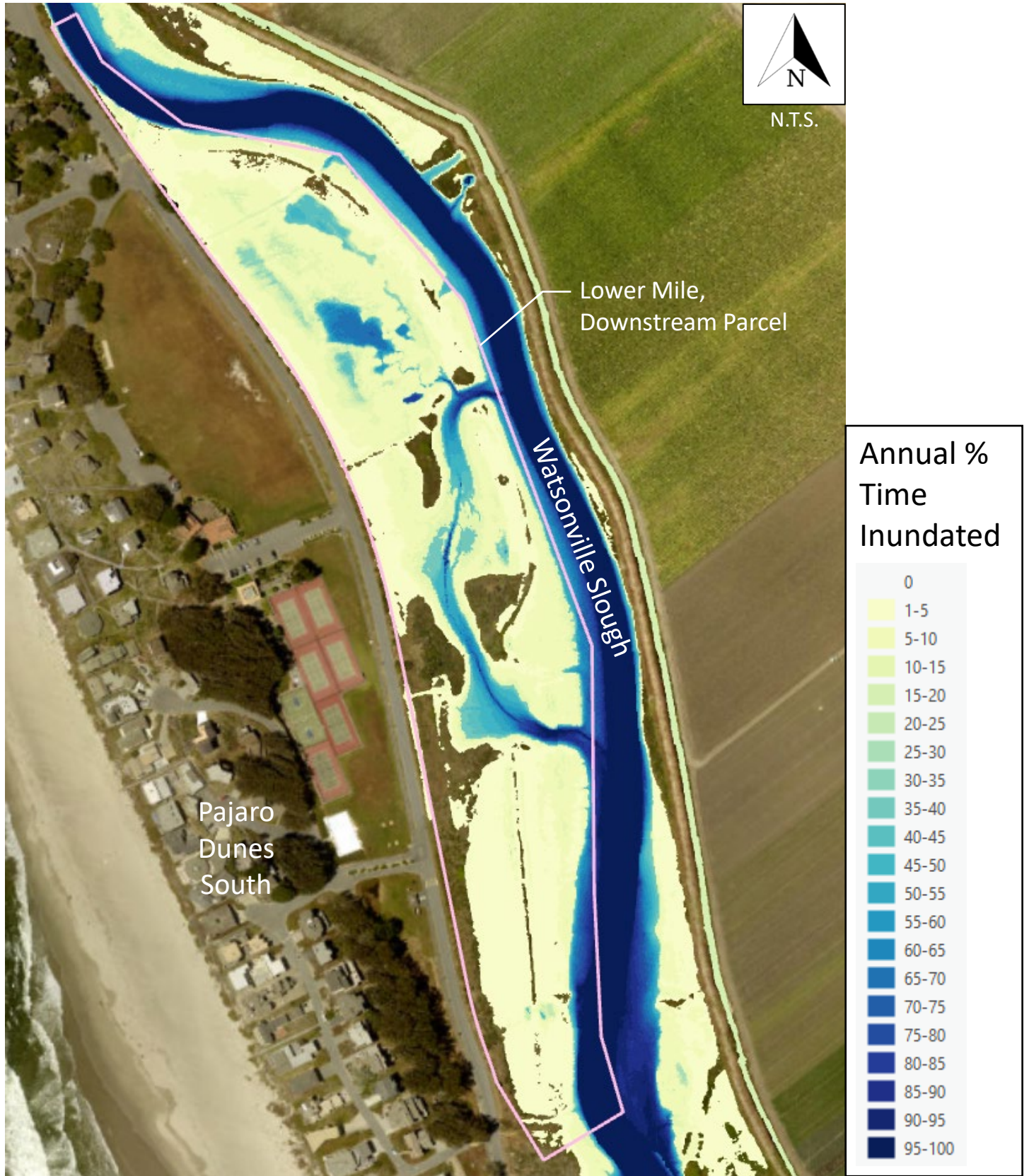
Figure 28: Annual PTI – Lower Mile, Downstream Parcel; Year 0; Crossing Improvements + Earthwork
