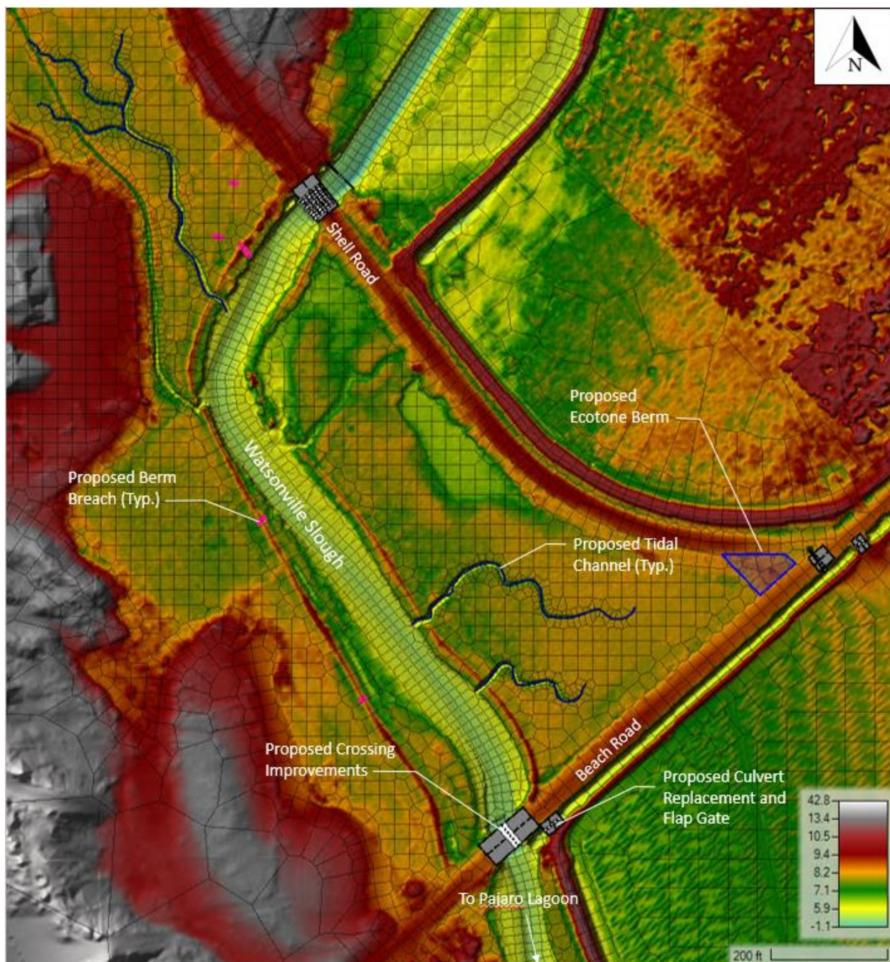
Figure 10: Crossing Improvements + Earthwork project scenario.
