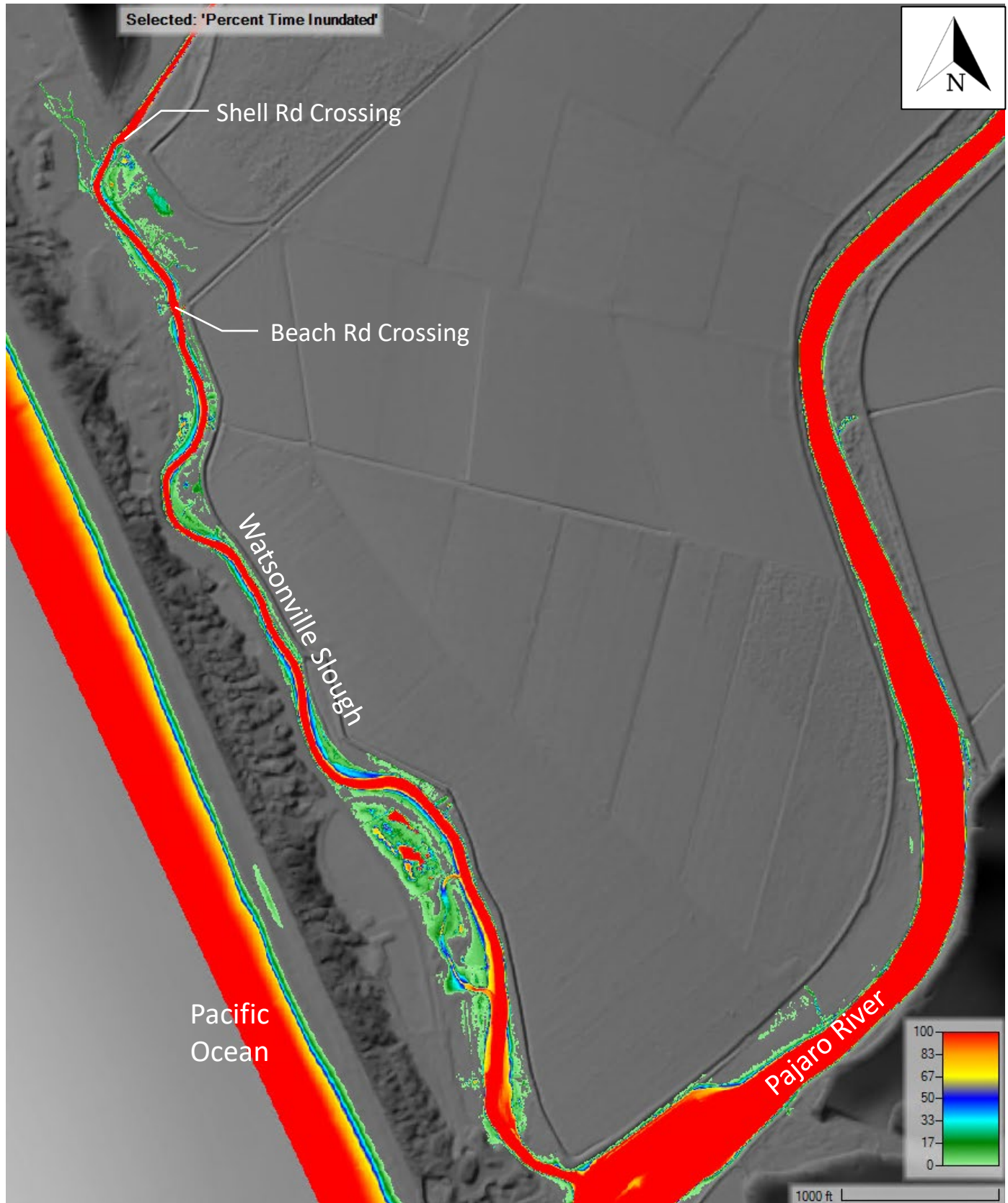
Figure 31: Percent time inundated – Crossing Improvements + Earthwork; Year 25; Open Lagoon, Dry Season
