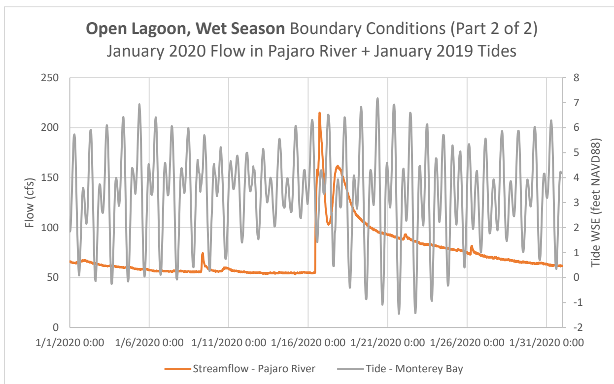
Figure 4: Hydrologic boundary conditions selected as representative of the Open Lagoon, Wet Season hydrologic regime.
