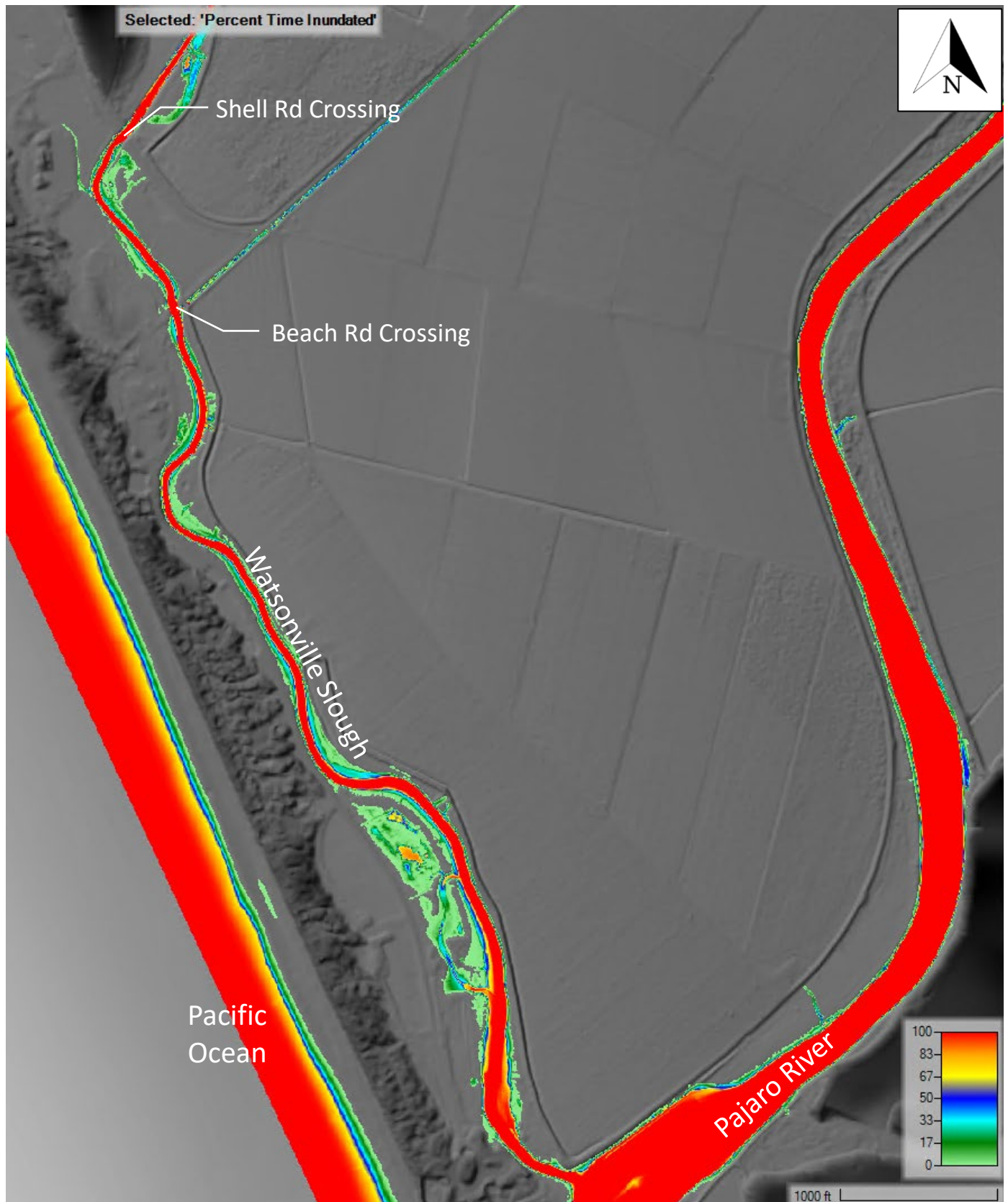
Figure 2: Percent time inundated – No Action; Year 0; Open Lagoon, Wet Season
