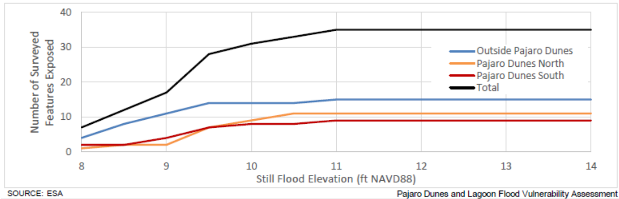
Figure 12. Total number of surveyed features exposed by range of still water flooding elevations (ESA, 2018)
