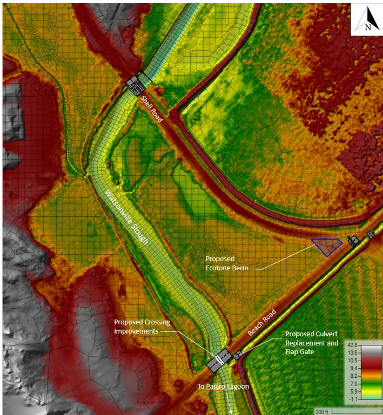
Figure 8: Crossing Improvements project scenario.
