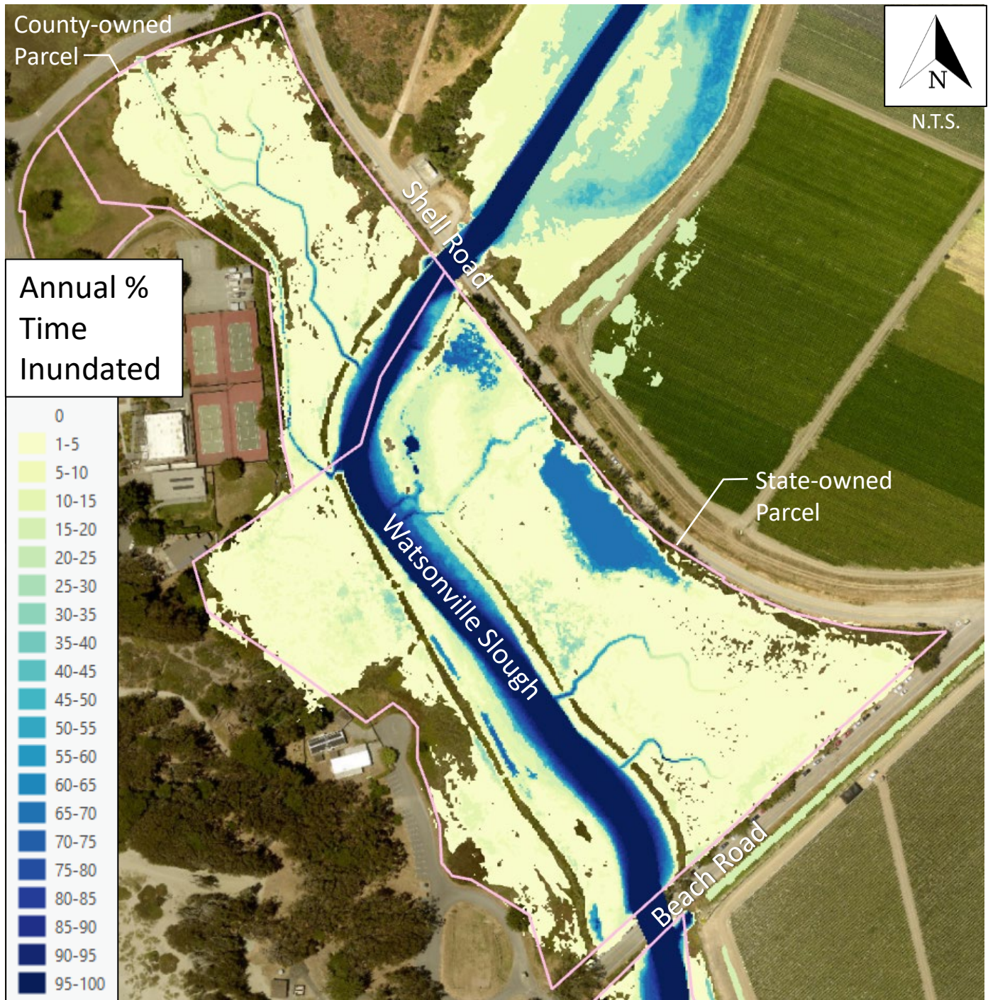
Figure 12: Annual PTI – State and County Parcels; Year 50; Crossing Improvements + Earthwork
