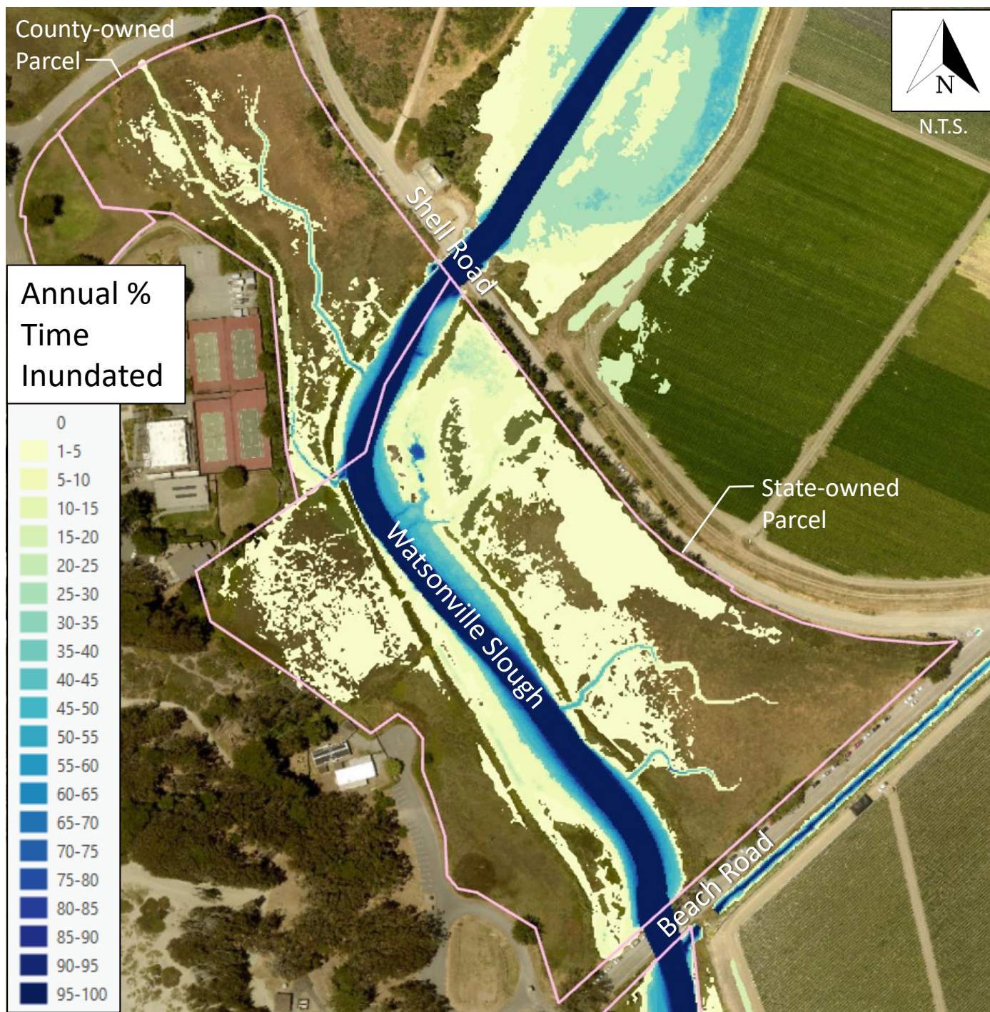
Figure 3: Annual PTI – State and County Parcels; Year 0; Earthwork
