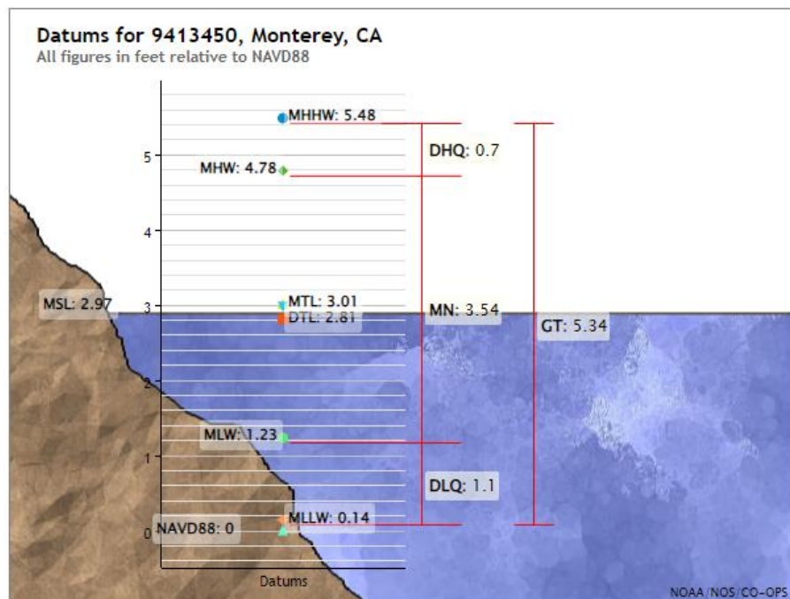
Figure 48: Tidal datums for NOAA Monterey tide station (#9413450).
