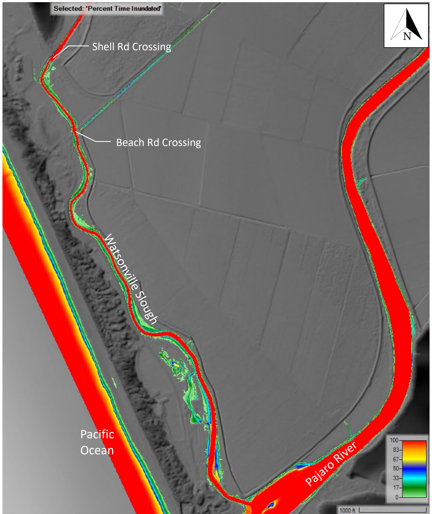
Figure 1: Percent time inundated – No Action; Year 0; Open Lagoon, Dry Season
