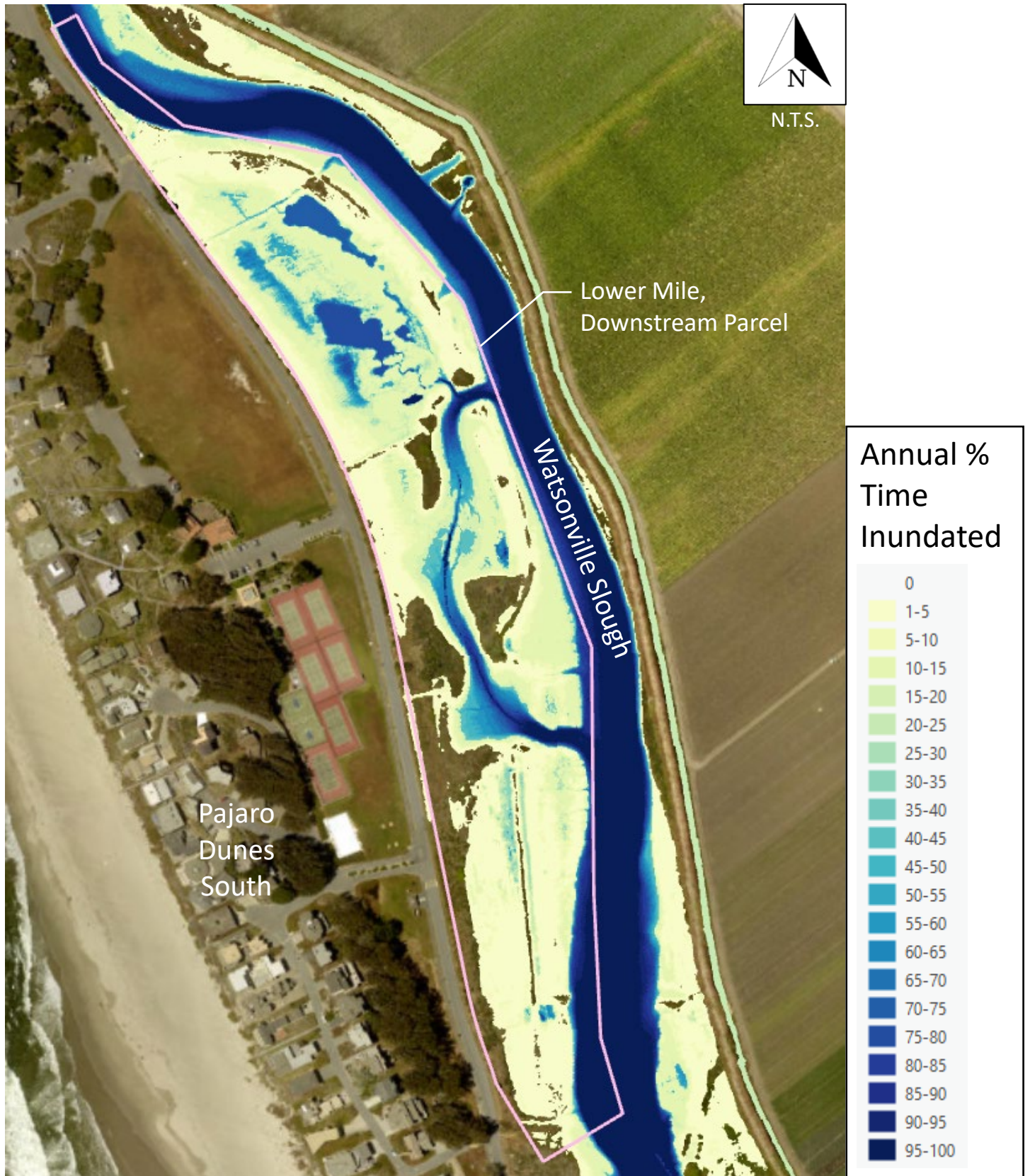
Figure 30: Annual PTI – Lower Mile, Downstream Parcel; Year 25; Crossing Improvements
