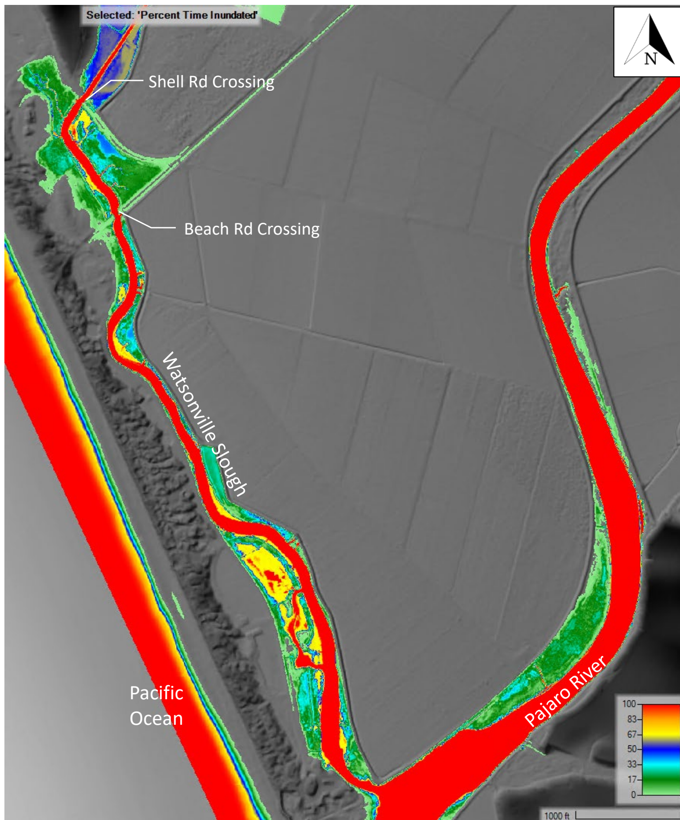
Figure 30: Percent time inundated – Crossing Improvements + Earthwork; Year 0; Closed Lagoon, Wet Season
