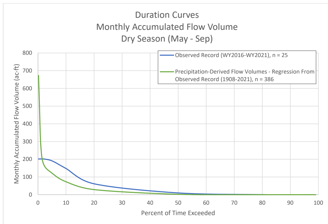
Figure 12: Duration curves for monthly accumulated flow volume in Watsonville Slough during the dry season.
