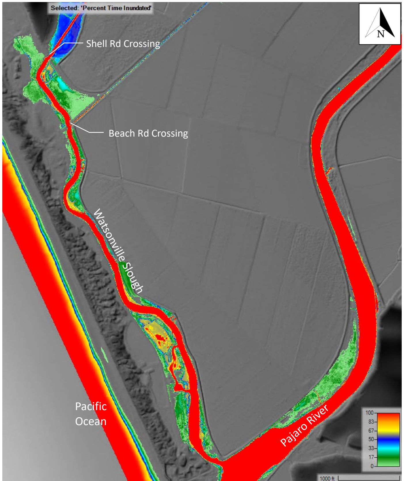
Figure 3: Percent time inundated – No Action; Year 0; Closed Lagoon, Wet Season
