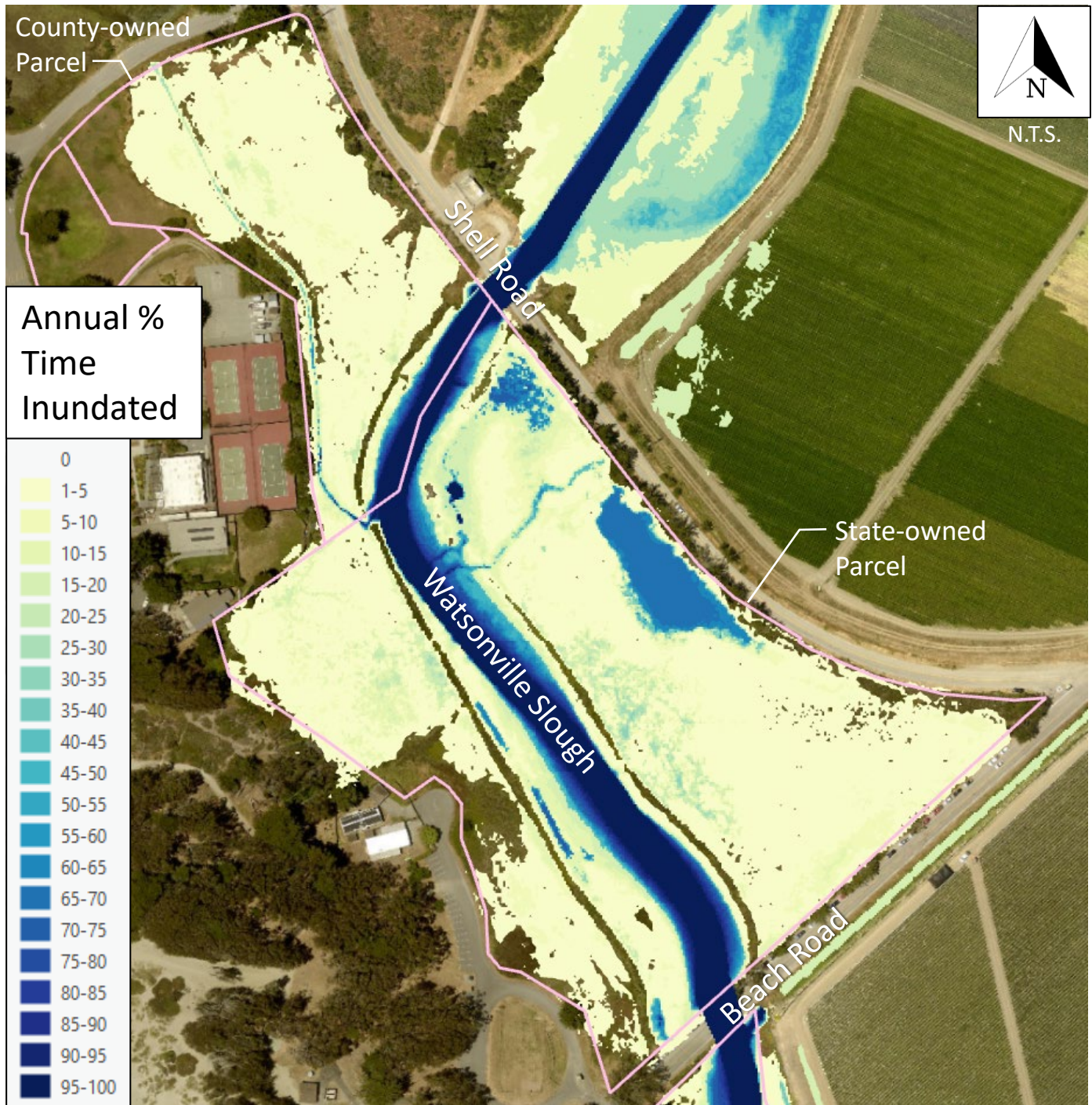
Figure 10: Annual PTI – State and County Parcels; Year 50; Crossing Improvements
