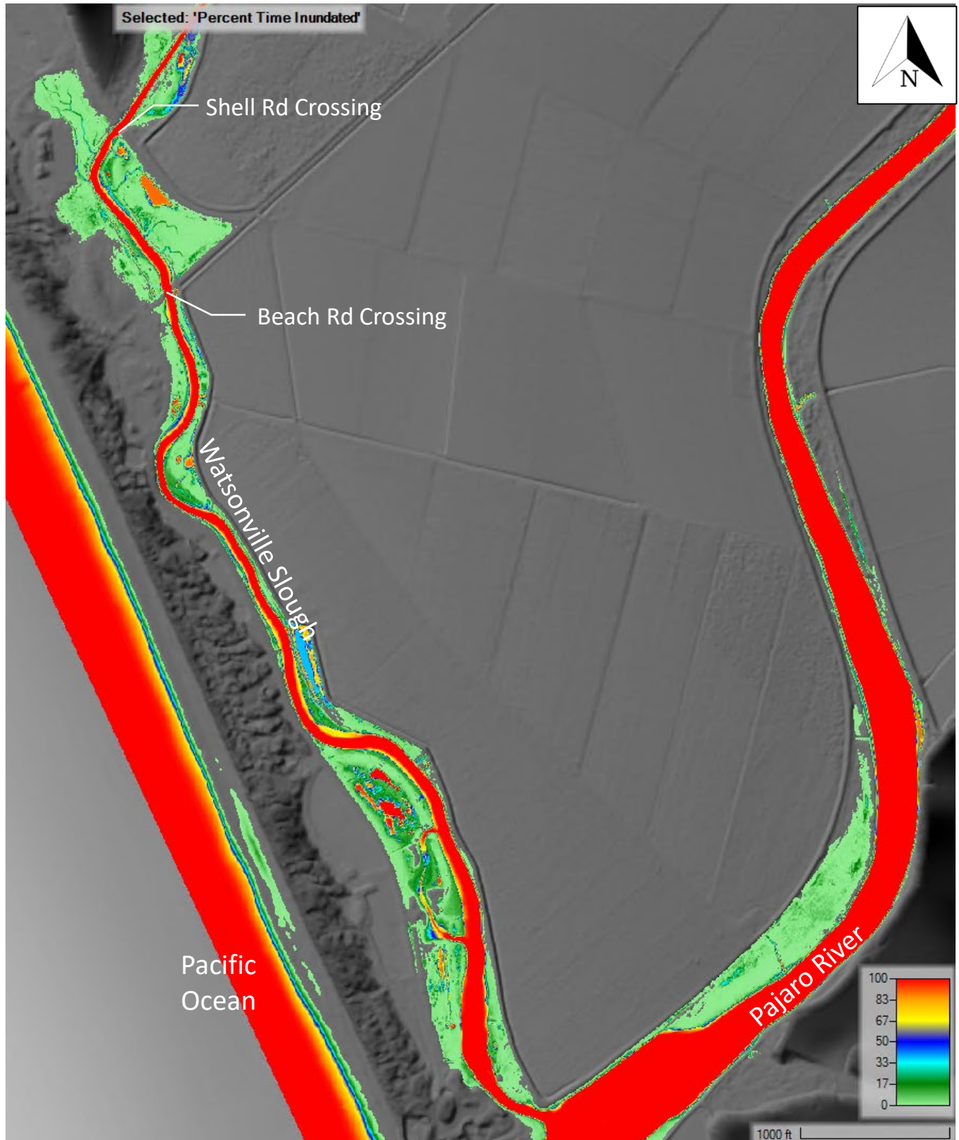
Figure 35: Percent time inundated – Crossing Improvements + Earthwork; Year 50; Open Lagoon, Wet Season
