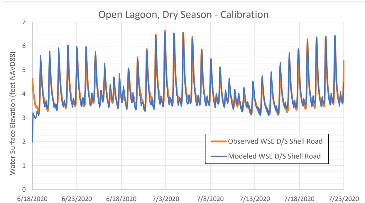
Figure 21: Observed vs. Modeled water surface elevation downstream of Shell Road for Open Lagoon model for June to July 2020.
