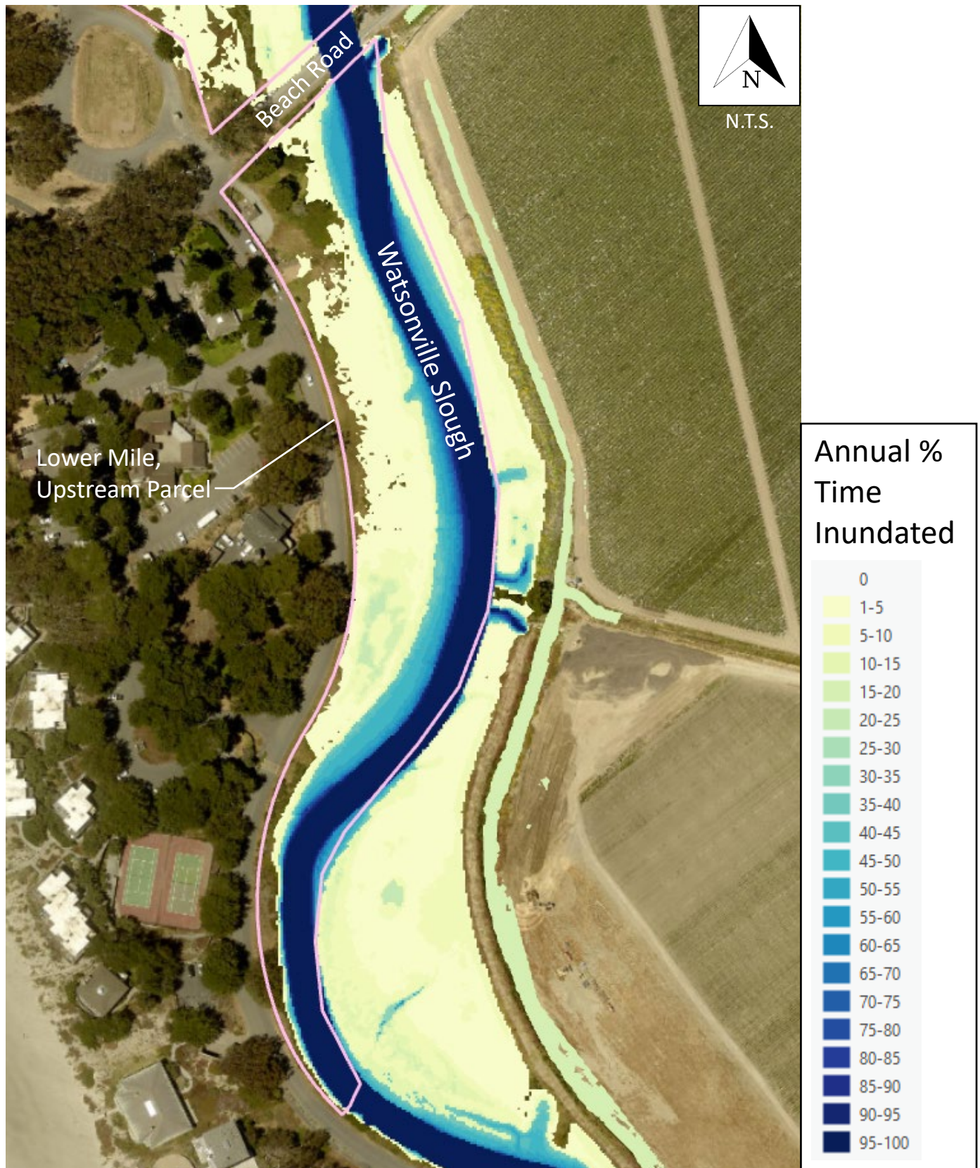
Figure 16: Annual PTI – Lower Mile, Upstream Parcel; Year 0; Crossing Improvements + Earthwork
