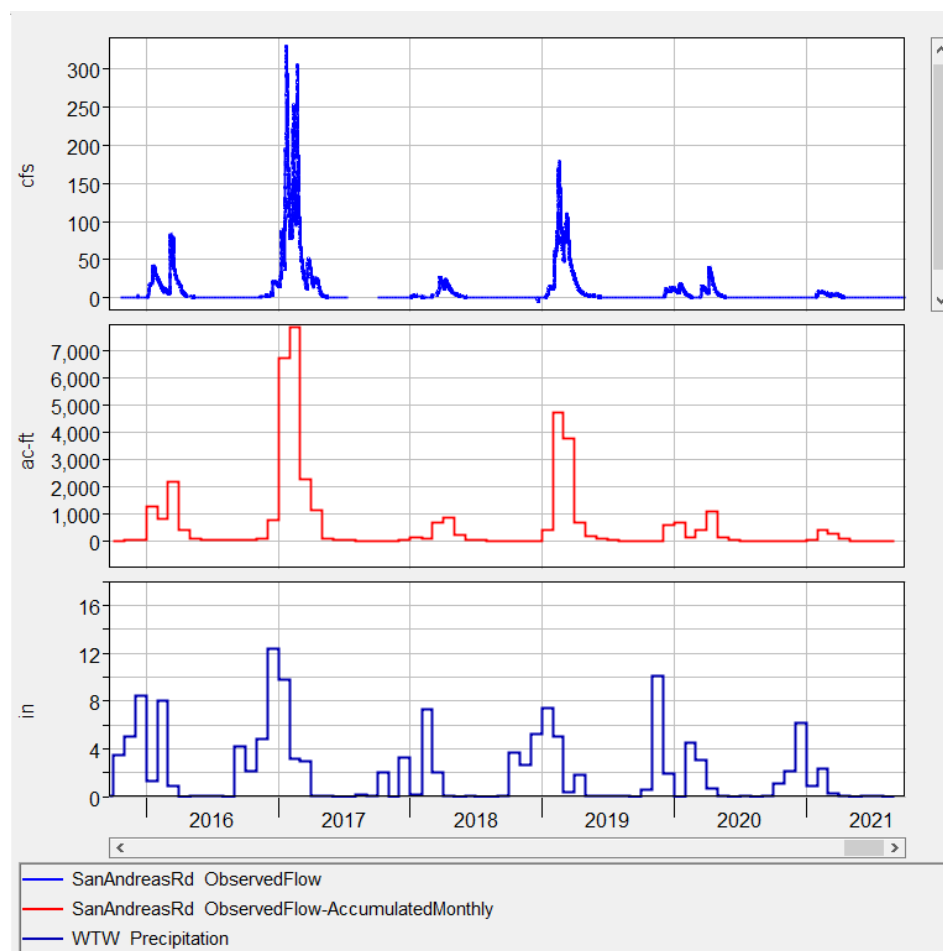
Figure 8: 15-minute flow values (blue) and monthly accumulated flow volumes (red) for the observed flow record from the PV Water gage located at San Andreas Road, compared to monthly precipitation (navy) at Watsonville Waterworks rain gage.
