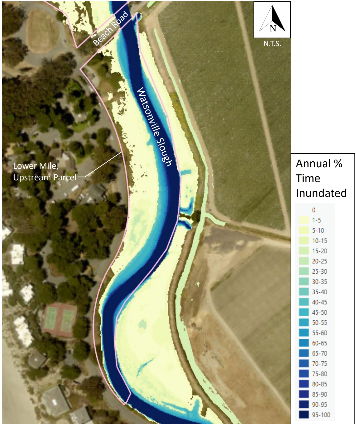
Figure 14: Annual PTI – Lower Mile, Upstream Parcel; Year 0; Crossing Improvements
