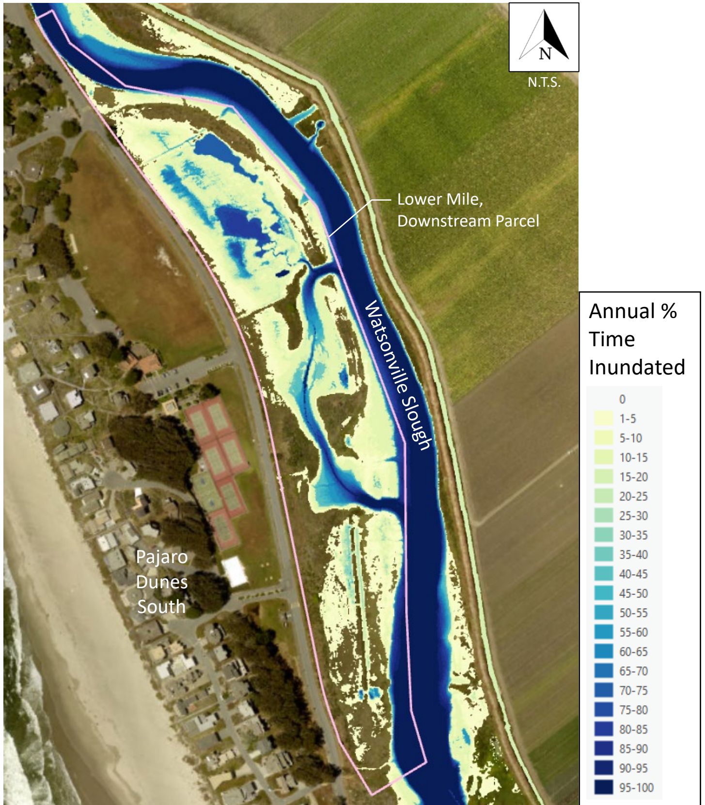
Figure 31: Annual PTI – Lower Mile, Downstream Parcel; Year 25; Earthwork
