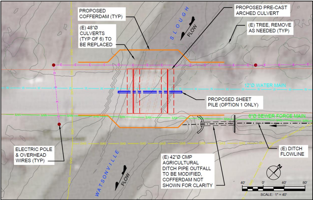
Figure 10 Culvert Replacement Plan - Option 1
