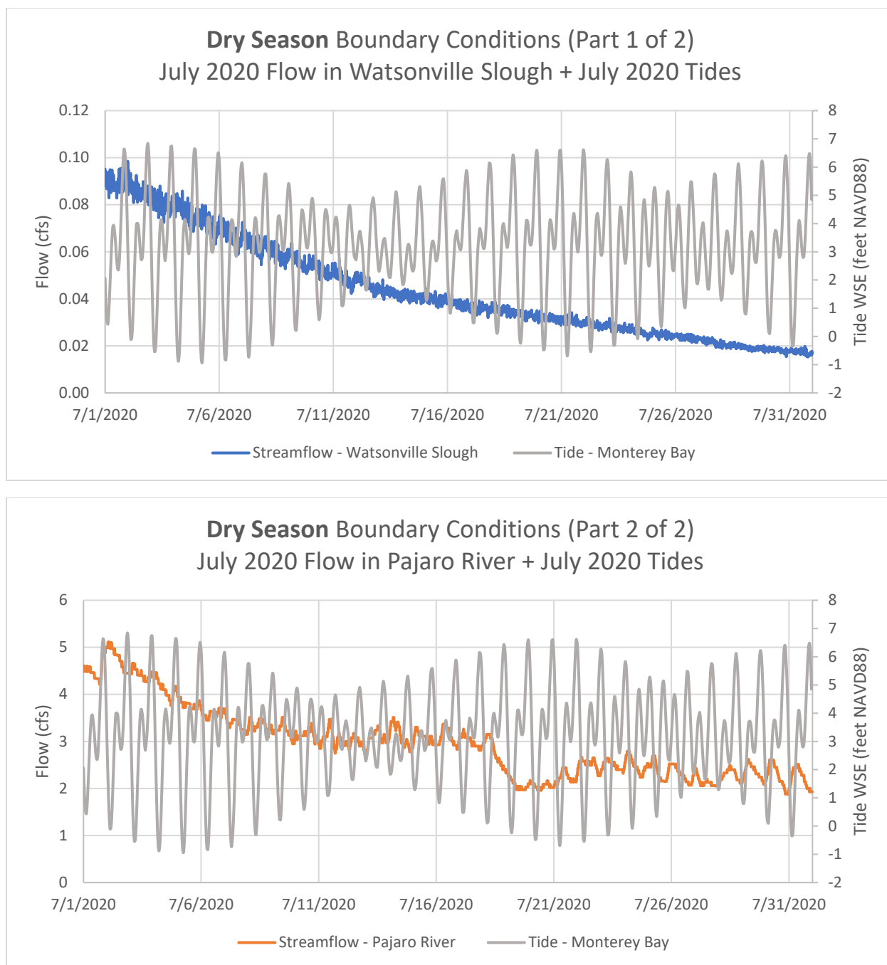
Figure 19: Open lagoon, dry season boundary conditions.
