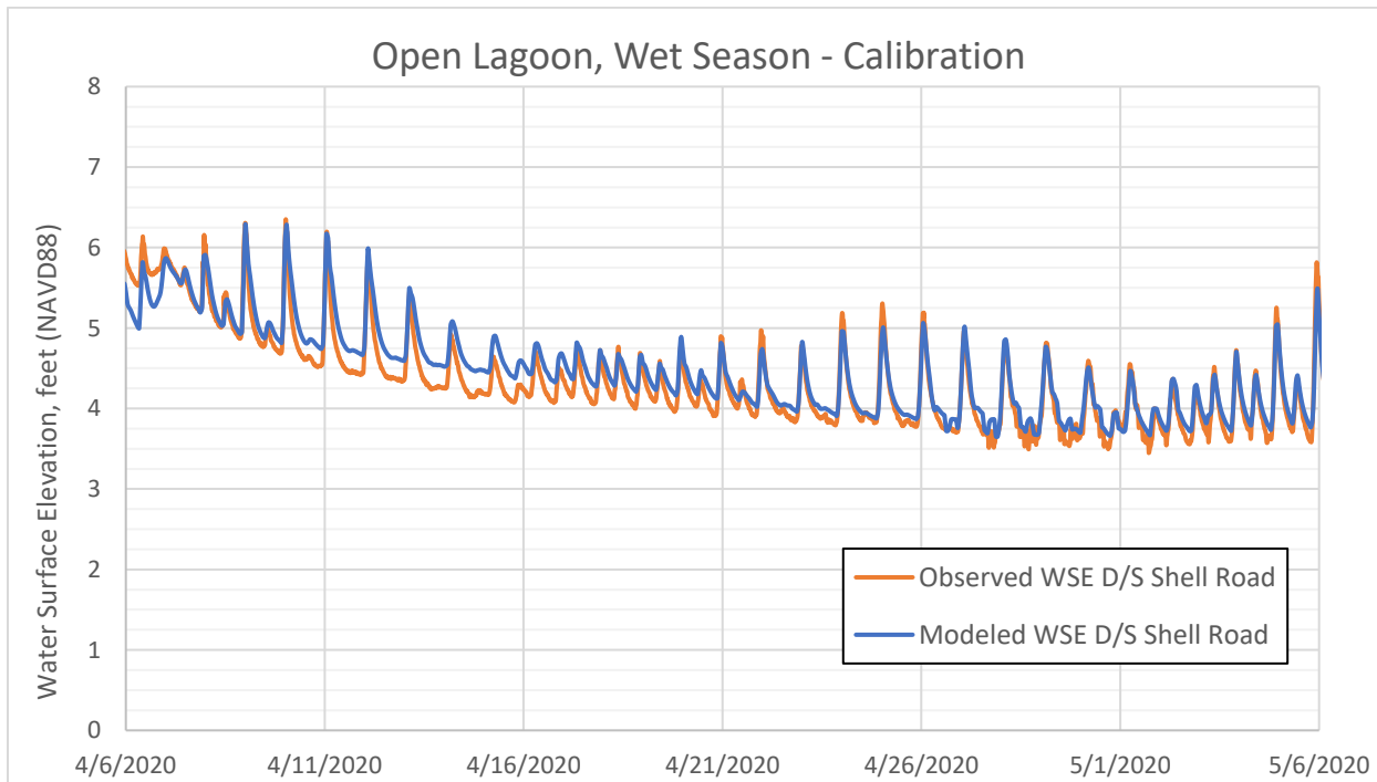
Figure 22: Observed vs. Modeled water surface elevation downstream of Shell Road for Open Lagoon model for April 2020.
