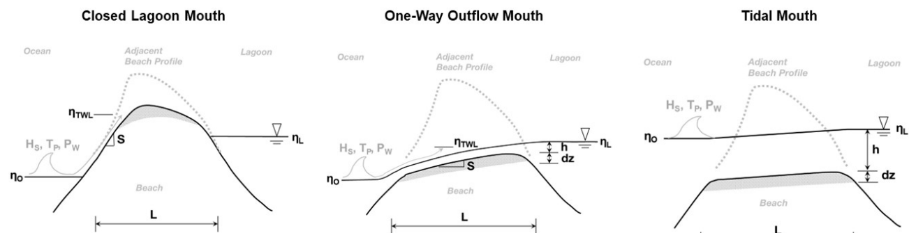
Figure 2a Schematic of water balance component of the QCM.
