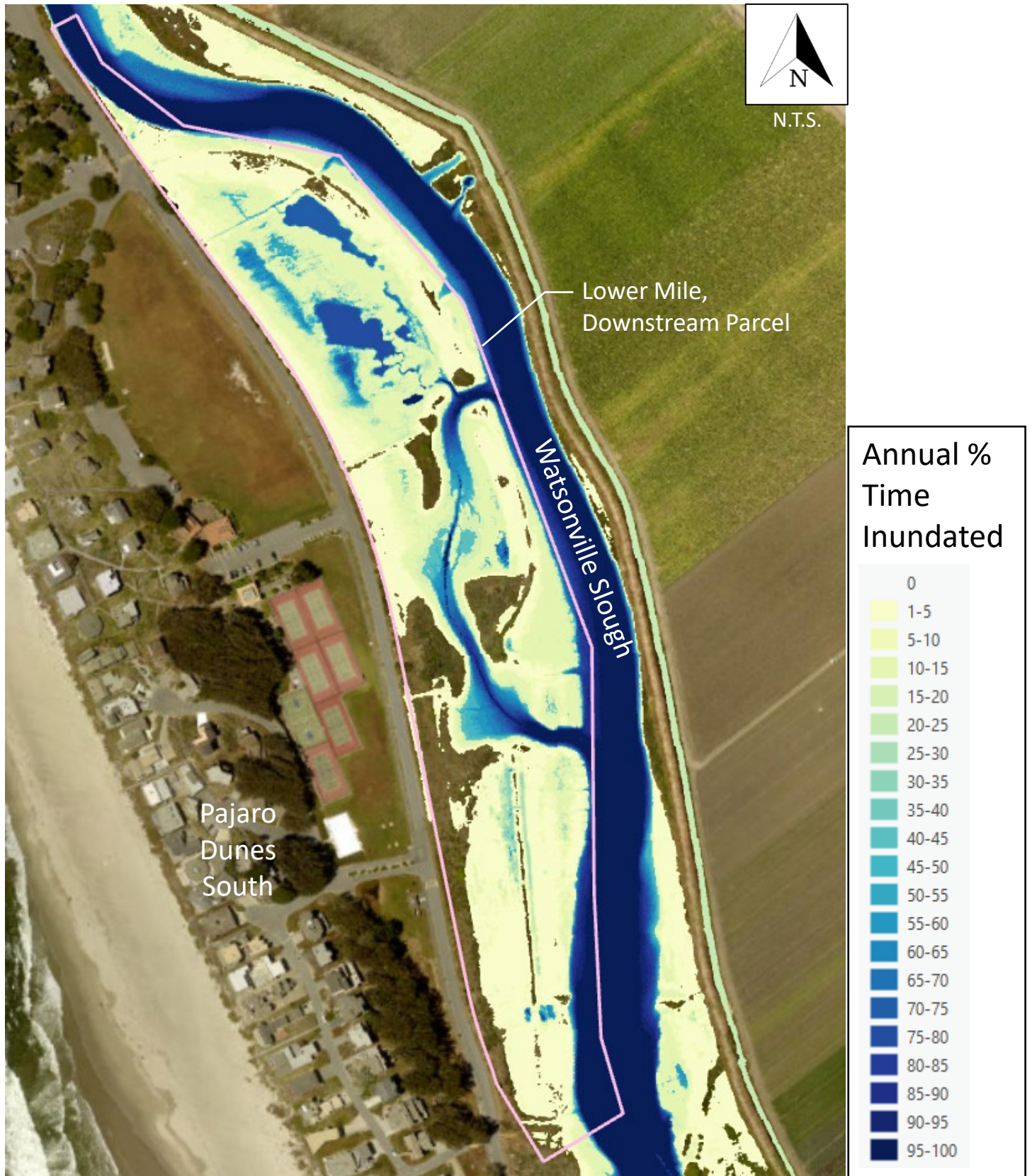
Figure 32: Annual PTI – Lower Mile, Downstream Parcel; Year 25; Crossing Improvements + Earthwork
