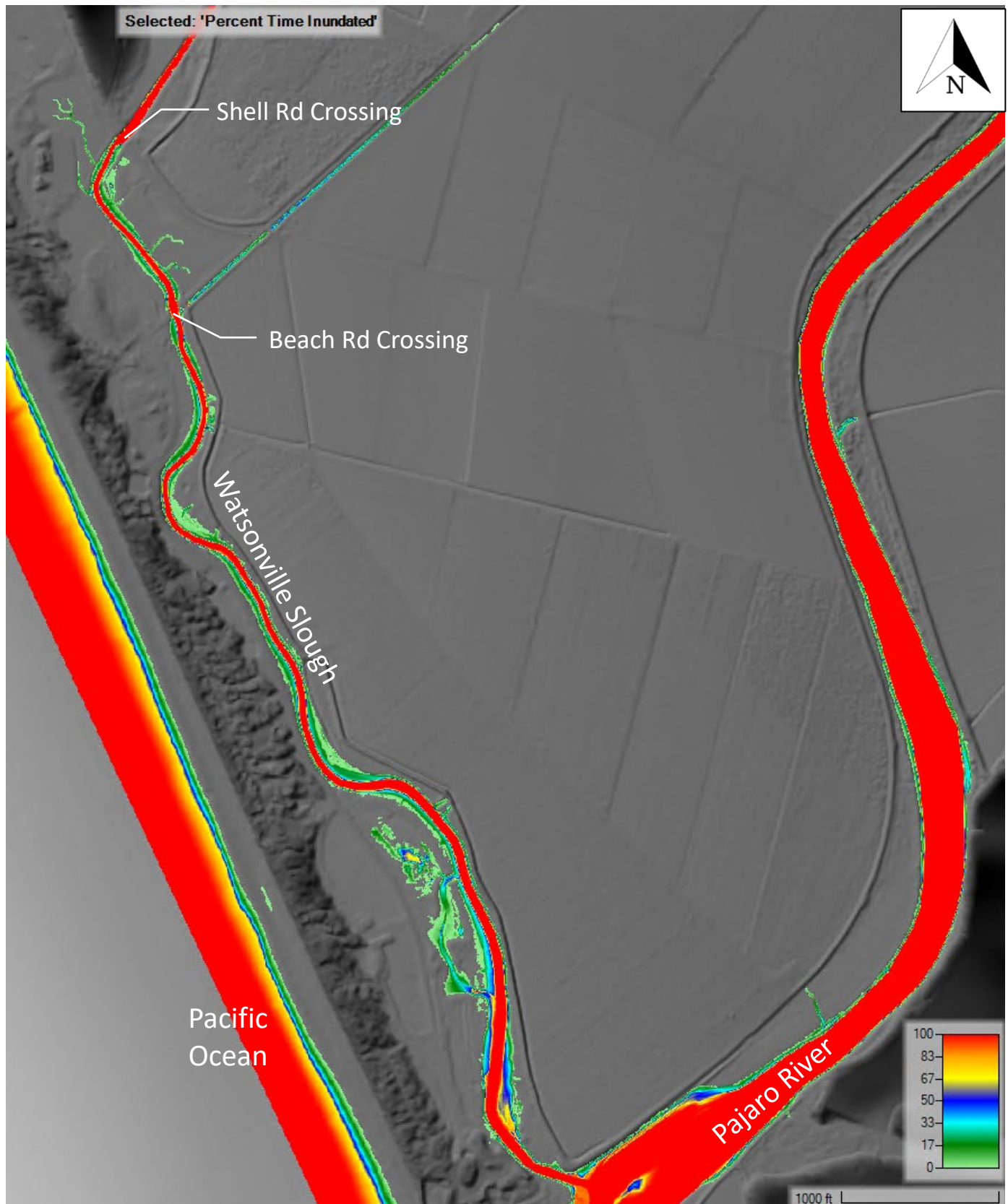
Figure 19: Percent time inundated – Earthwork; Year 0; Open Lagoon, Dry Season
