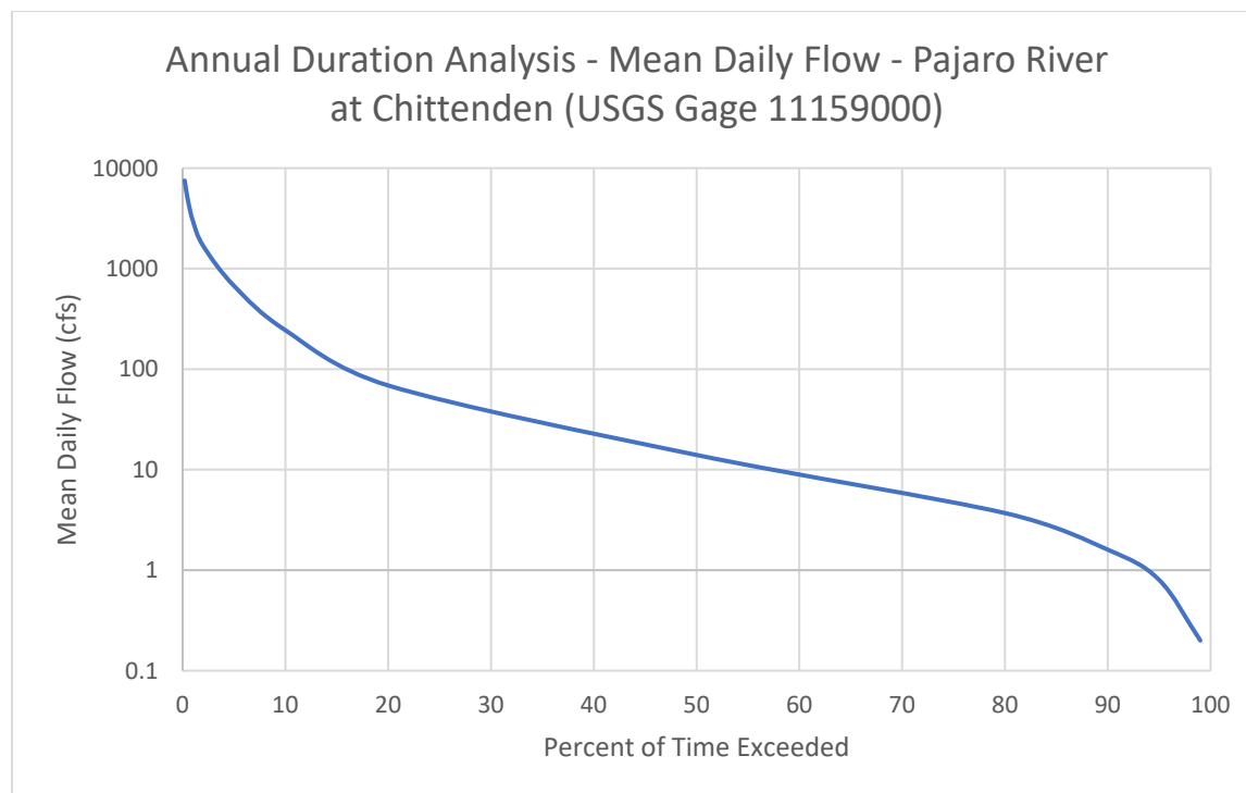
Figure 14: Duration curve for mean daily flow in Pajaro River at Chittenden.
