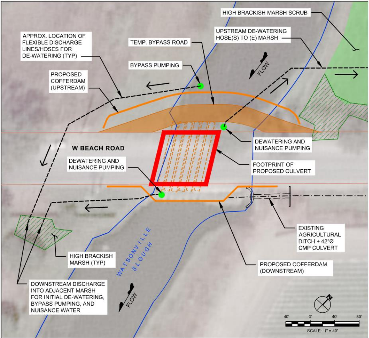
Figure 9 Dewatering Schematic (Enlarged)
