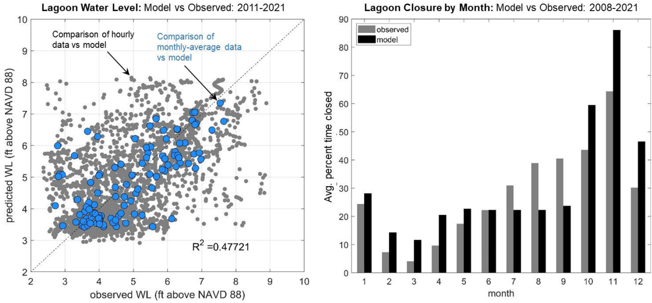
Figure 6 (left) Comparison of modeled and observed water levels in the lagoon and (right) comparison of modeled and observed % time of inlet closure by month of the year.
