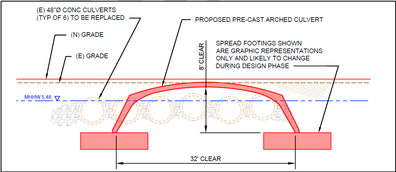
Figure 11 Culvert Replacement Elevation
