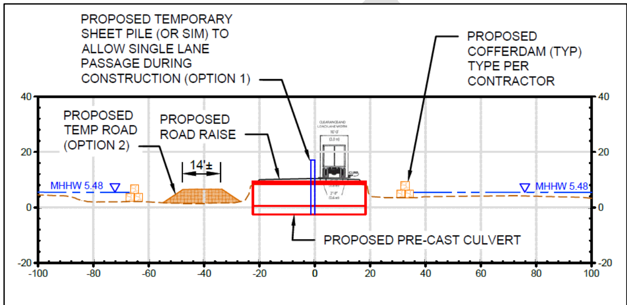
Figure 13 Road Section A (During Construction)
