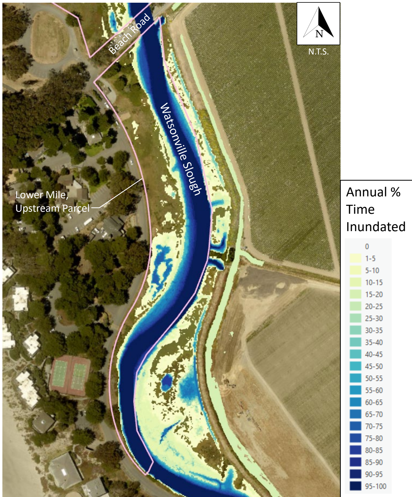
Figure 23: Annual PTI – Lower Mile, Upstream Parcel; Year 50; Earthwork
