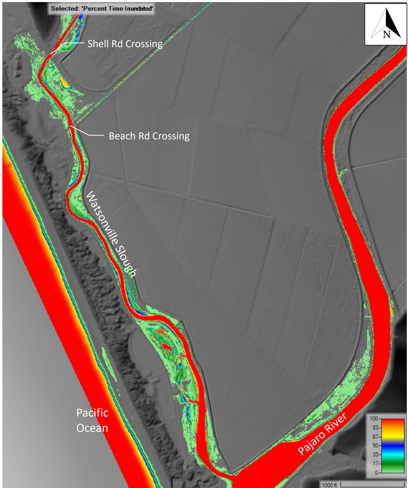
Figure 23: Percent time inundated – Earthwork; Year 25; Open Lagoon, Wet Season
