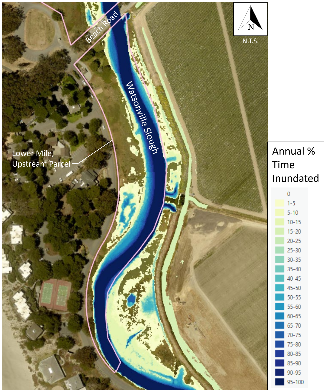
Figure 17: Annual PTI – Lower Mile, Upstream Parcel; Year 25; No Action
