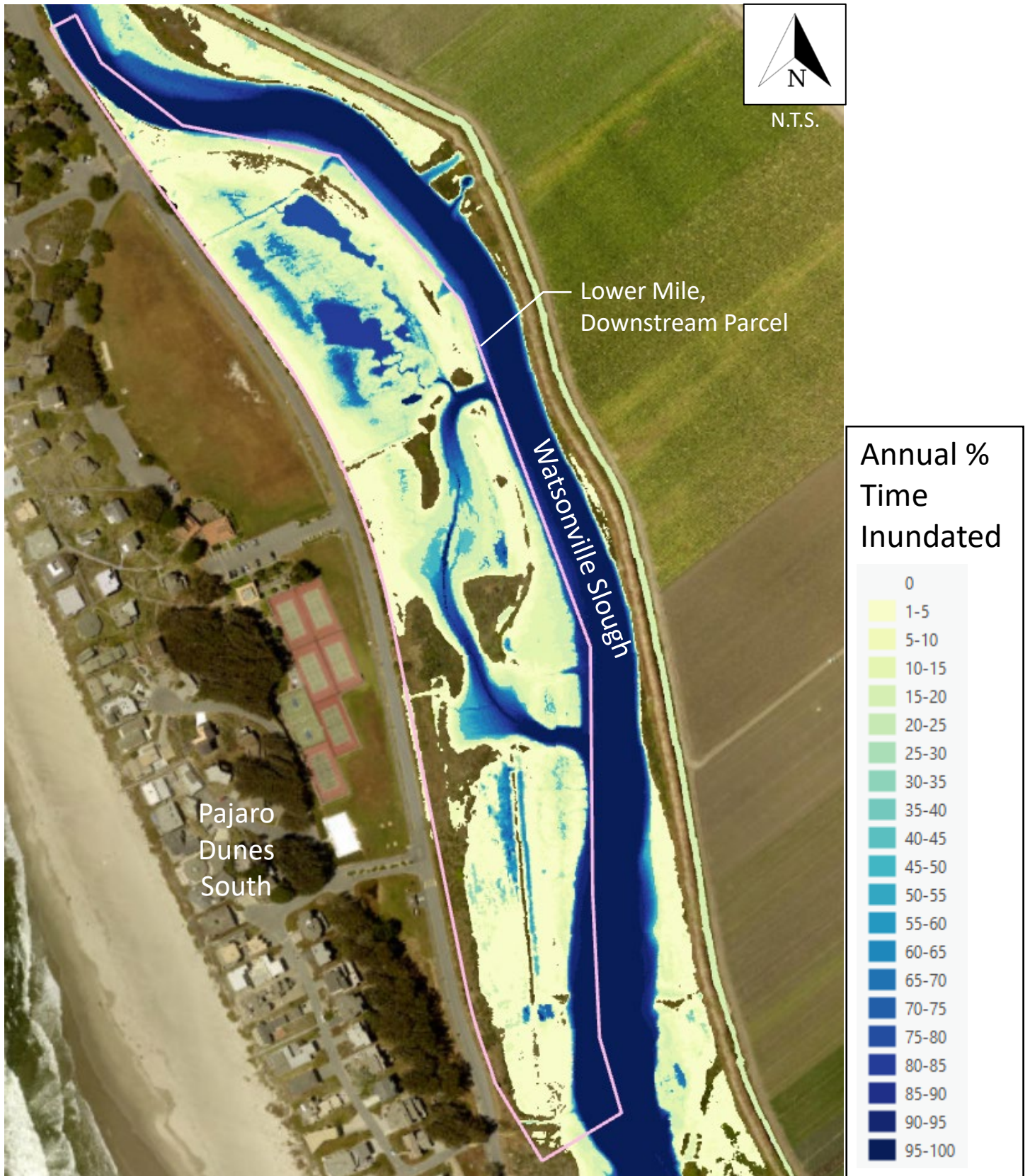
Figure 34: Annual PTI – Lower Mile, Downstream Parcel; Year 50; Crossing Improvements
