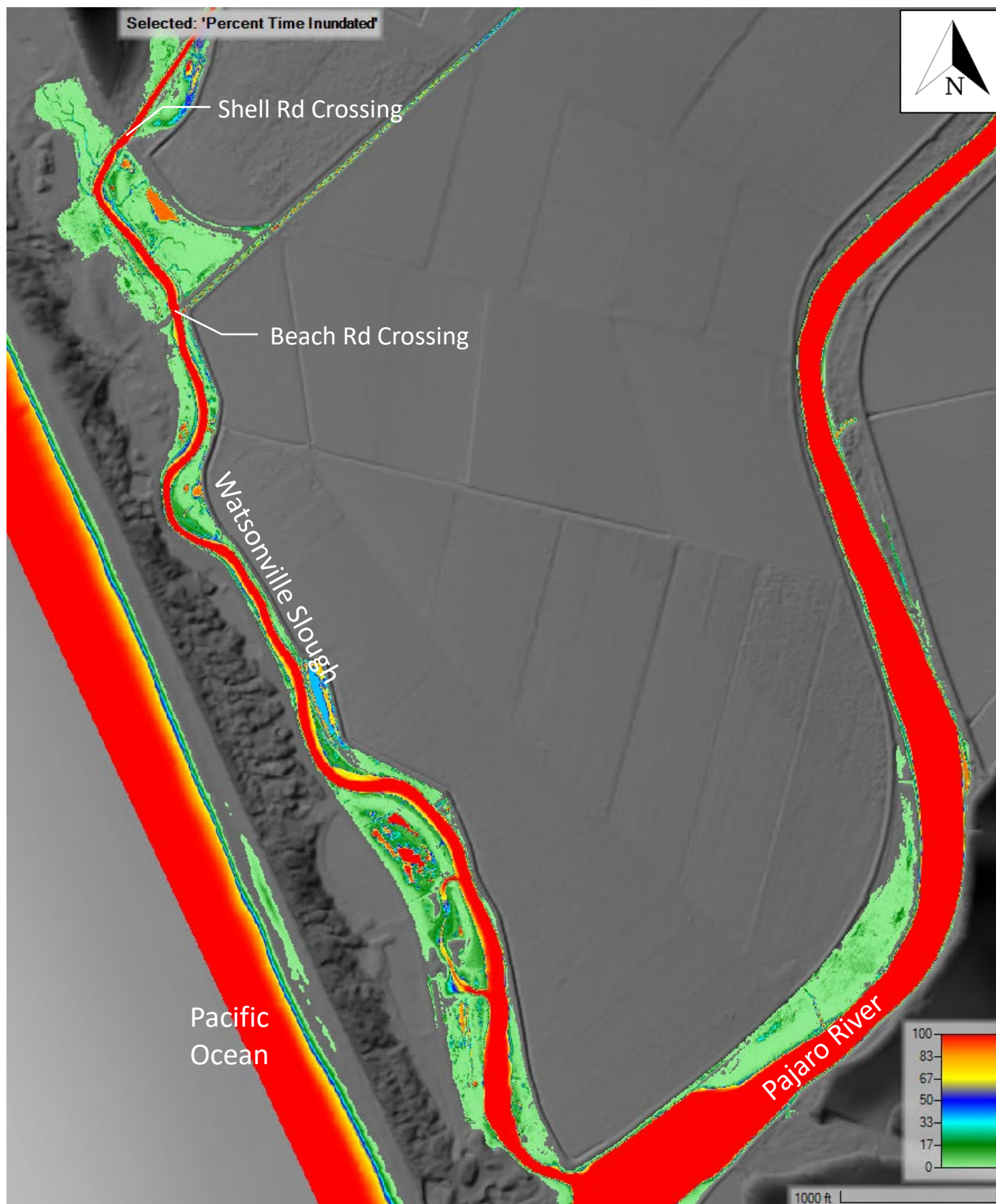
Figure 26: Percent time inundated – Earthwork; Year 50; Open Lagoon, Wet Season
