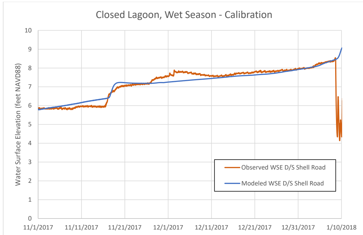
Figure 23: Observed vs. Modeled water surface elevation downstream of Shell Road for Closed Lagoon model for November 2017 to January 2018 closure event.
