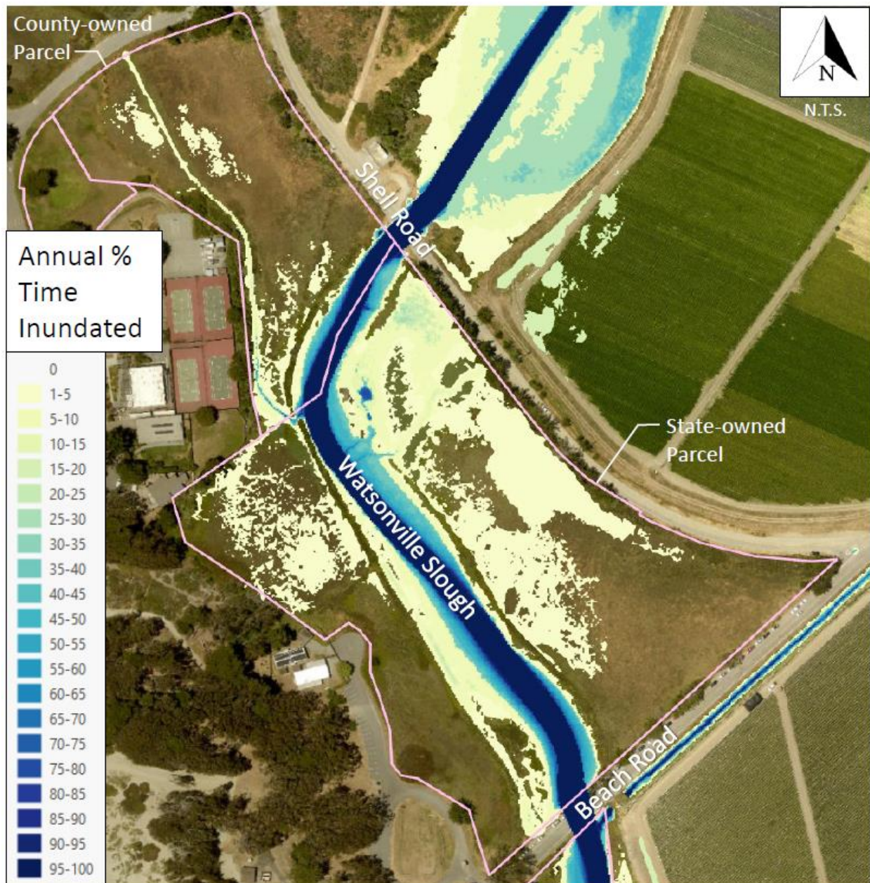
Figure 28: Annual percent time inundated for No Action, Project Year 0.
