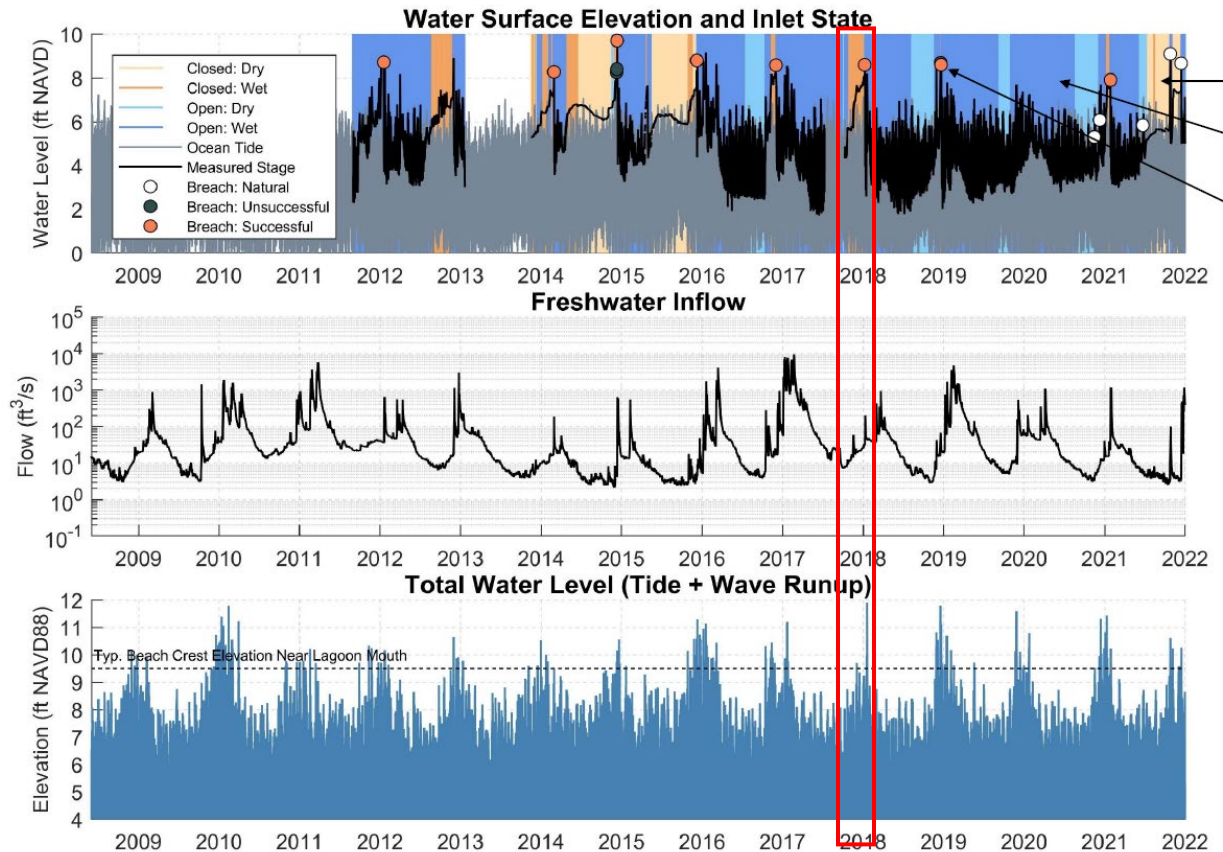
Figure 21: Historical record of water levels in Pajaro Lagoon, freshwater inflow into the lagoon, and total water level in Monterey Bay, with lagoon closure state and breach events indicated. The red box highlights the closure period that was selected for hydraulic modeling for the Watsonville CAP feasibility study. Figure adapted from preliminary results provided by ESA.
