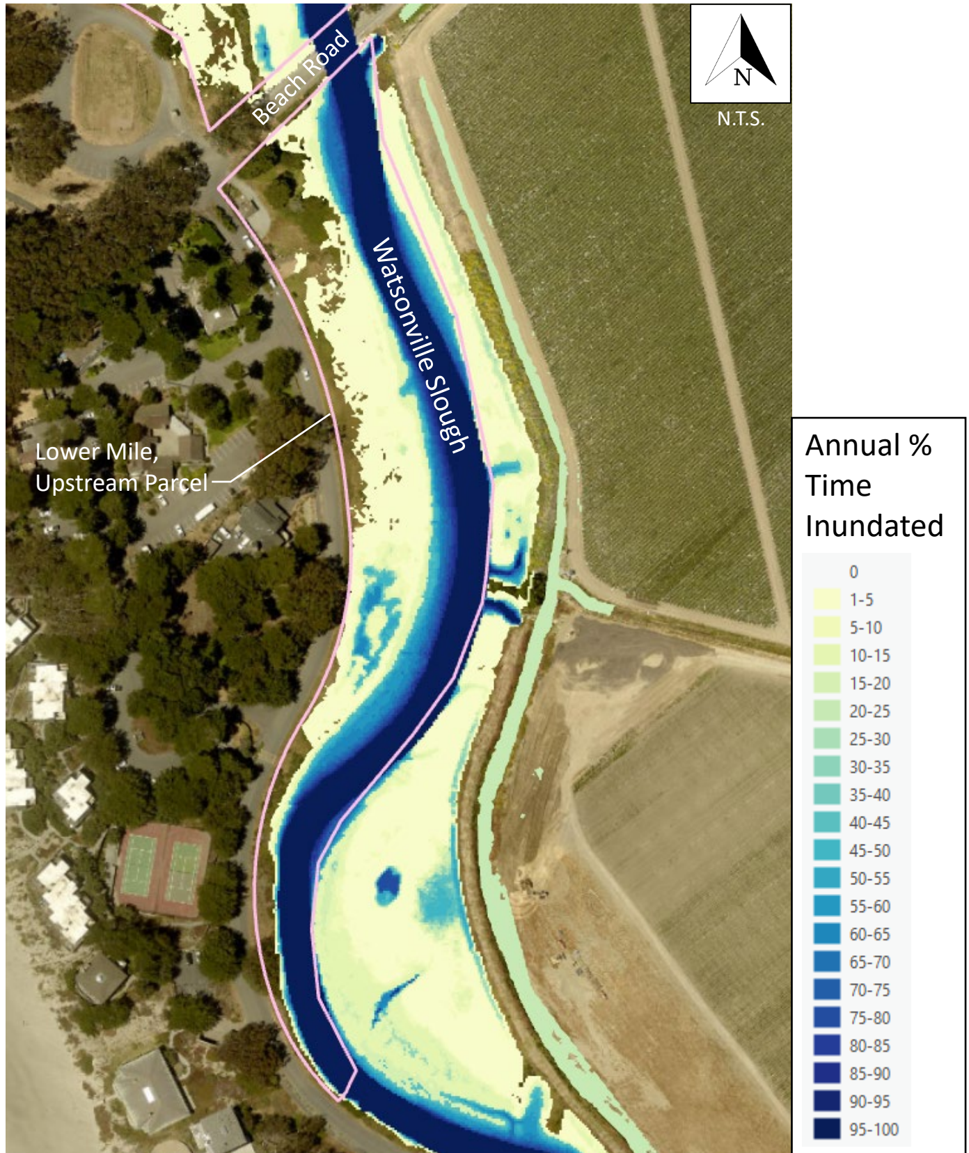
Figure 18: Annual PTI – Lower Mile, Upstream Parcel; Year 25; Crossing Improvements
