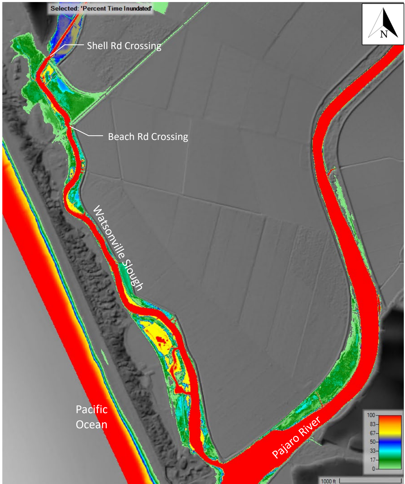
Figure 15: Percent time inundated – Crossing Improvements; Year 25; Closed Lagoon, Wet Season
