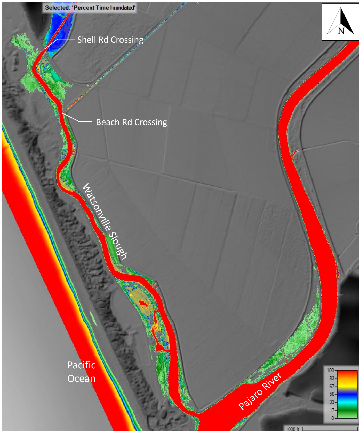
Figure 9: Percent time inundated – No Action; Year 50; Closed Lagoon, Wet Season
