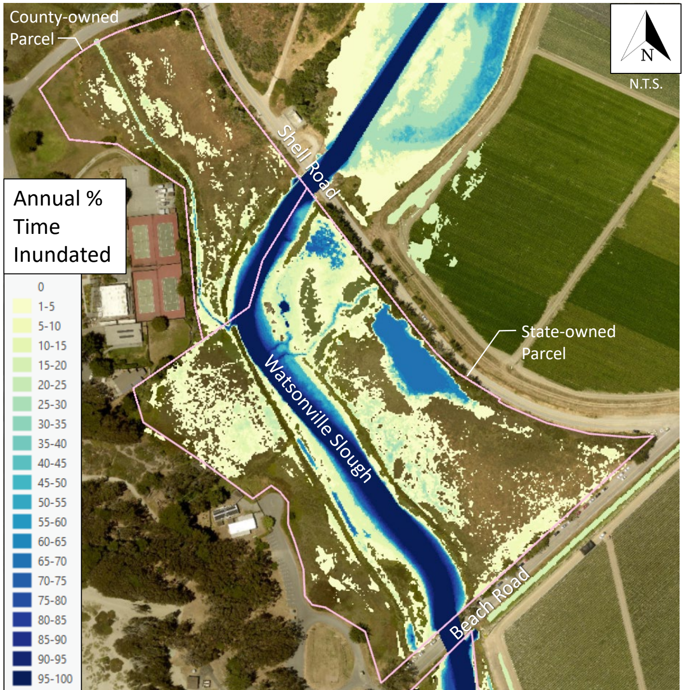
Figure 9: Annual PTI – State and County Parcels; Year 50; No Action
