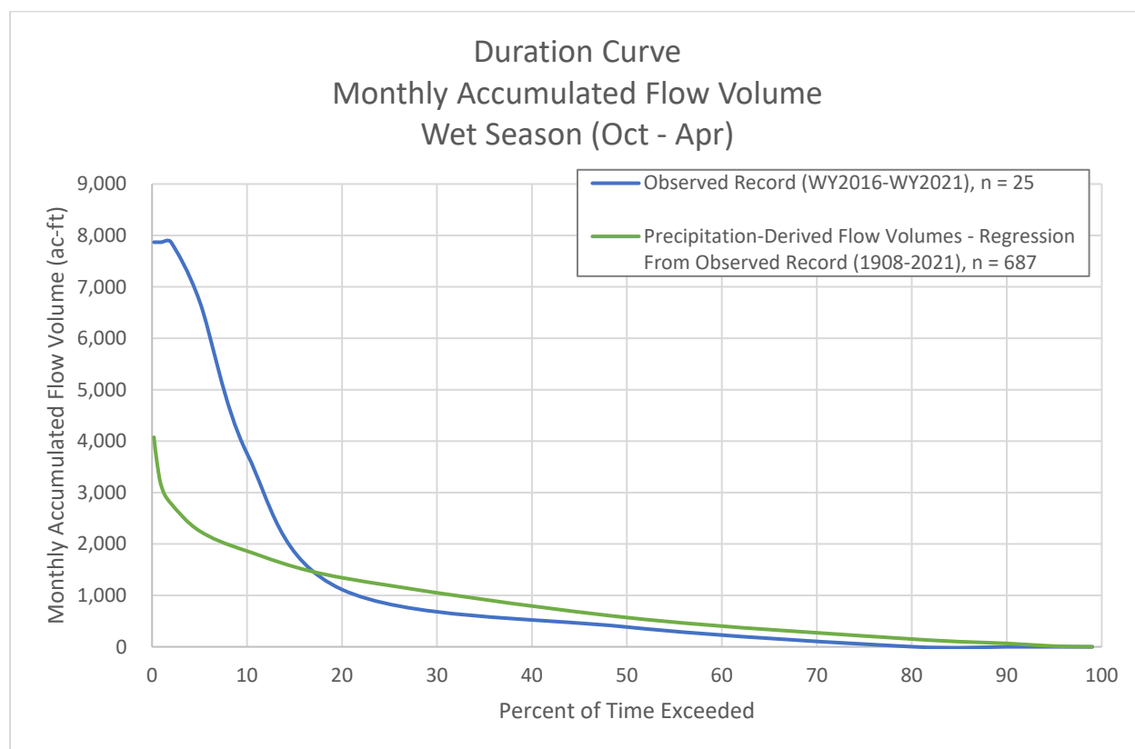
Figure 13: Duration curves for monthly accumulated flow volume in Watsonville Slough during the wet season.
