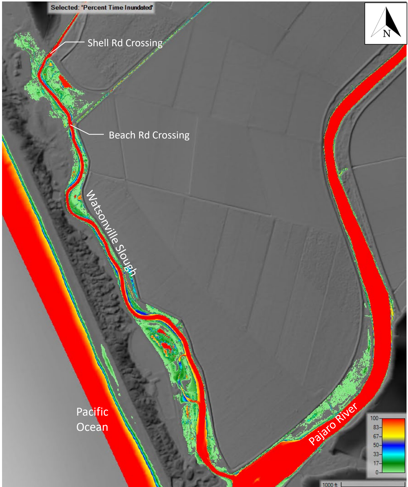
Figure 25: Percent time inundated – Earthwork; Year 50; Open Lagoon, Dry Season
