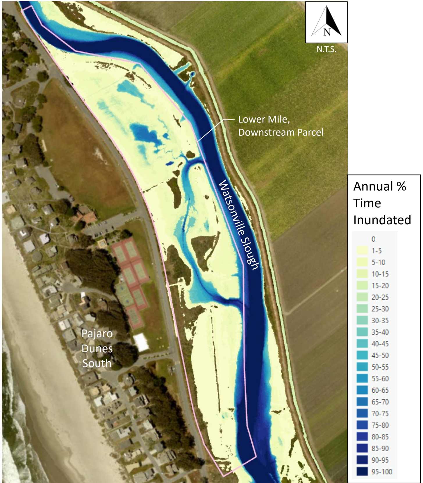
Figure 26: Annual PTI – Lower Mile, Downstream Parcel; Year 0; Crossing Improvements
