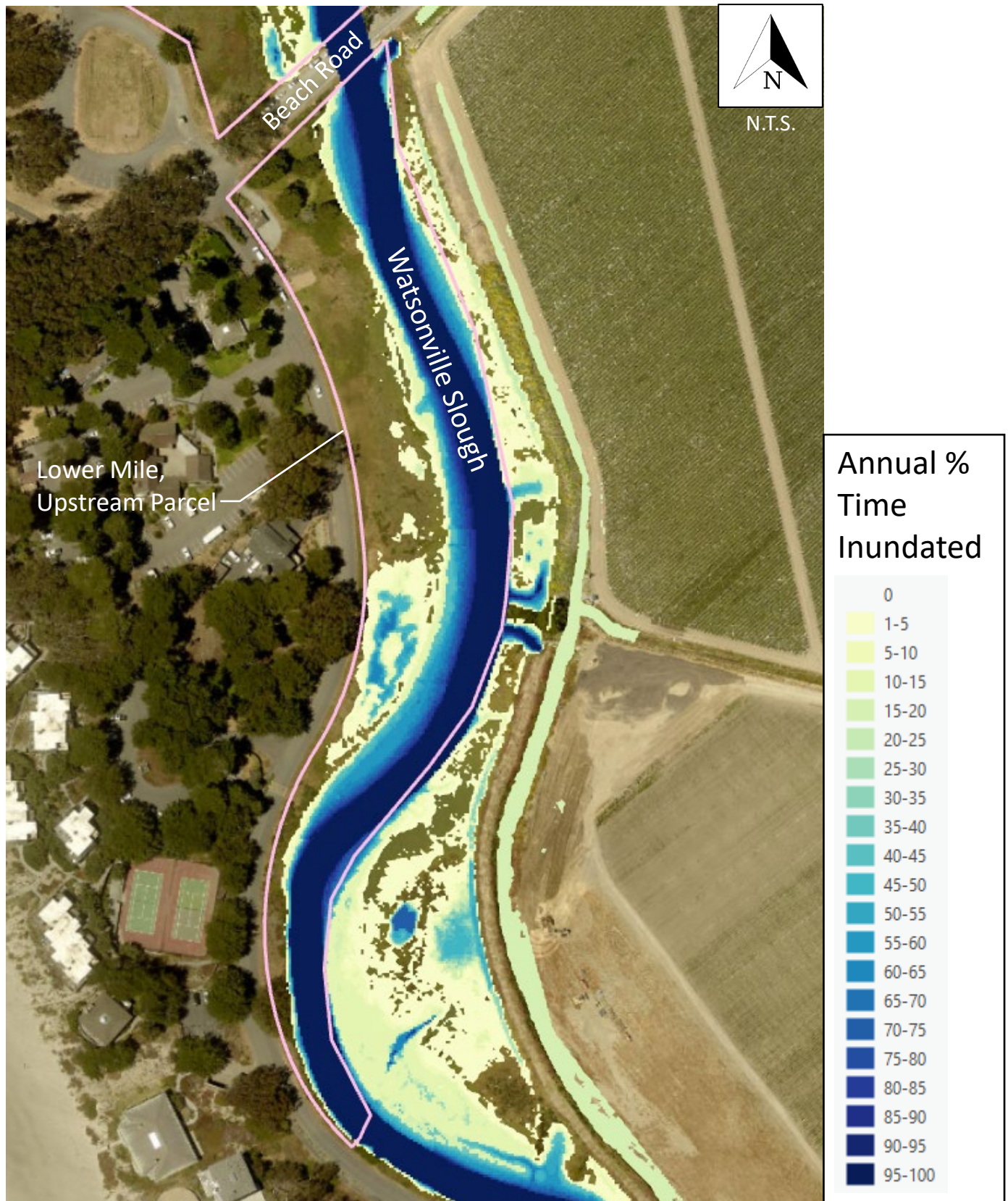
Figure 19: Annual PTI – Lower Mile, Upstream Parcel; Year 25; Earthwork
