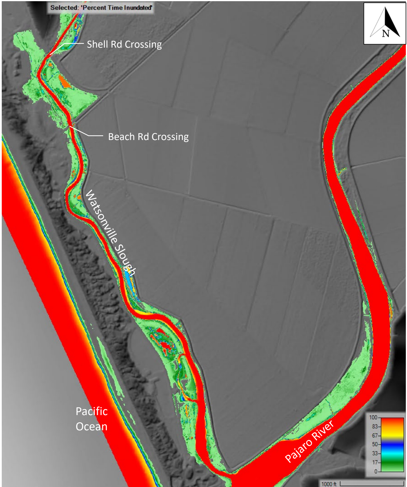
Figure 17: Percent time inundated – Crossing Improvements; Year 50; Open Lagoon, Wet Season
