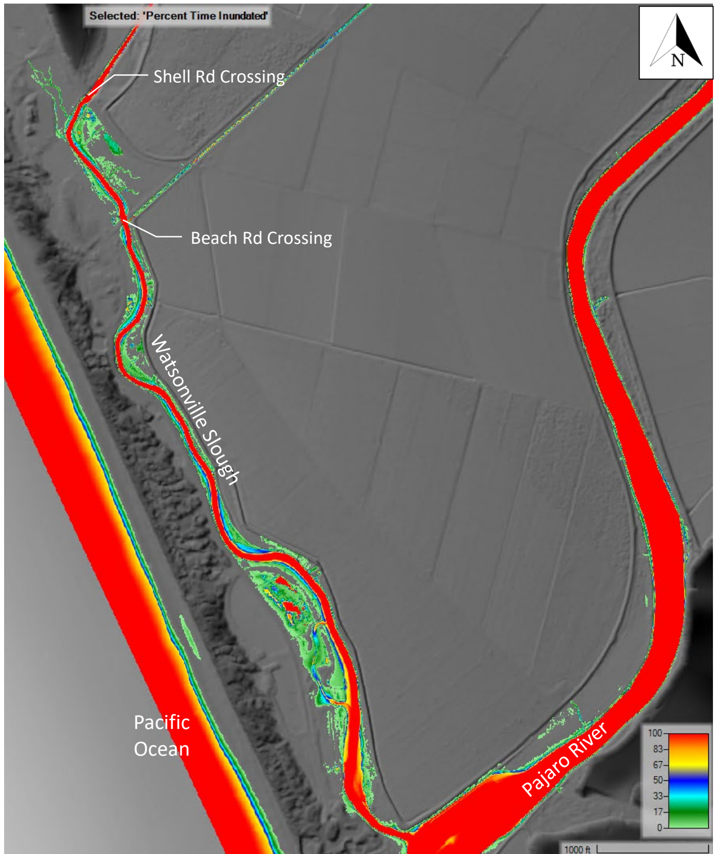
Figure 22: Percent time inundated – Earthwork; Year 25; Open Lagoon, Dry Season
