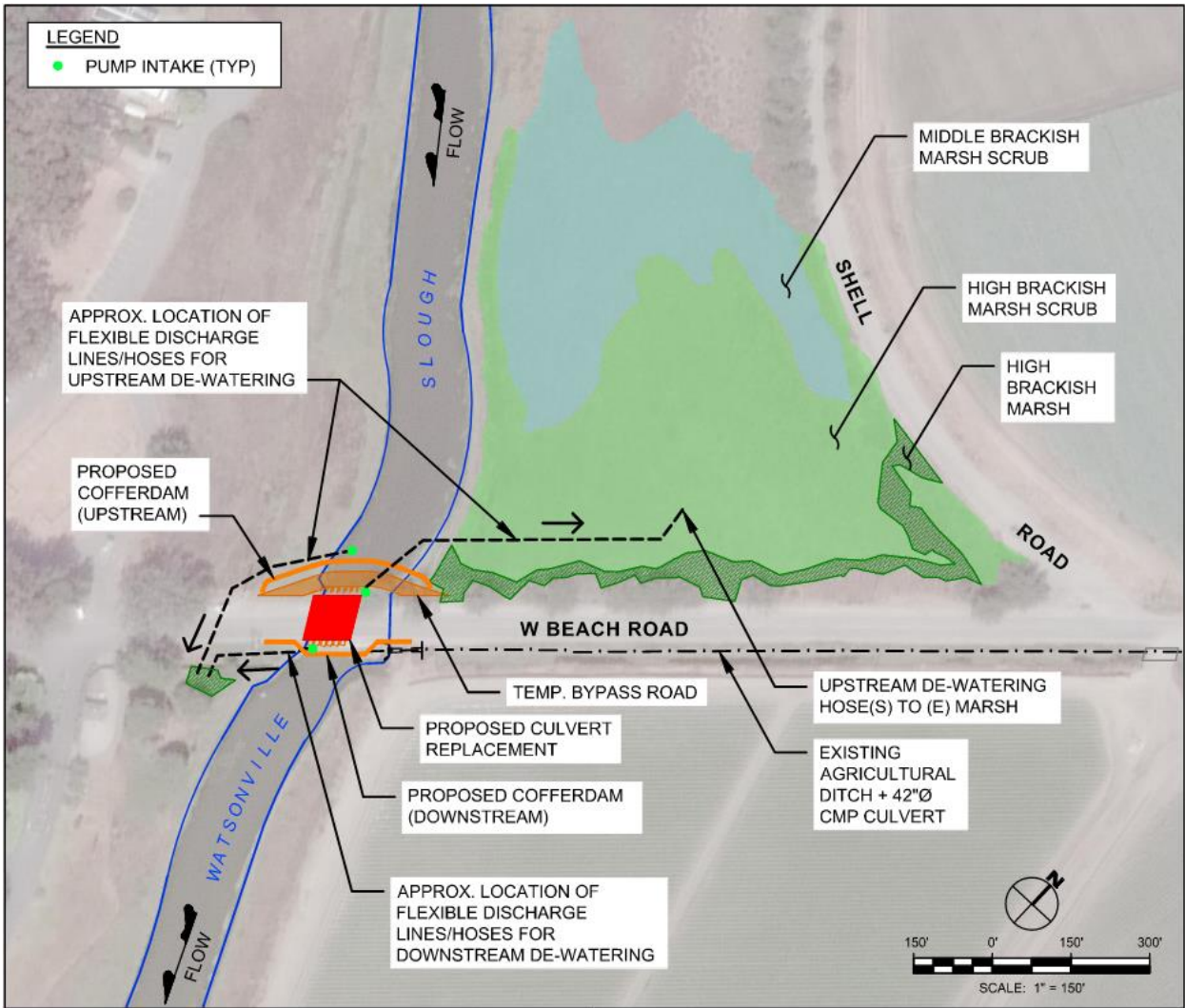
Figure 8 Dewatering Schematic
