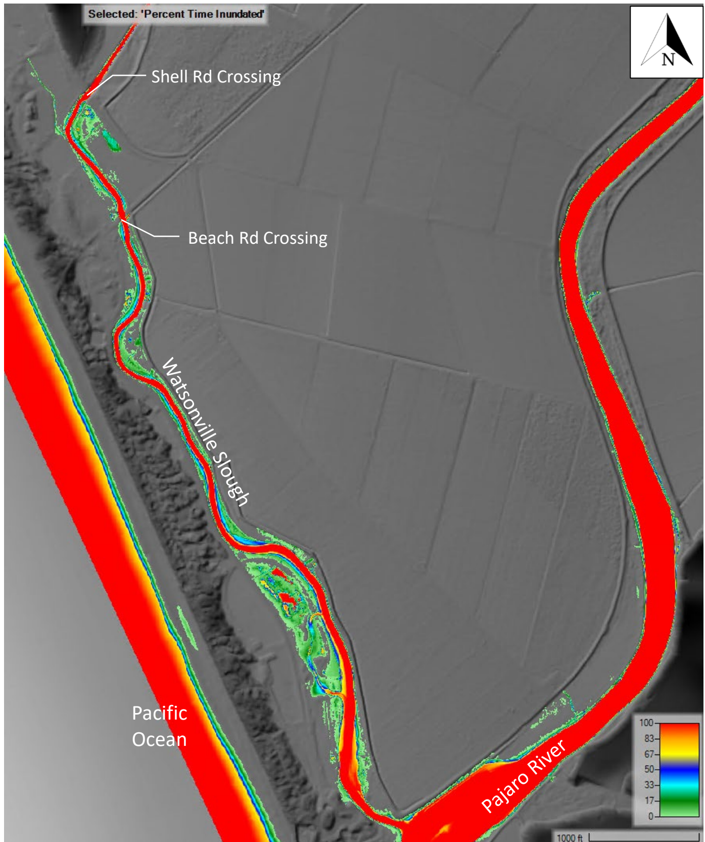
Figure 13: Percent time inundated – Crossing Improvements; Year 25; Open Lagoon, Dry Season
