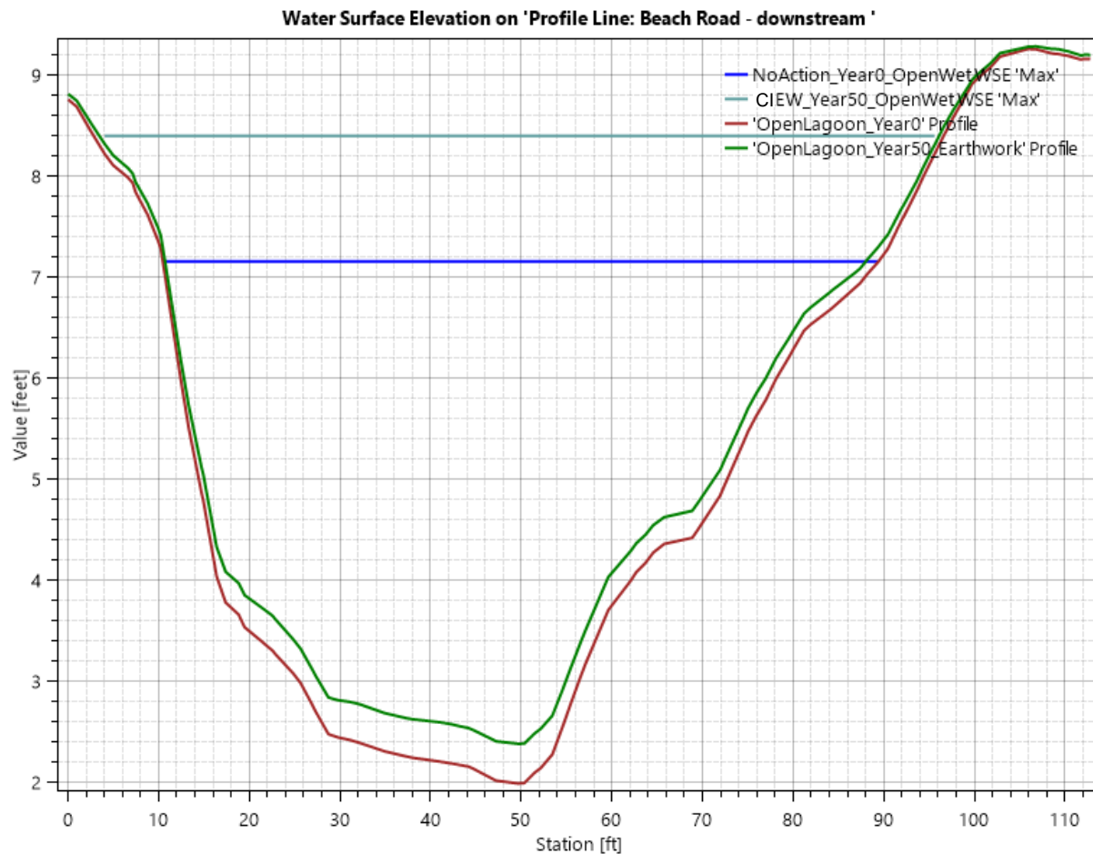
Figure 27: Cross section of terrain and maximum computed WSE immediately downstream of the Beach Road crossing for Simulation 2 (No Action; Year 0; Open Lagoon, Wet Season) and Simulation 46 (Crossing Improvements + Earthwork; Year 50; Open Lagoon, Wet Season).
