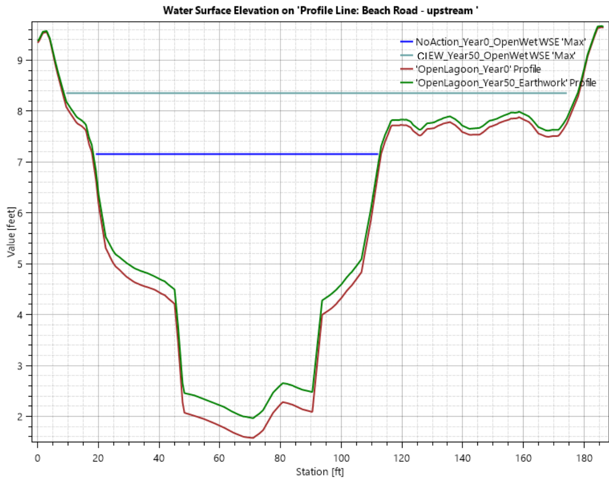
Figure 26: Cross section of terrain and maximum computed WSE immediately upstream of the Beach Road crossing for Simulation 2 (No Action, Year 0, Open Lagoon, Wet Season) and Simulation 46 (Crossing Improvements + Earthwork, Year 50, Open Lagoon, Wet Season).
