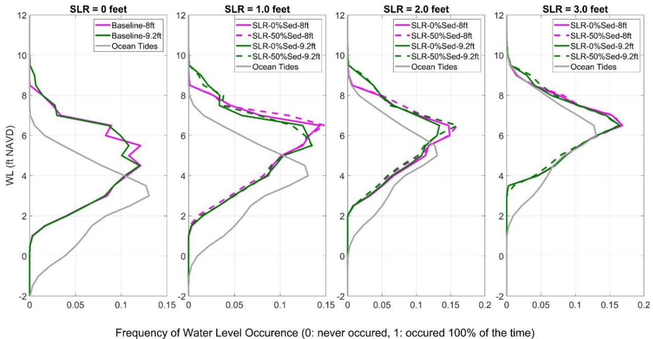
Figure 12 Frequency of modeled lagoon water levels for With and Without-Project conditions, lagoon sedimentation, and 0 to 3 feet of sea-level rise.
