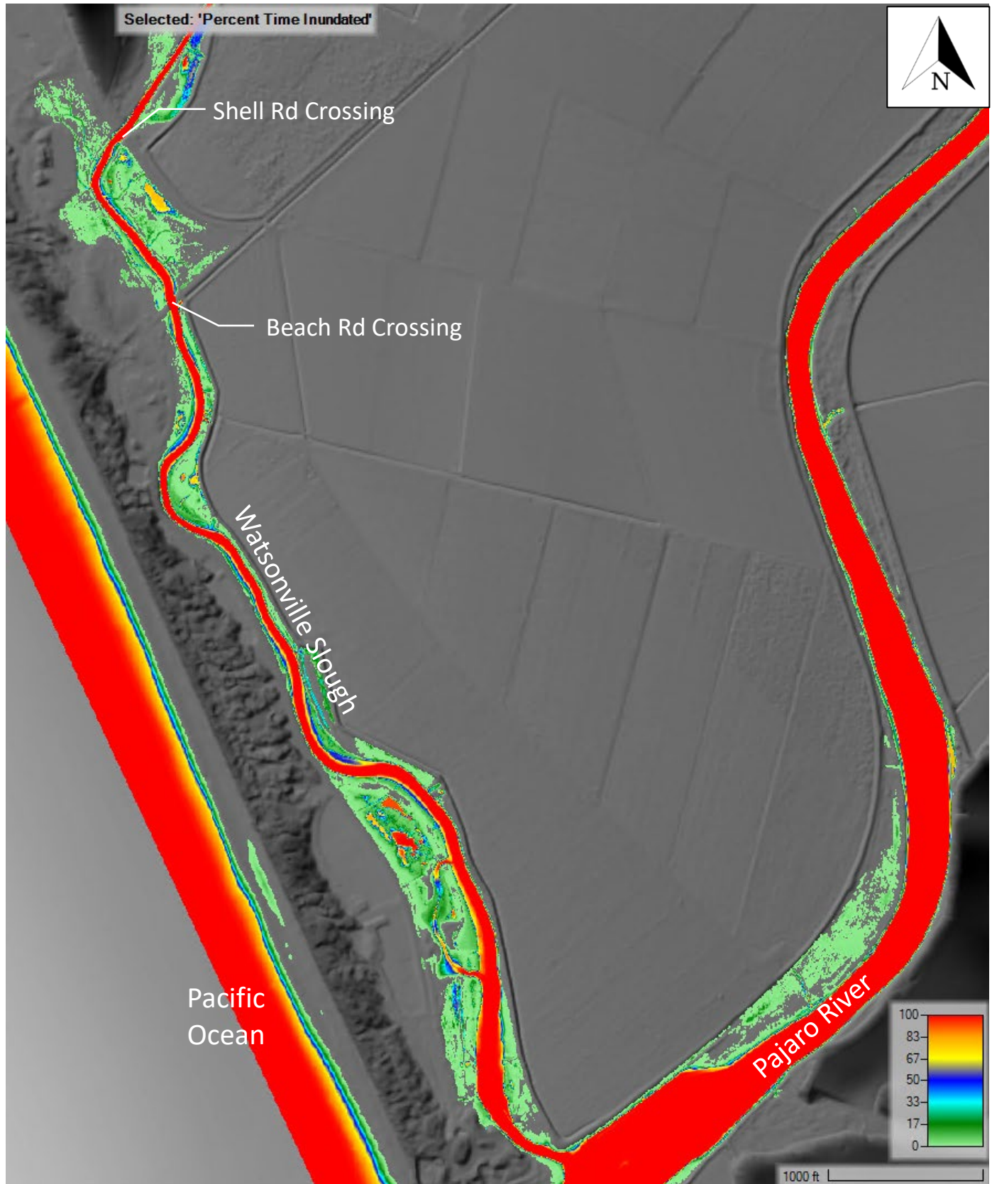
Figure 32: Percent time inundated – Crossing Improvements + Earthwork; Year 25; Open Lagoon, Wet Season
