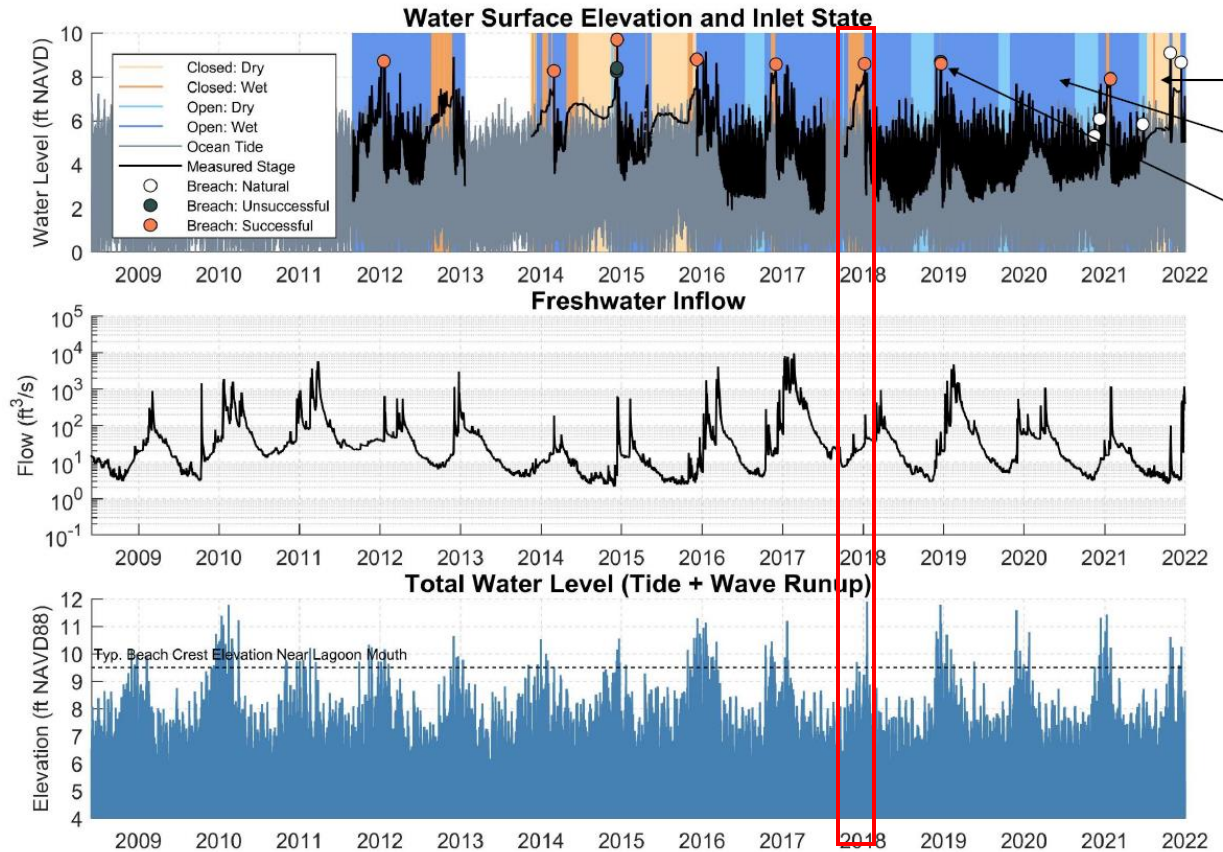
Figure 5: Historical record of water levels in Pajaro Lagoon, freshwater inflow into the lagoon, and total water level in Monterey Bay, with lagoon closure state and breach events indicated. The red box highlights the closure period that was selected for hydraulic modeling for the Watsonville CAP feasibility study. Figure adapted from preliminary results provided by ESA.
