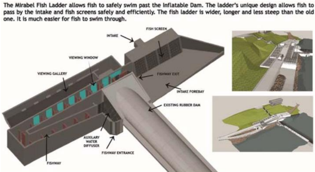
Figure 3-4 Mirabel Fish Ladder and Diversion Facility
