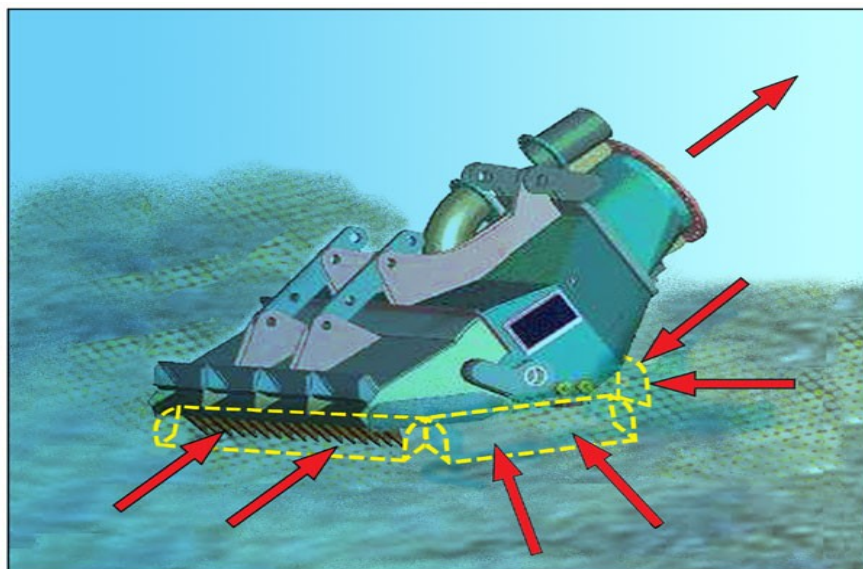
Figure 2-2 Hopper Drag Head Schematic
