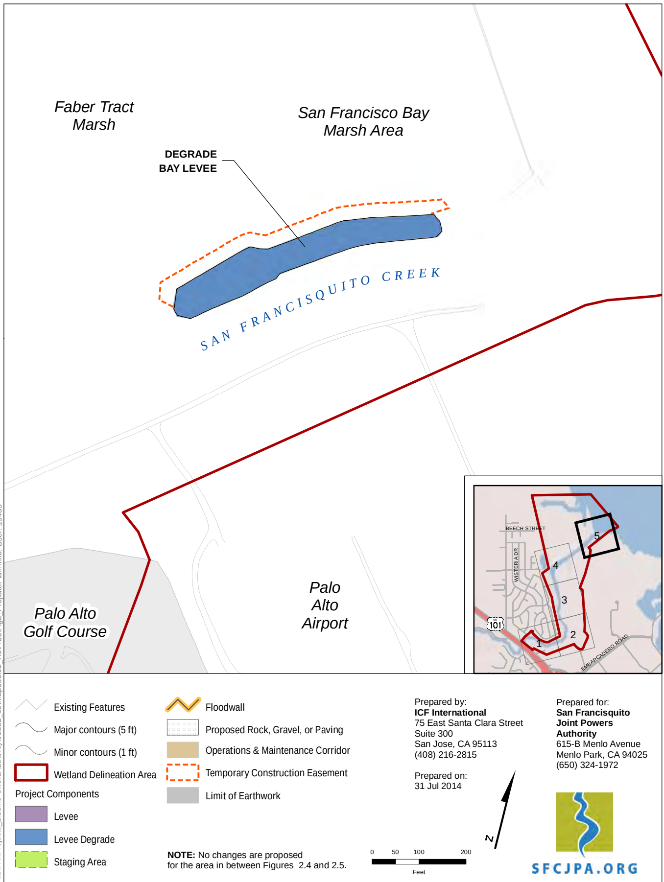
Figure 2. 5 Project Site Plan San Francisquito Creek Flood Reduction, Ecosystem Restoration & Recreation Project - S.F. Bay-Highway 101 July 31, 2014
