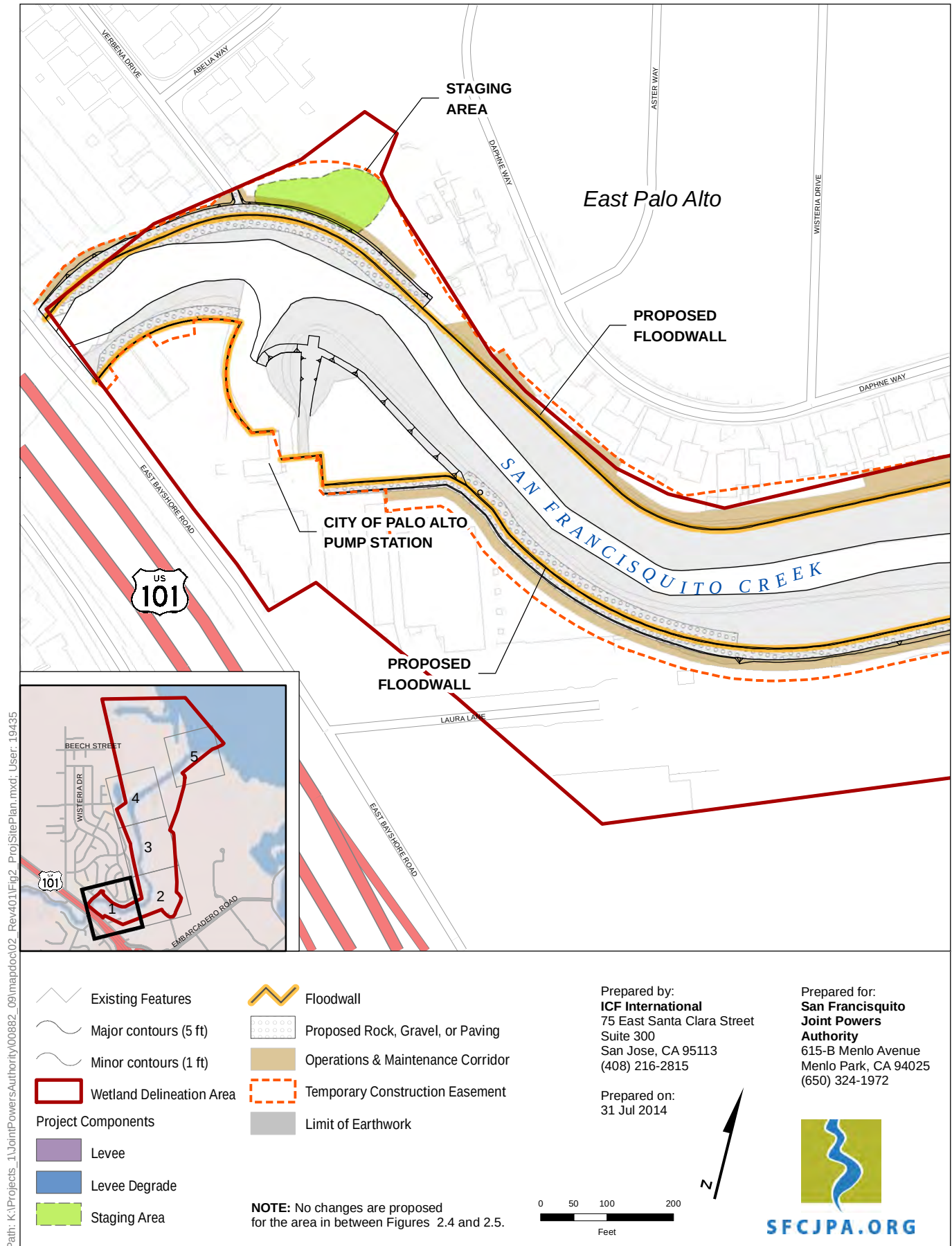
Figure 2. 1 Project Site Plan San Francisquito Creek Flood Reduction, Ecosystem Restoration & Recreation Project - S.F. Bay-Highway 101 July 31, 2014
