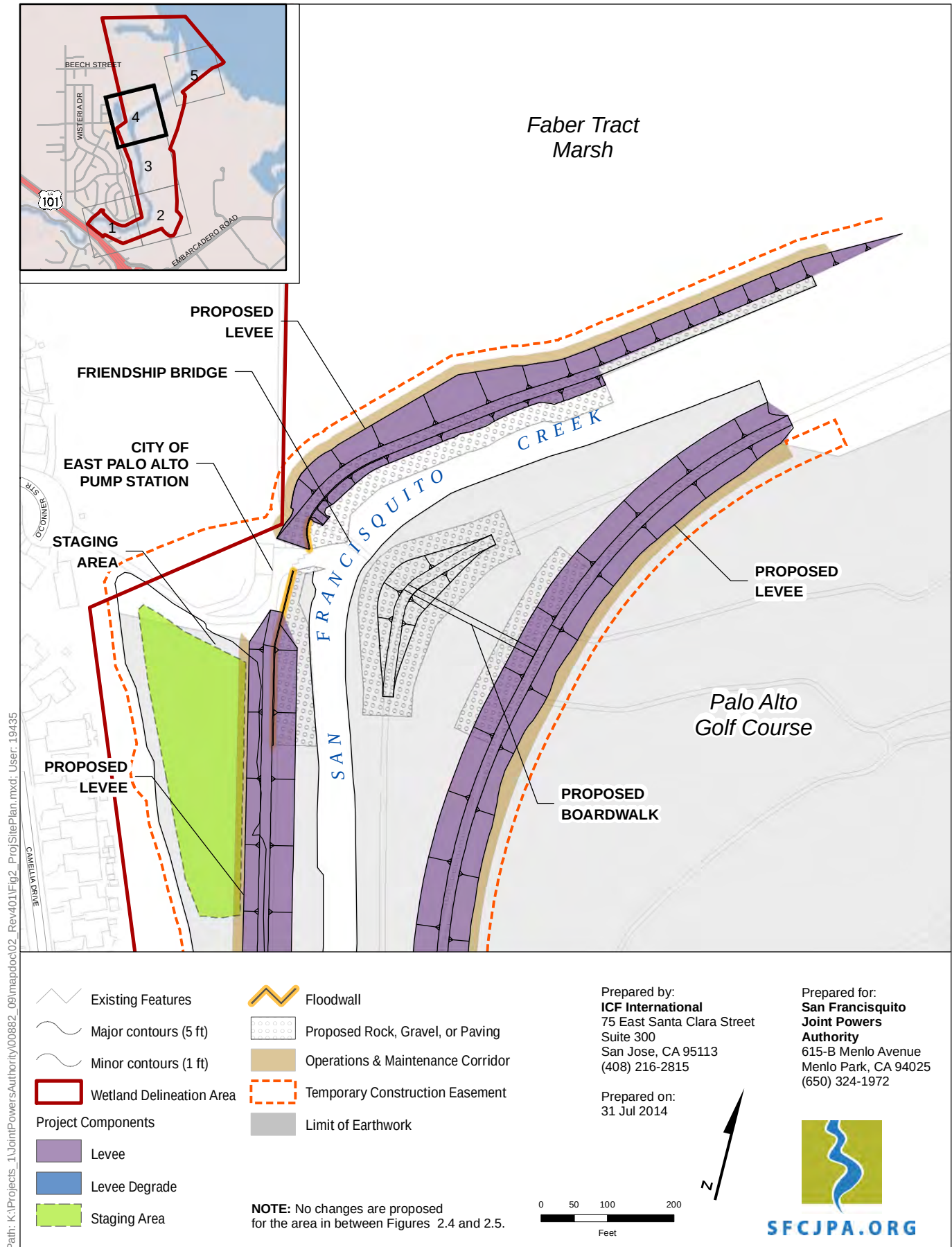
Figure 2. 4 Project Site Plan San Francisquito Creek Flood Reduction, Ecosystem Restoration & Recreation Project - S.F. Bay-Highway 101 July 31, 2014
