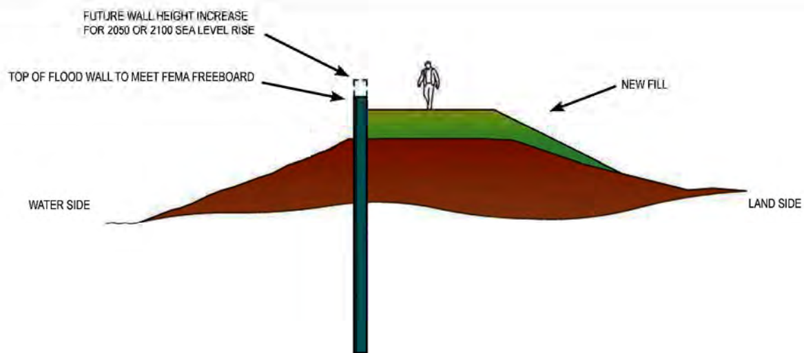
Figure 4. Typical Sheet Pile Flood Wall Cross Section Levee Protection Planning and Improvement Project CIP 301-657 City of Foster City, San Mateo County, California
