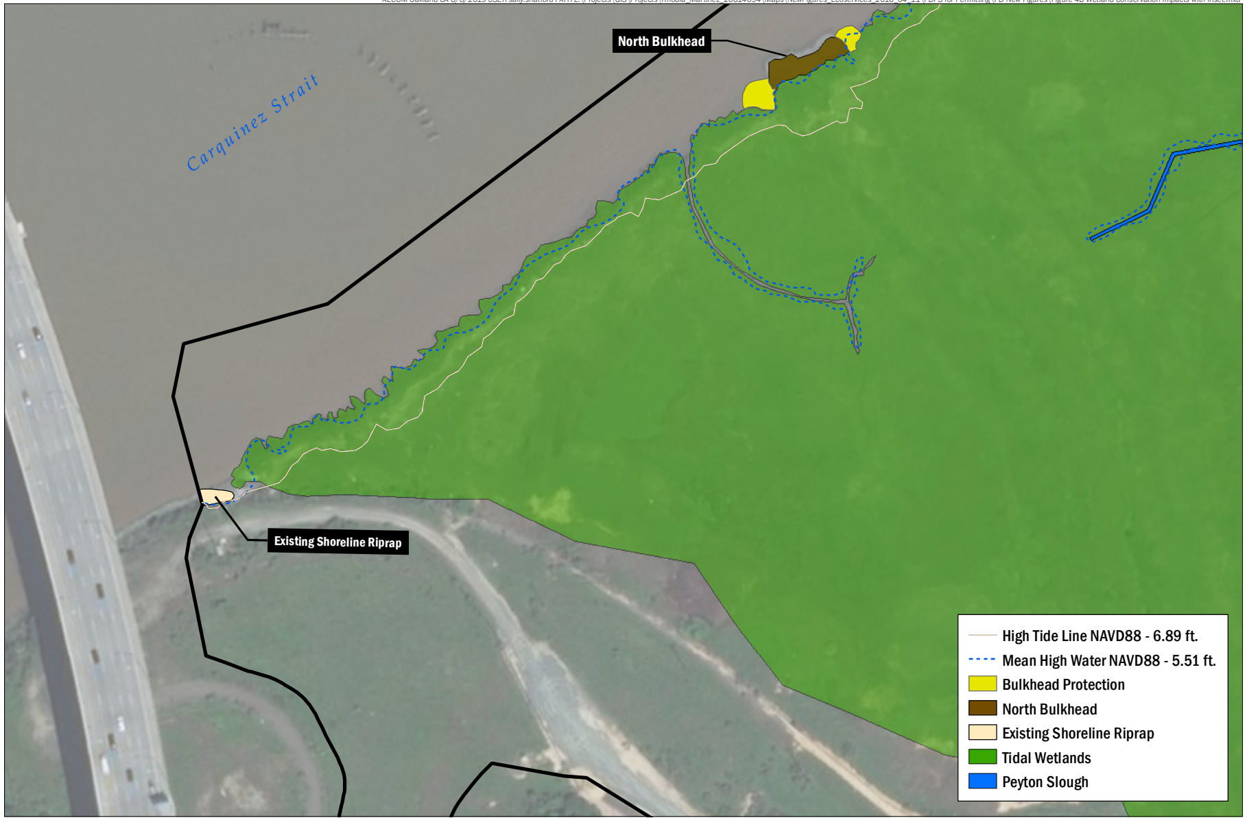
FIGURE 4B North Bulkhed Repair and Protection
