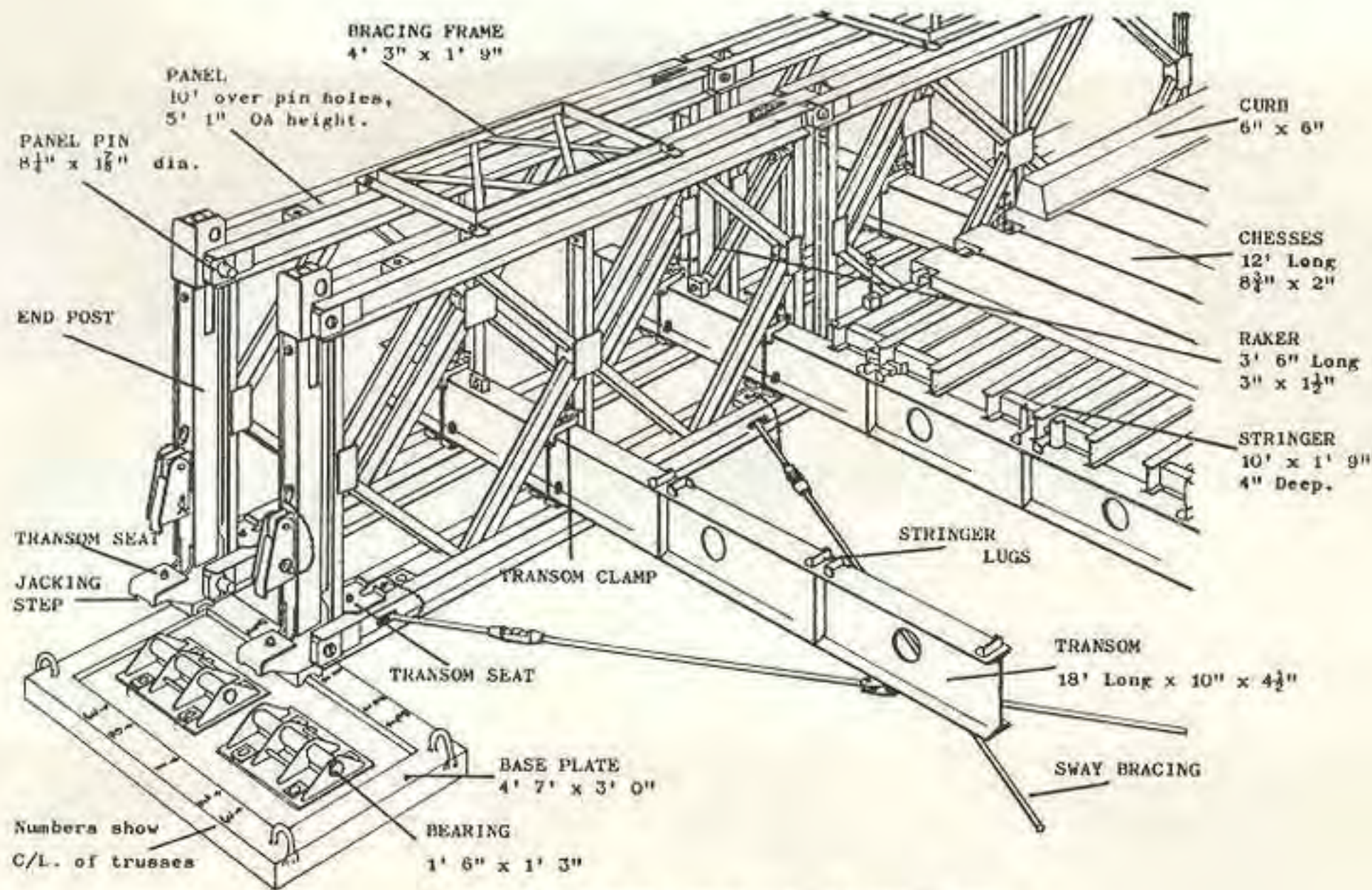
DIAGRAM OF DOUBLE TRUSS - SINGLE STOREY (DS)
