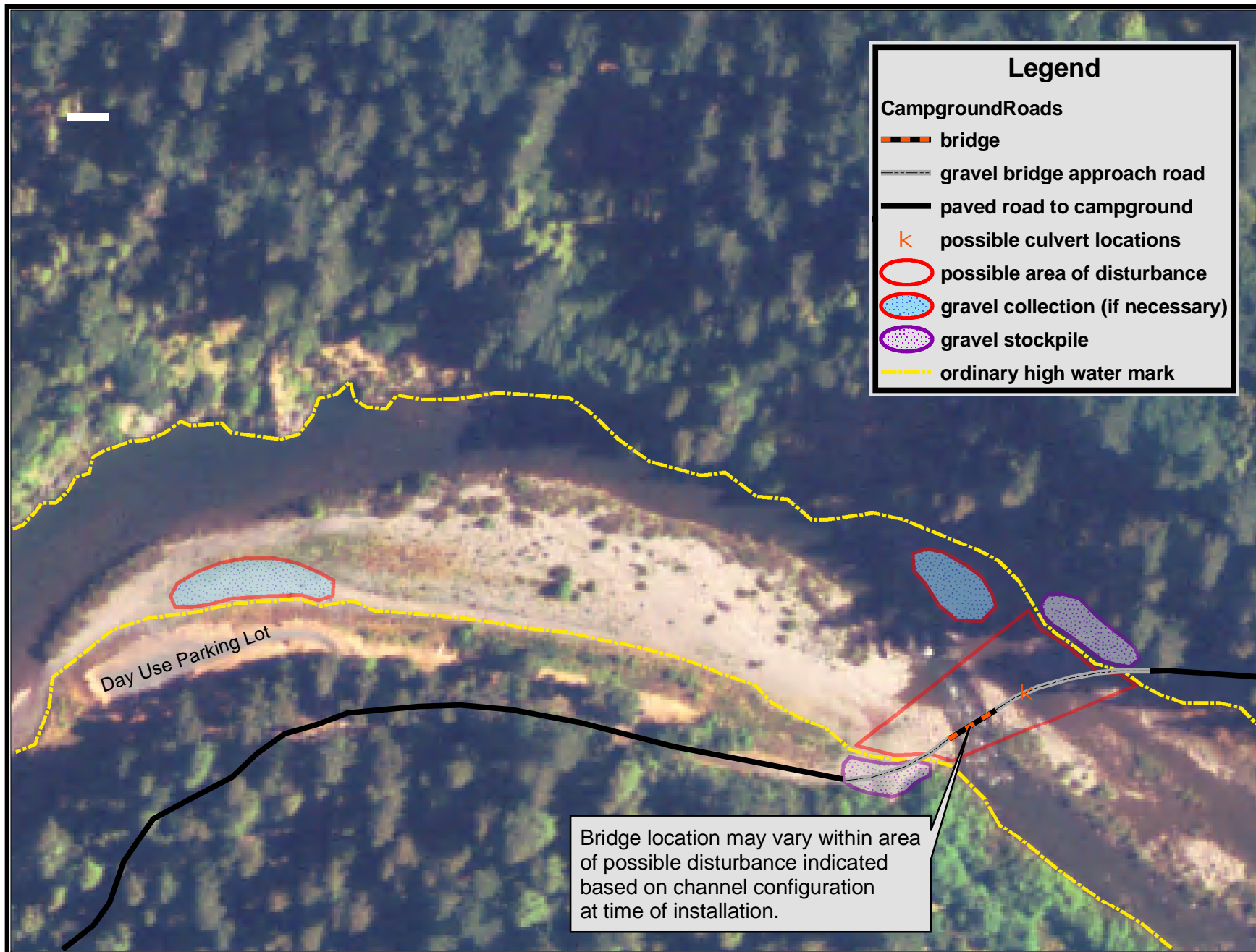
California Department of Parks and Recreation Bailey Bridges Project Site Plan Standish-Hickey State Recreation Area
