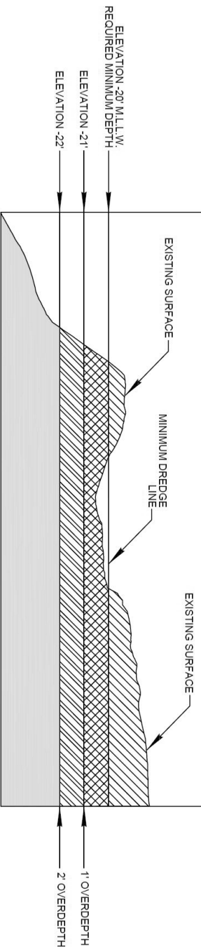
TYPICAL DREDGING SECTION B-B BARGE PIER (NOT TO SCALE)
