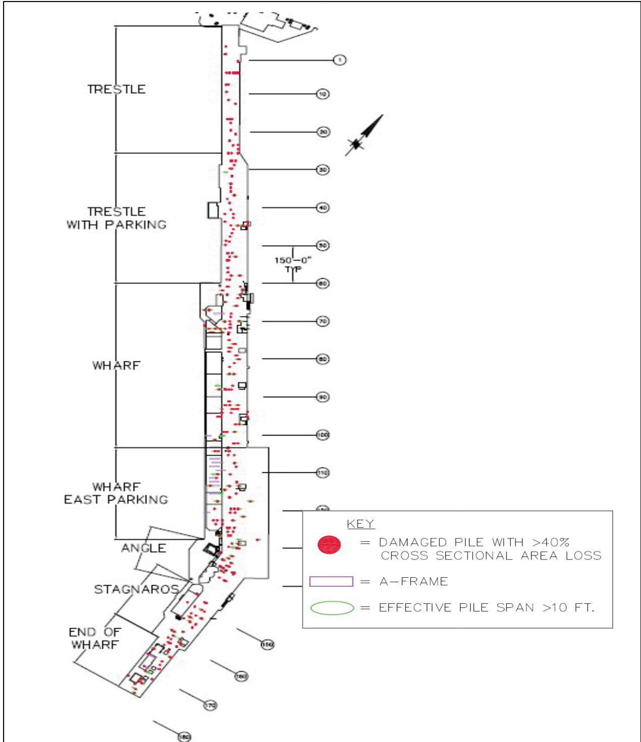
Figure 2: Piling Survey Summary (2014)
