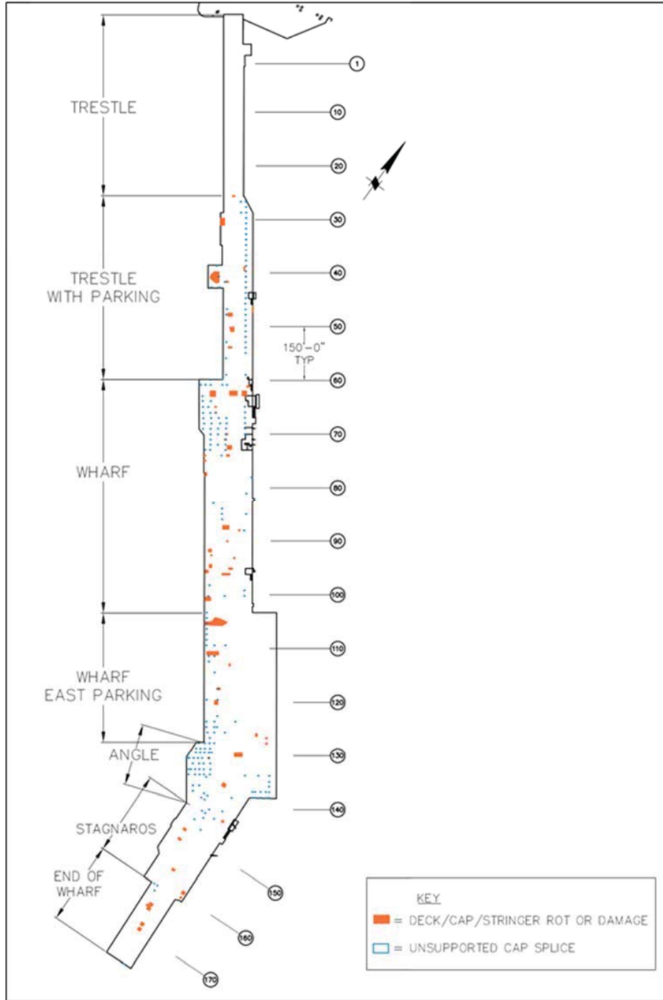
Figure 4: Substructure Damage Plan
