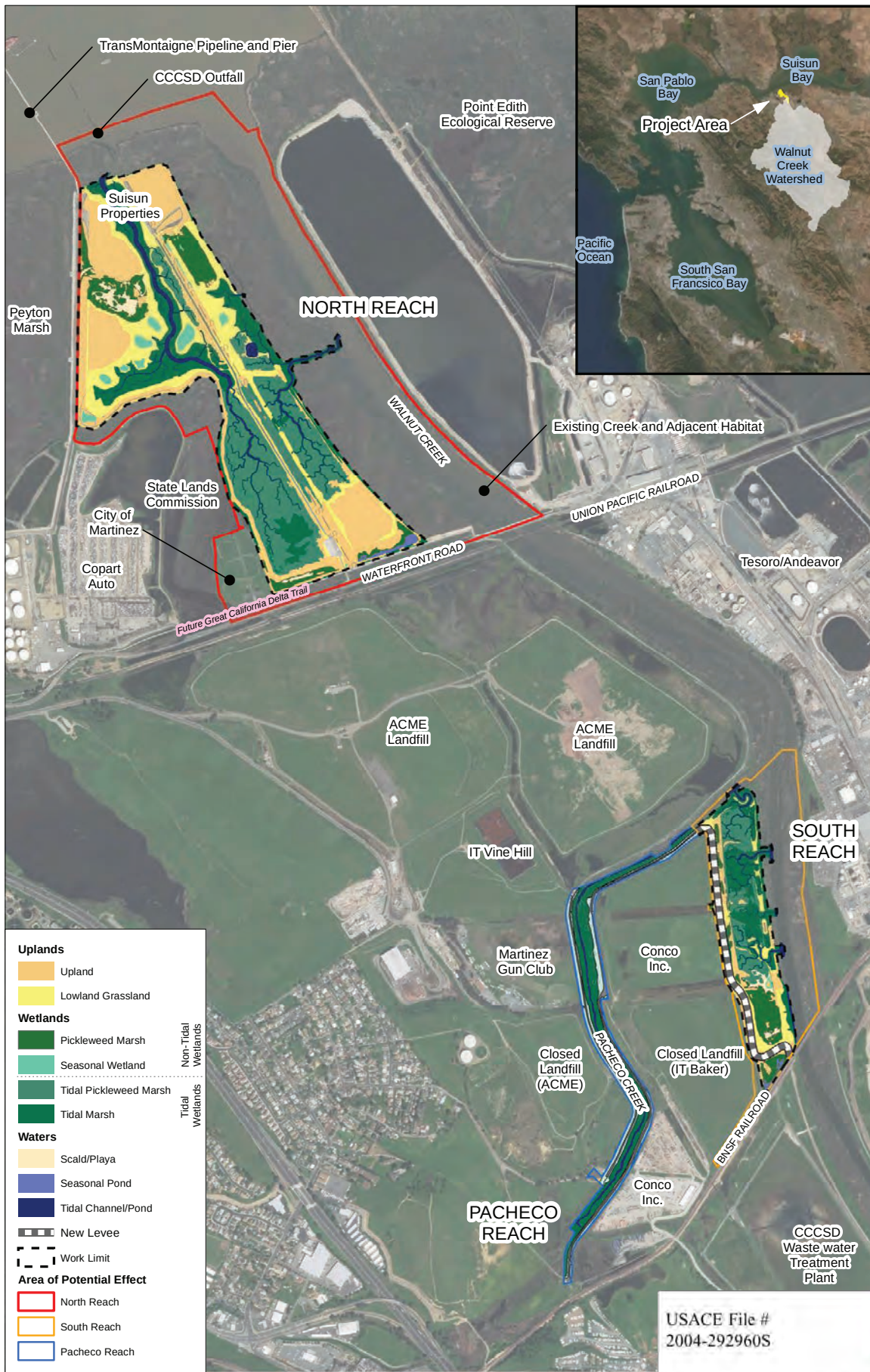
Lower Walnut Creek Restoration Project Figure 3: Project Restoration Plan
