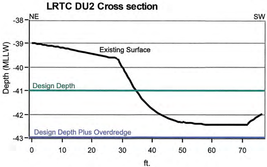
Figure 5. Typical Cross Section
