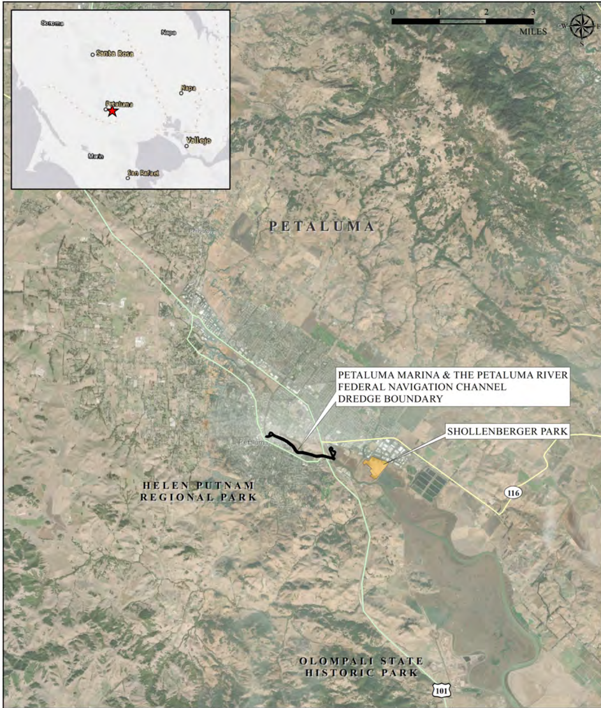
FIGURE 2. VICINITY MAP: PETALUMA MARINA AND THE PETALUMA RIVER FEDERAL NAVIGATION CHANNEL
