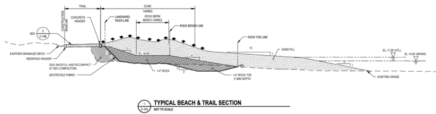
Figure 3 Proposed Living shoreline design
