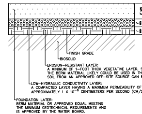
BIOSOLID CAP DETAIL
